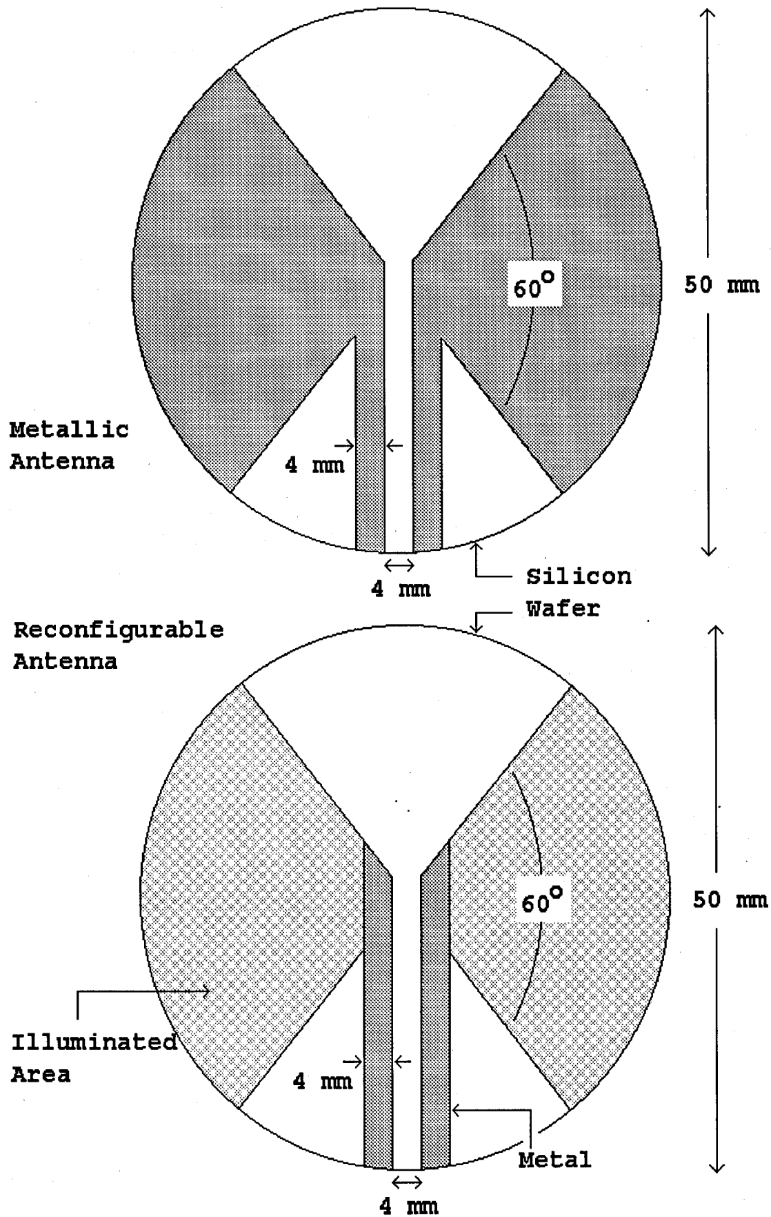
Figure 2 Triangular Antennas
