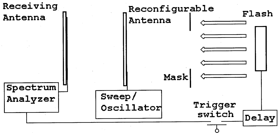
Figure 1 Experimental Set-up
