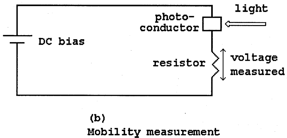
Figure 13 Semiconductor Characterization
