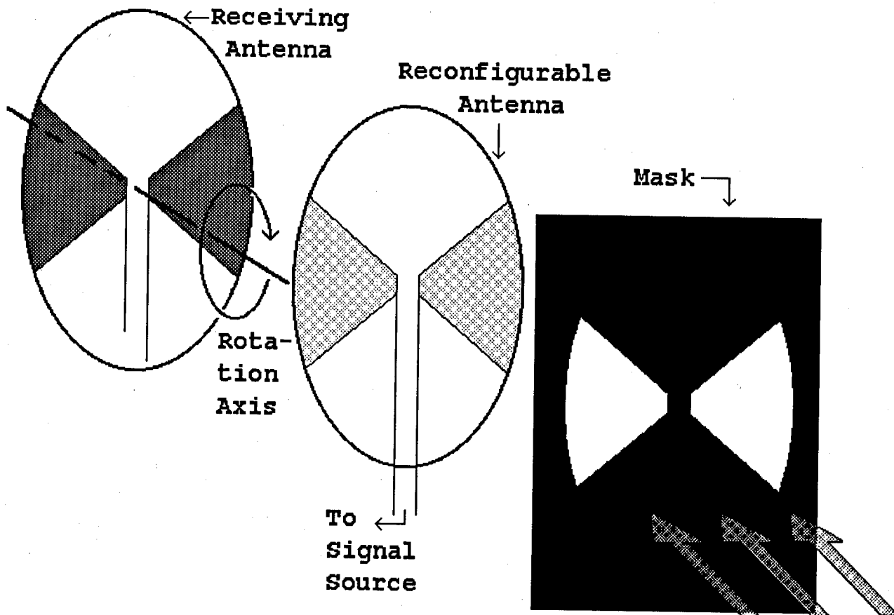
Figure 10 Polarization Check
