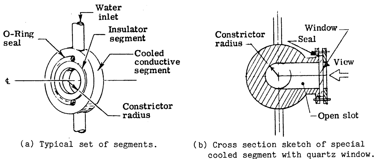
Figure 11.- Arc channel or "constrictor" segments.
