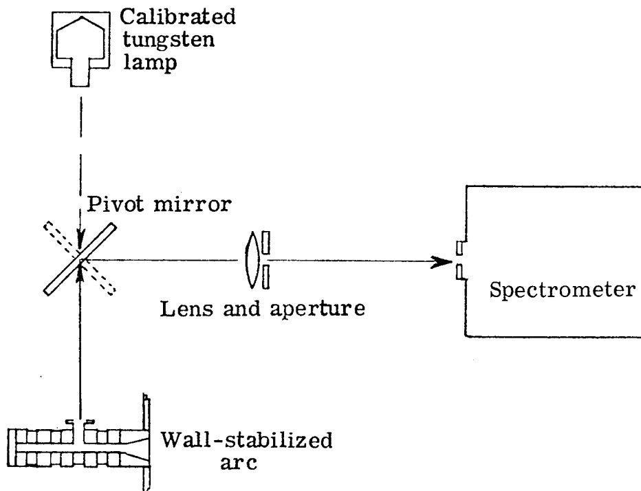
Figure 10.- Diagnostic optical system.
