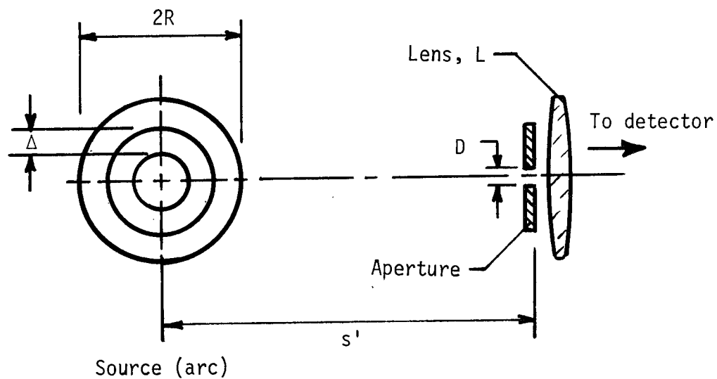
Figure 15.- Model of arc cross section with lens and aperture stop.
