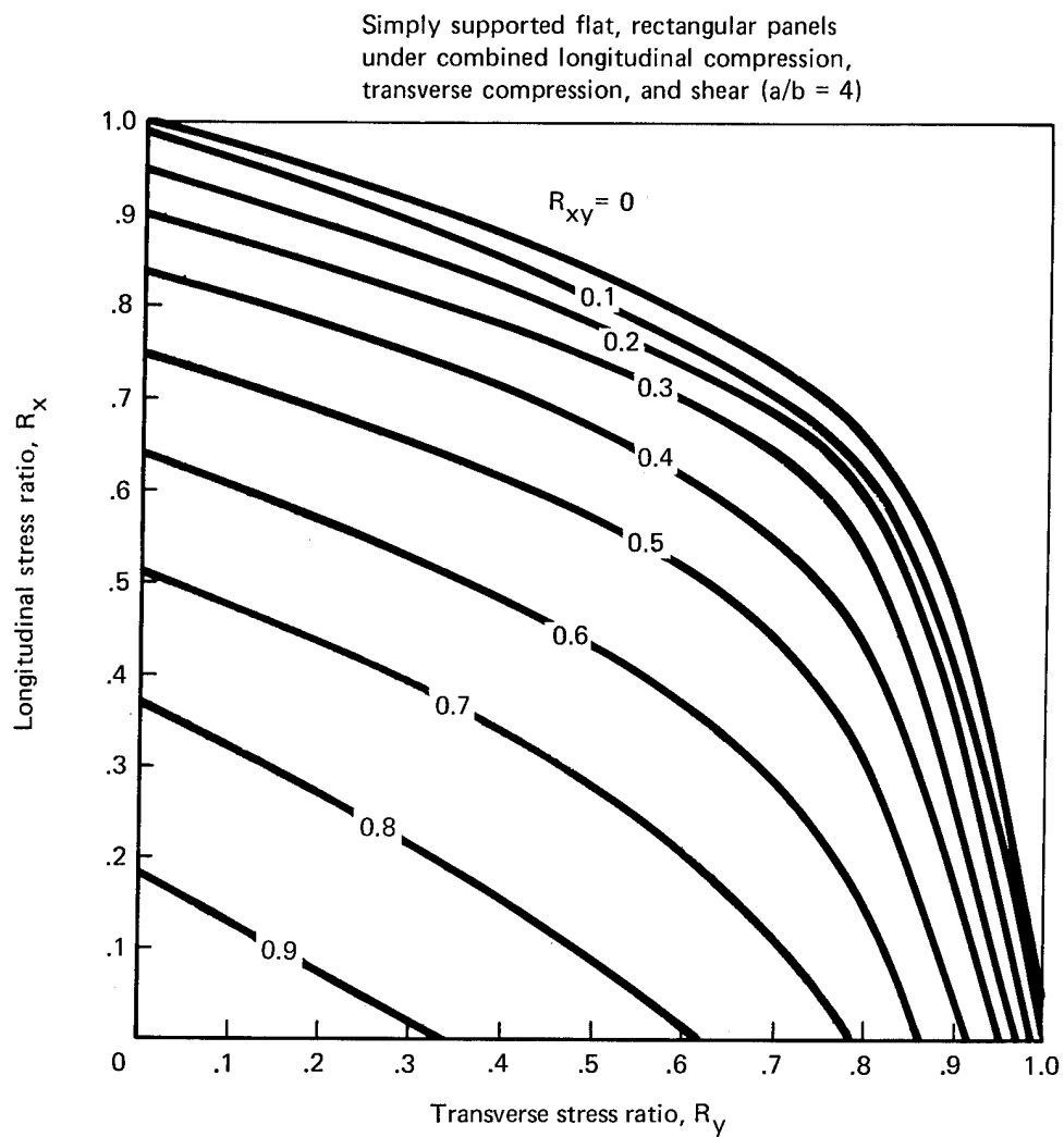
Figure 6-4.—Initial Buckling of Flat Rectangular Panels
