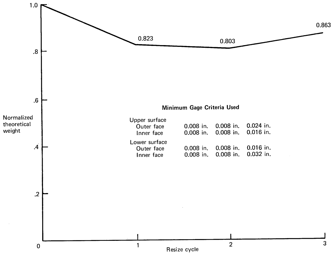
Figure 7-7.—Theoretical Wing Weight, Wing Box Primary Structure, ATLAS Resizing
