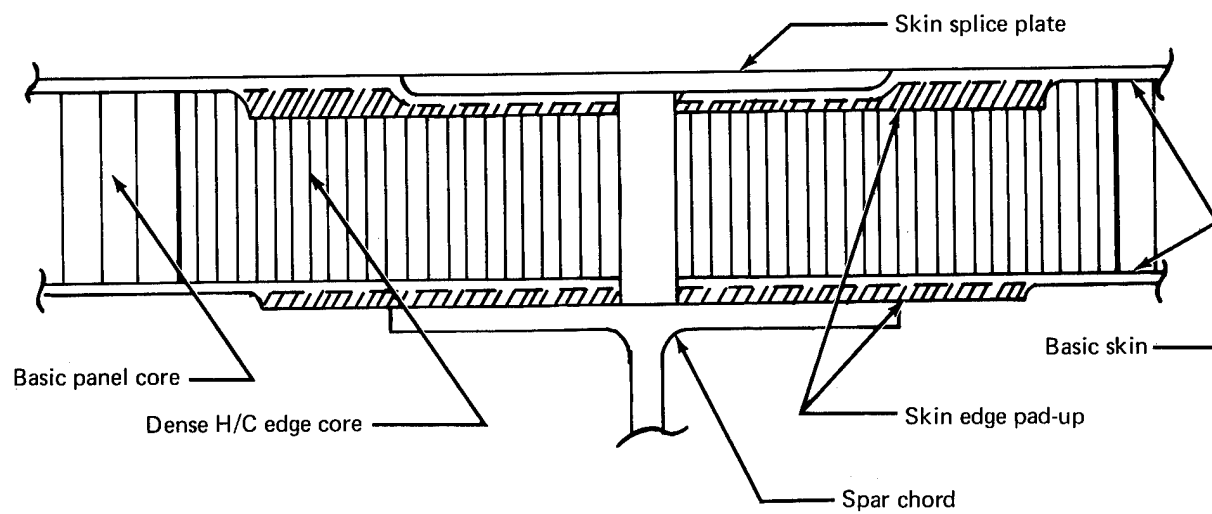
Figure 5-2.—Skin Spanwise Edge Design
