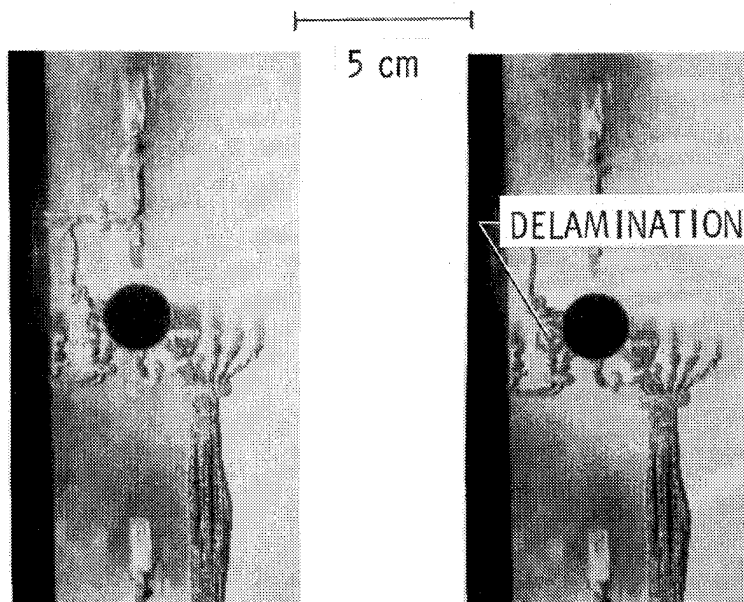
(b) 95.4 percent of ultimate load. Delamination to left of hole.
