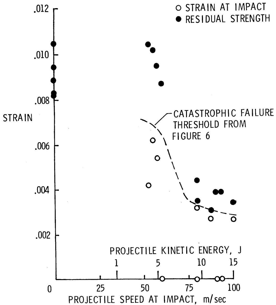
Figure 8. - Effect of projectile speed on residual strength.
