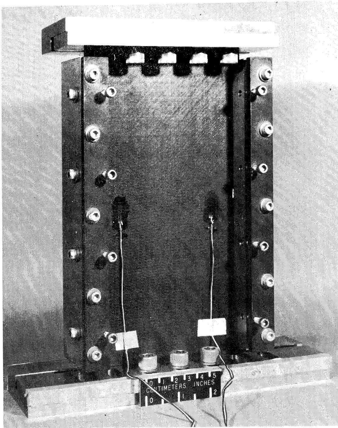
Figure 1. - 48-ply graphite-epoxy specimen in test fixture.
