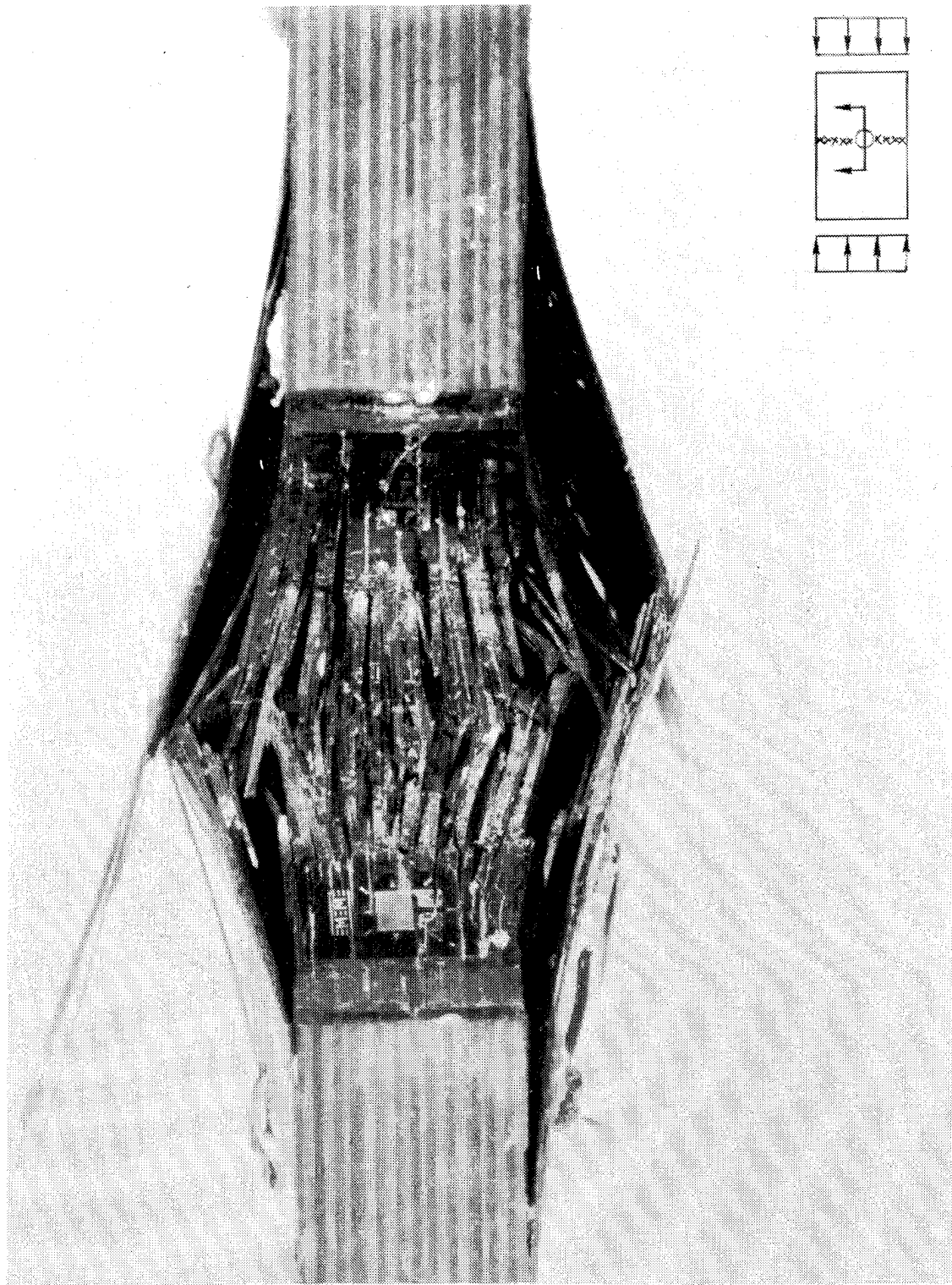
Figure 13. - Cross section of a failed specimen with a 1.91 cm diameter hole.
