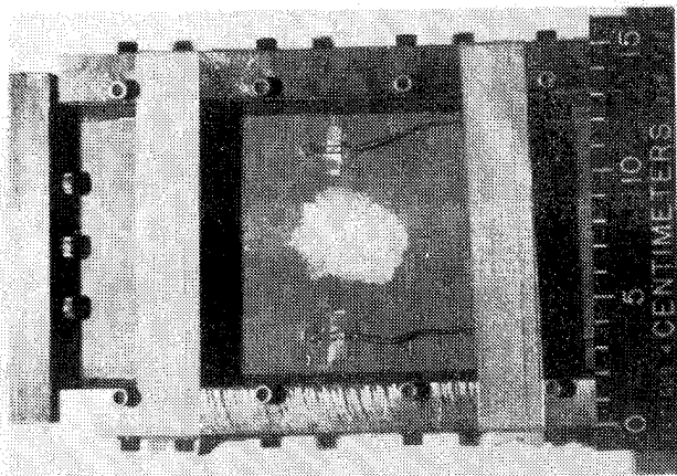
(a) Specimen with initial impact damage.
