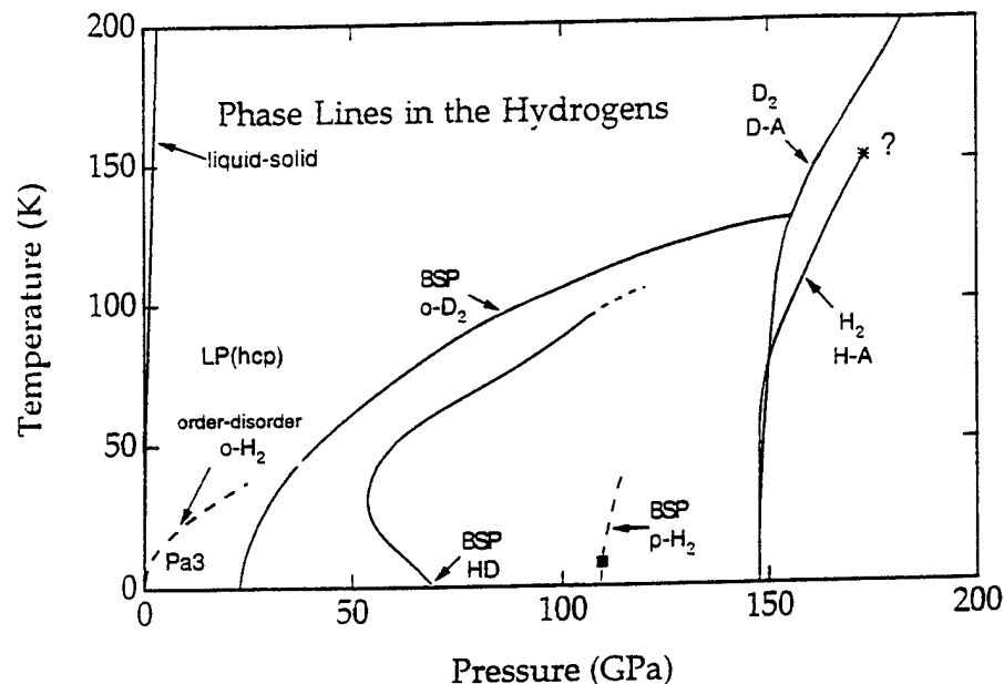
Figure 1 Partial Phase Diagram of the Hydrogens
