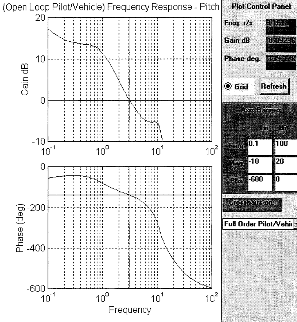
Figure 2-32. Bode plot of open loop MOCM pilot/vehicle.
