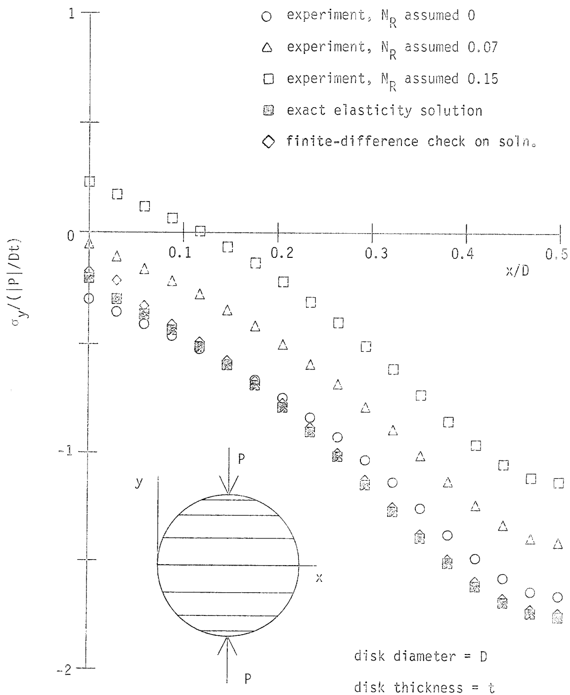
Fig. 99 Comparison of \sigma_y stresses along diameter perpendicular to load, fibers perpendicular to load.
