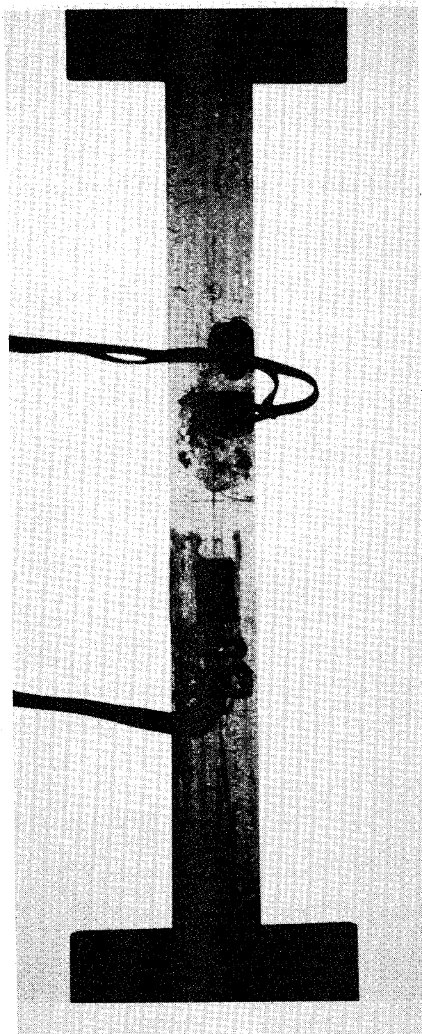
Fig. 16 The 0° tensile specimen in light field with fringe order 1.
