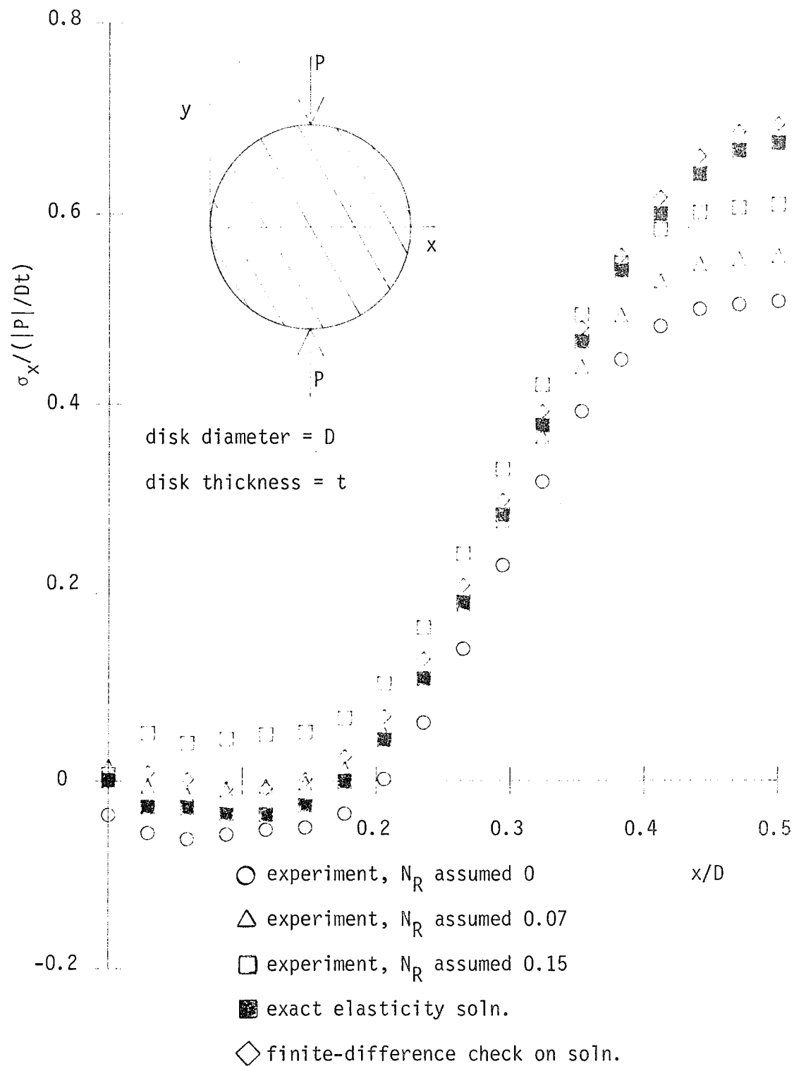
Fig. 88 Comparison of \sigma_x stresses along diameter perpendicular to load, fibers 30° relative to load.
