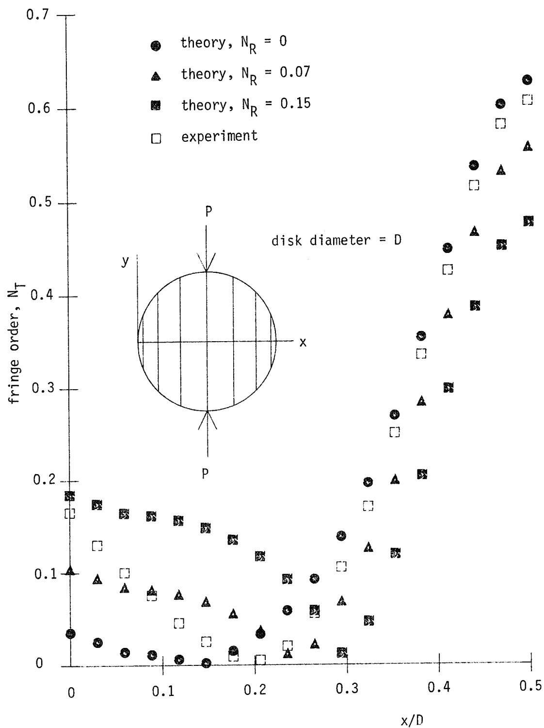
Fig. 60 Comparison between predicted and observed isochromatic fringe order along diameter perpendicular to load, fibers aligned with load.
