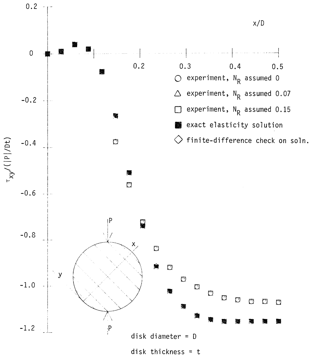
Fig. 98 Comparison of \tau_{xy} stresses along diameter perpendicular to fibers, fibers 45^\circ relative to load.
