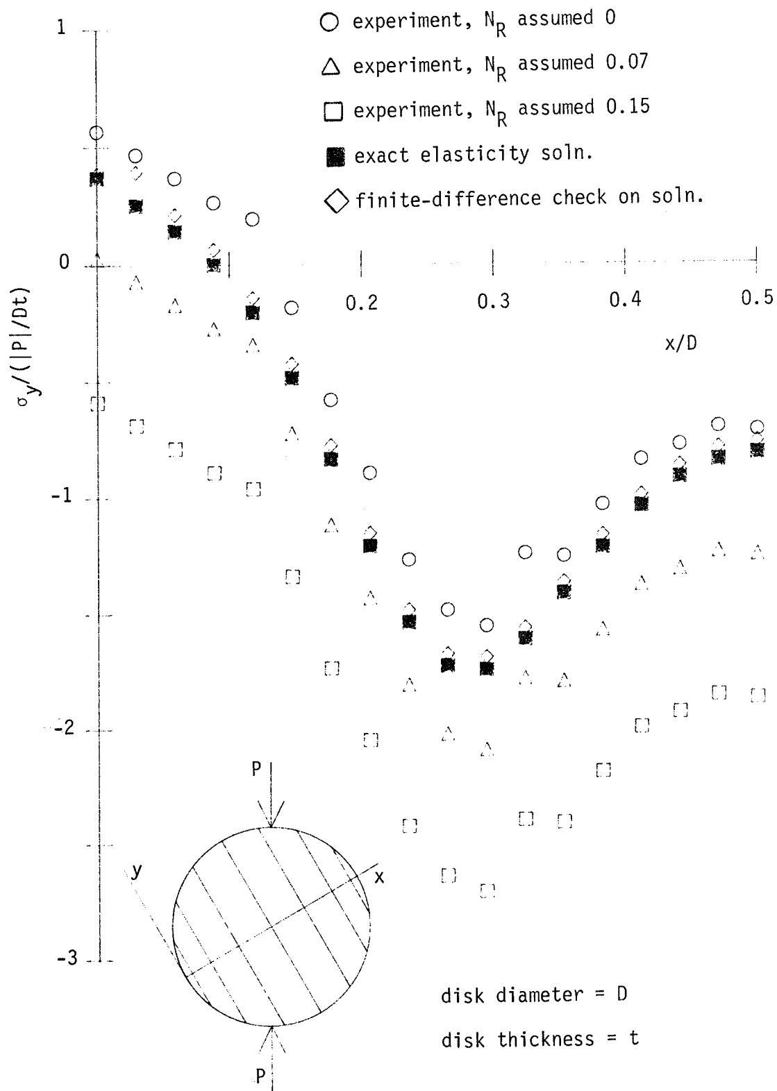
Fig. 90 Comparison of \sigma_y stresses along diameter perpendicular to fibers, fibers 30^\circ relative to load.
