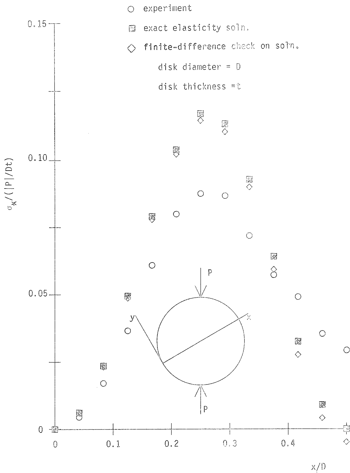
Fig. 109 Comparison of \sigma_x stresses along 30^\circ diameter, isotropic disk.
