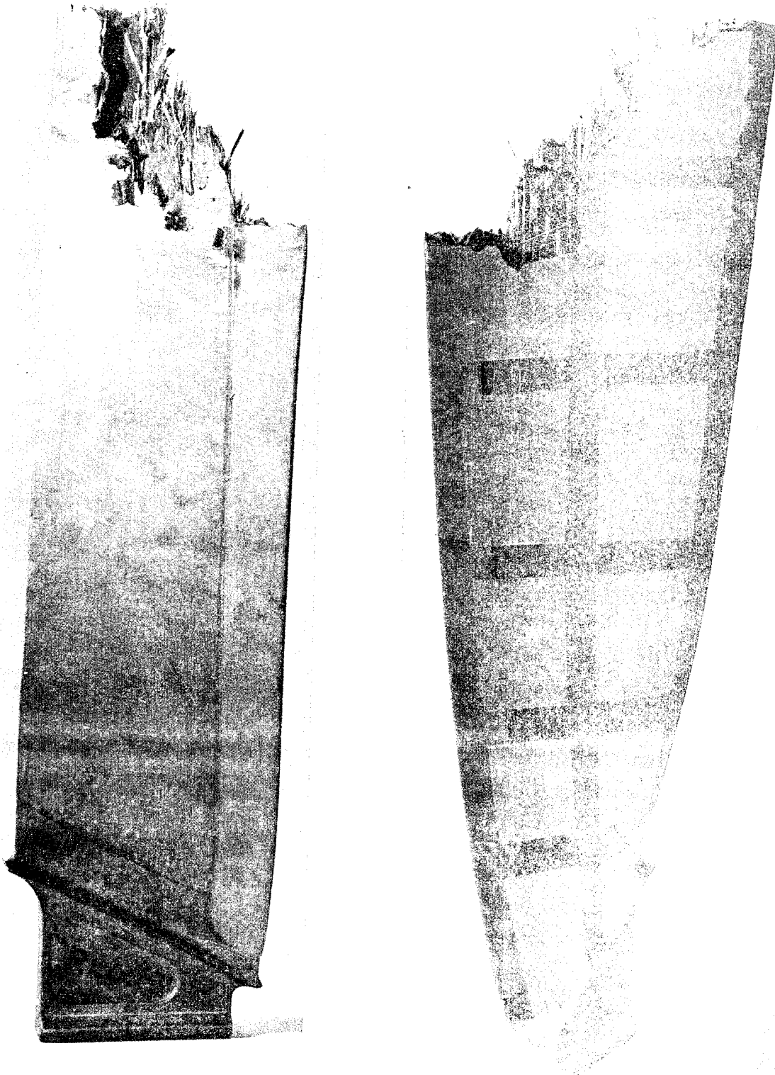
Figure 52. TiCore Superhybrid Blade (RL004) Shown After Whirligig Impact Testing of 1.5-pound Bird.
