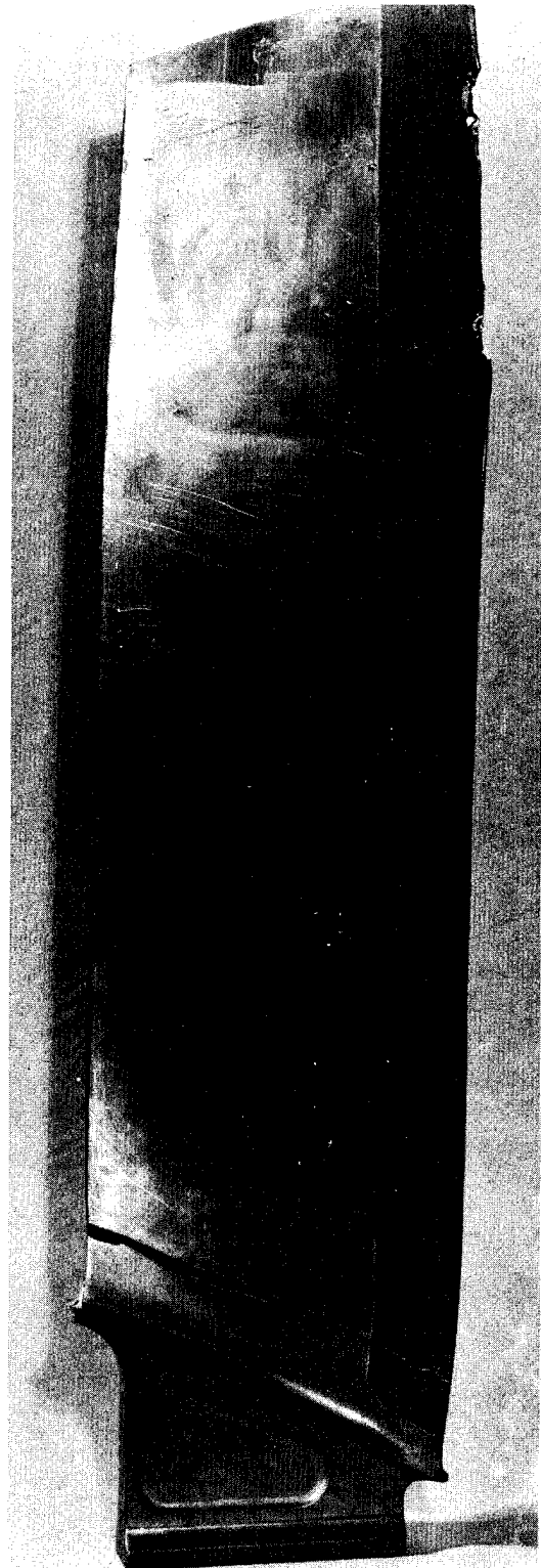
Figure 51. TiCore Superhybrid Blade (RL006) Without Leading Edge Protection, Shown After Impact Testing of 3.0-ounce Starling.
