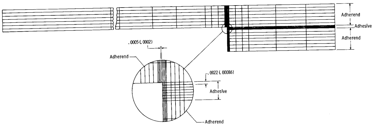
(b) STAGS (ref. 27) finite-difference mesh.
