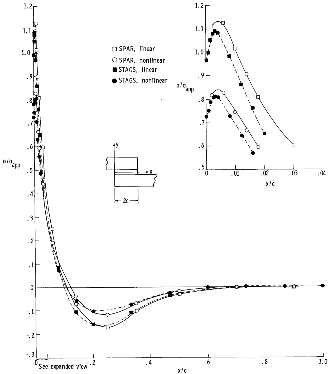
Figure 11.- Comparison of peel stress distributions along center line of adhesive given by finite-difference and finite-element analyses. T = 175 \text{ kN/m} (1000 lbf/in.); \sigma_{app} = T/t .
