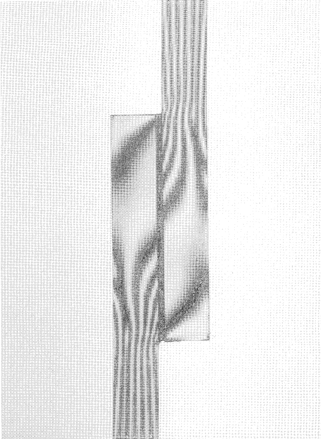
(c) Flexible adhesive model.
