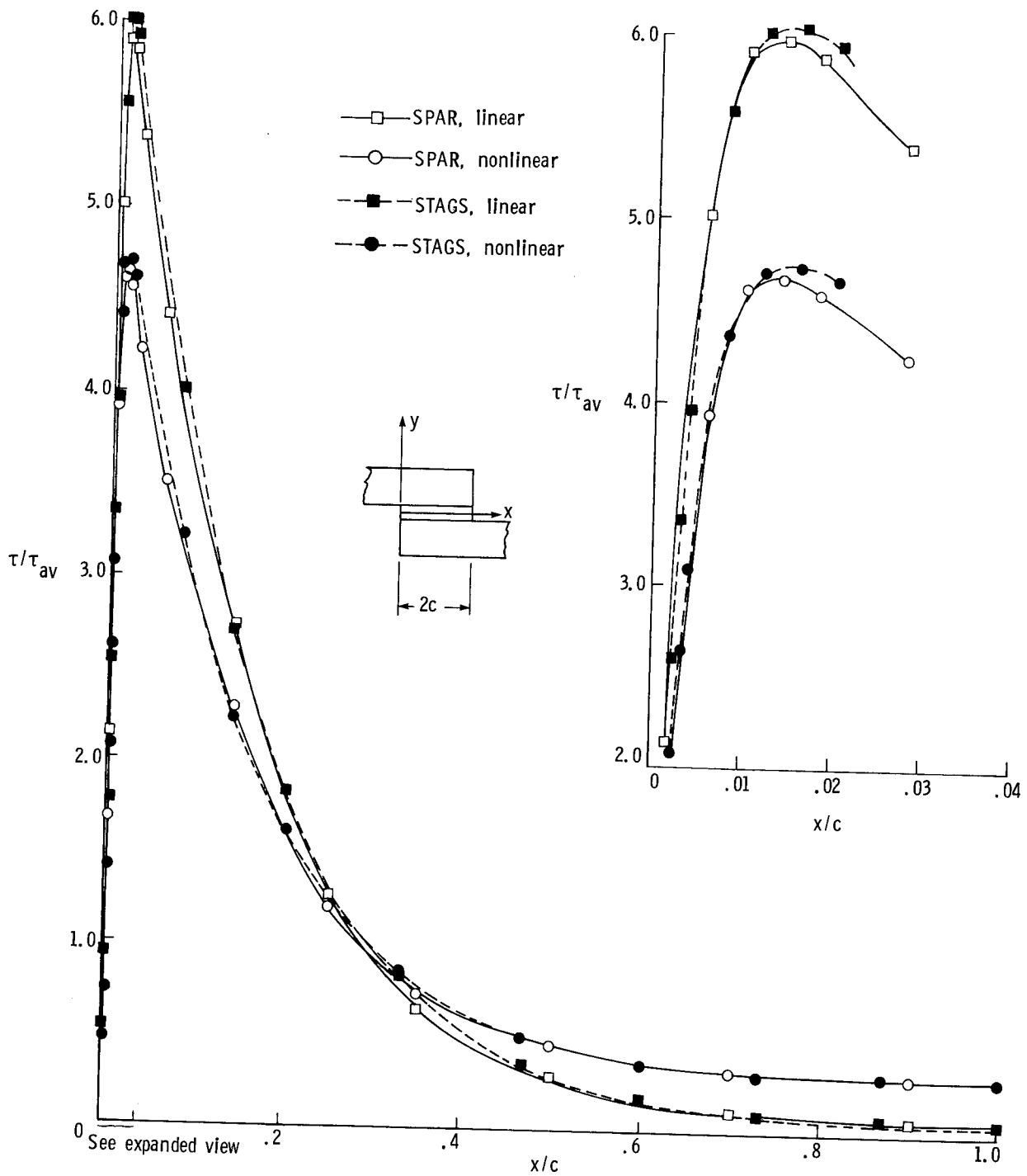
Figure 10.- Comparison of shear stress distributions along center line of adhesive given by finite-difference and finite-element analyses. T = 175 \text{ kN/m} (1000 lbf/in.); \tau_{av} = T/2c .
