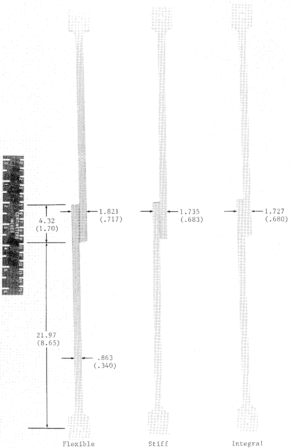
Figure 27.- Photograph of photoelastic models. Dimensions are given in centimeters (inches). L-79-1781.1
