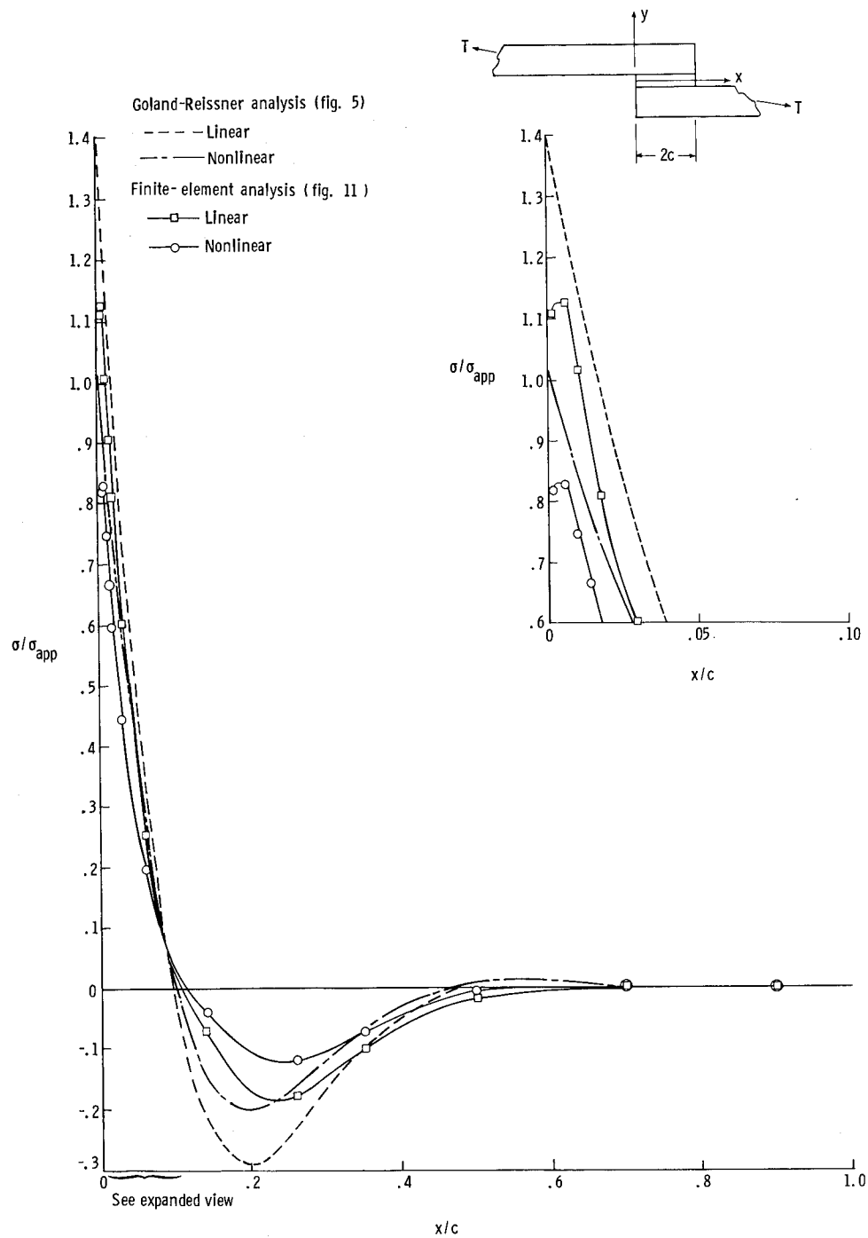
Figure 13.- Comparison of peel stress distributions along center line of adhesive given by Goland-Reissner analysis and finite-element analysis. T = 175 \text{ kN/m} (1000 lbf/in.); \sigma_{app} = T/t .
