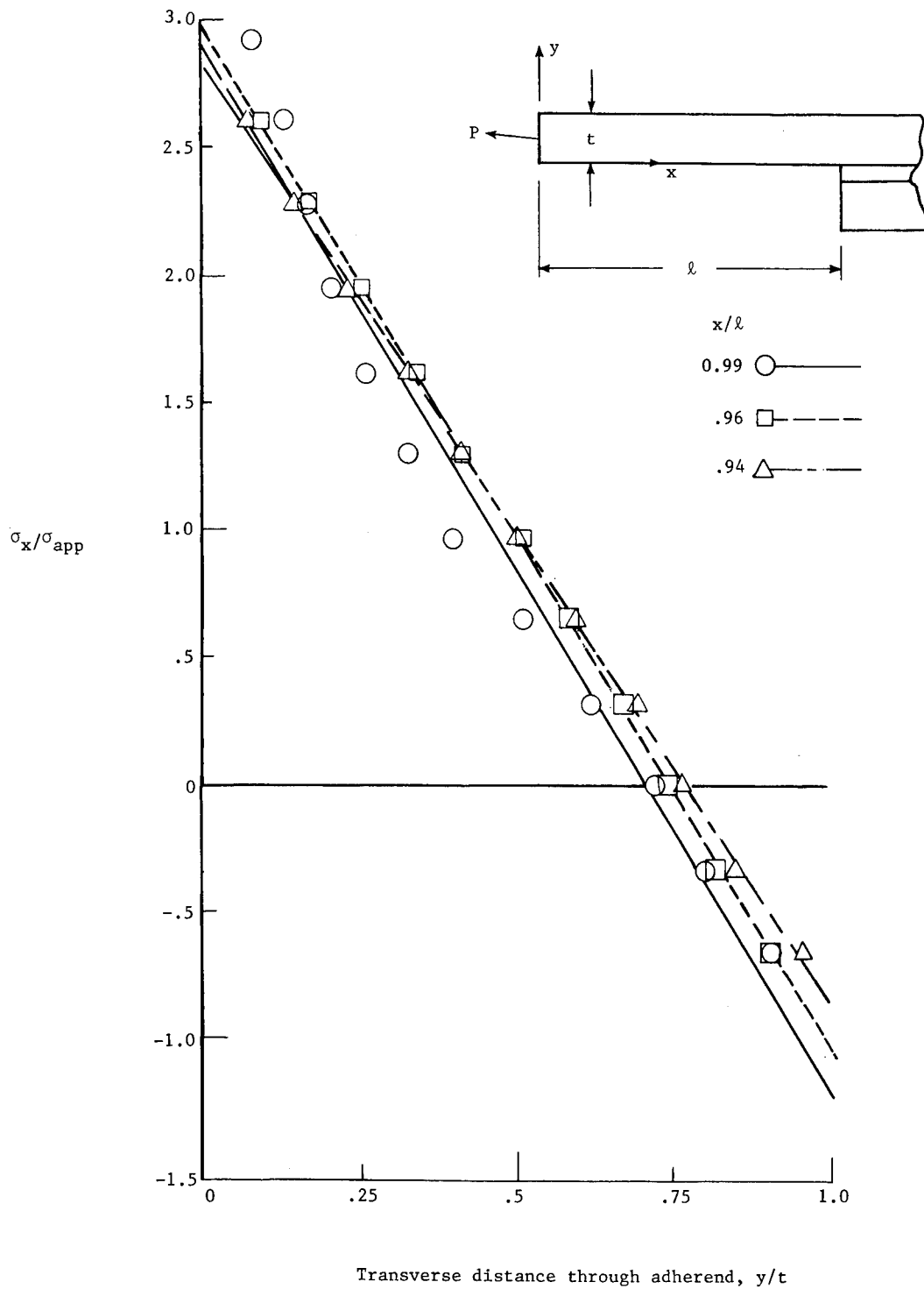
Figure 29.- Photoelastic measurement of adherend stress distribution near overlap. Stiff adhesive model; \sigma_{app} = P/a ; P = 133 \text{ N (30 lbf)} ; a = 0.32 \text{ cm}^2 (0.05 \text{ in}^2) ; l = 22.0 \text{ cm (8.65 in.)} ; c = 4.32 \text{ cm (1.70 in.)} ; t = 0.86 \text{ cm (0.34 in.)} .
