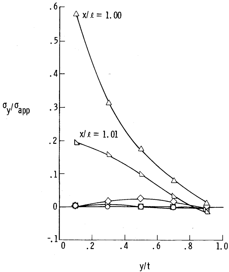
Figure 20.- Adherend transverse stress distributions at various locations. T = 175 \text{ kN/m (1000 lbF/in.)} ; \sigma_{app} = T/t .
