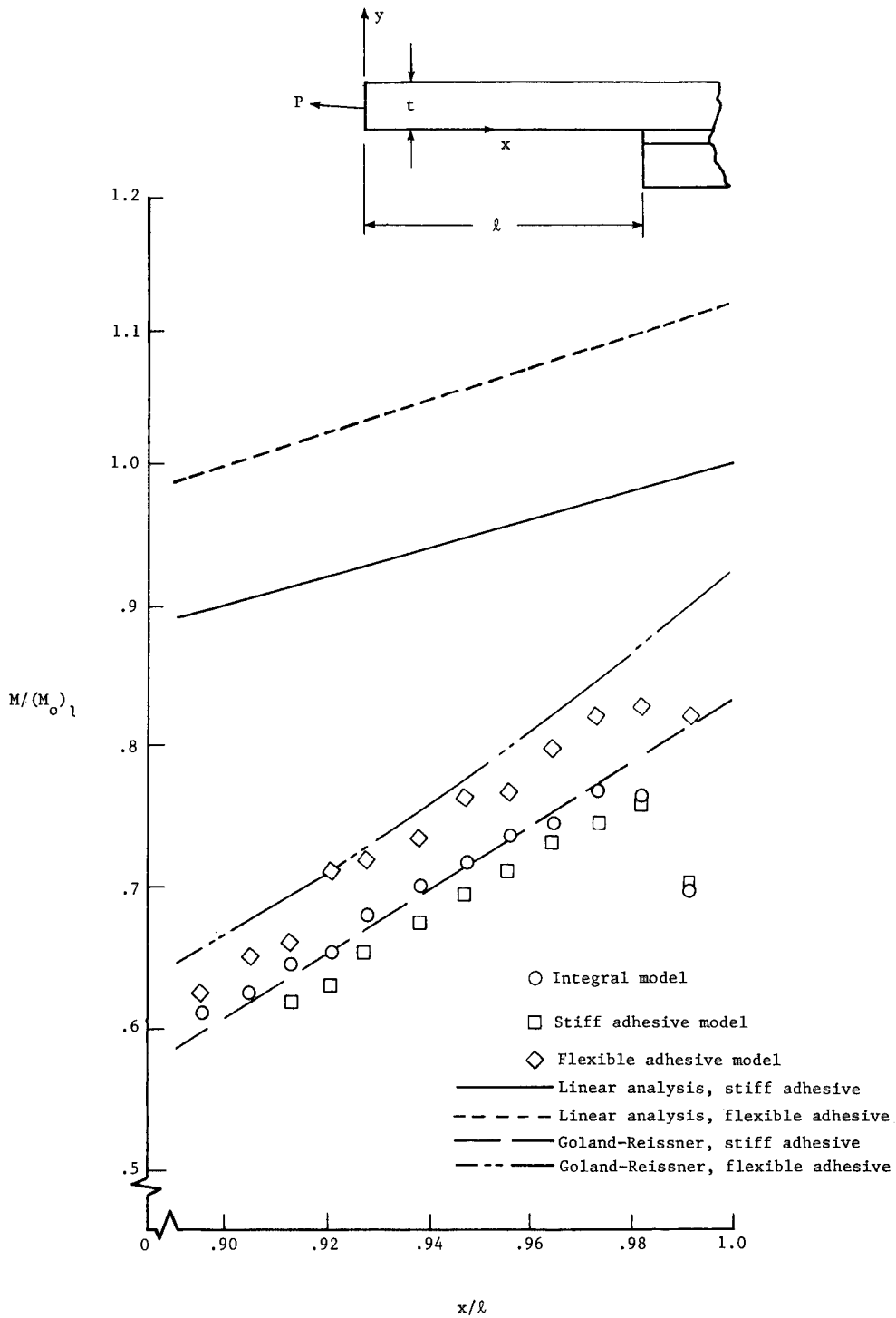
Figure 30.- Moment distribution along adherend near overlap. T = 133 \text{ N (30 lbf)} .
