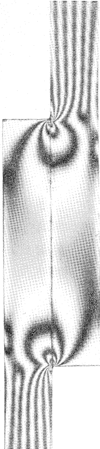
(b) Stiff adhesive model.
