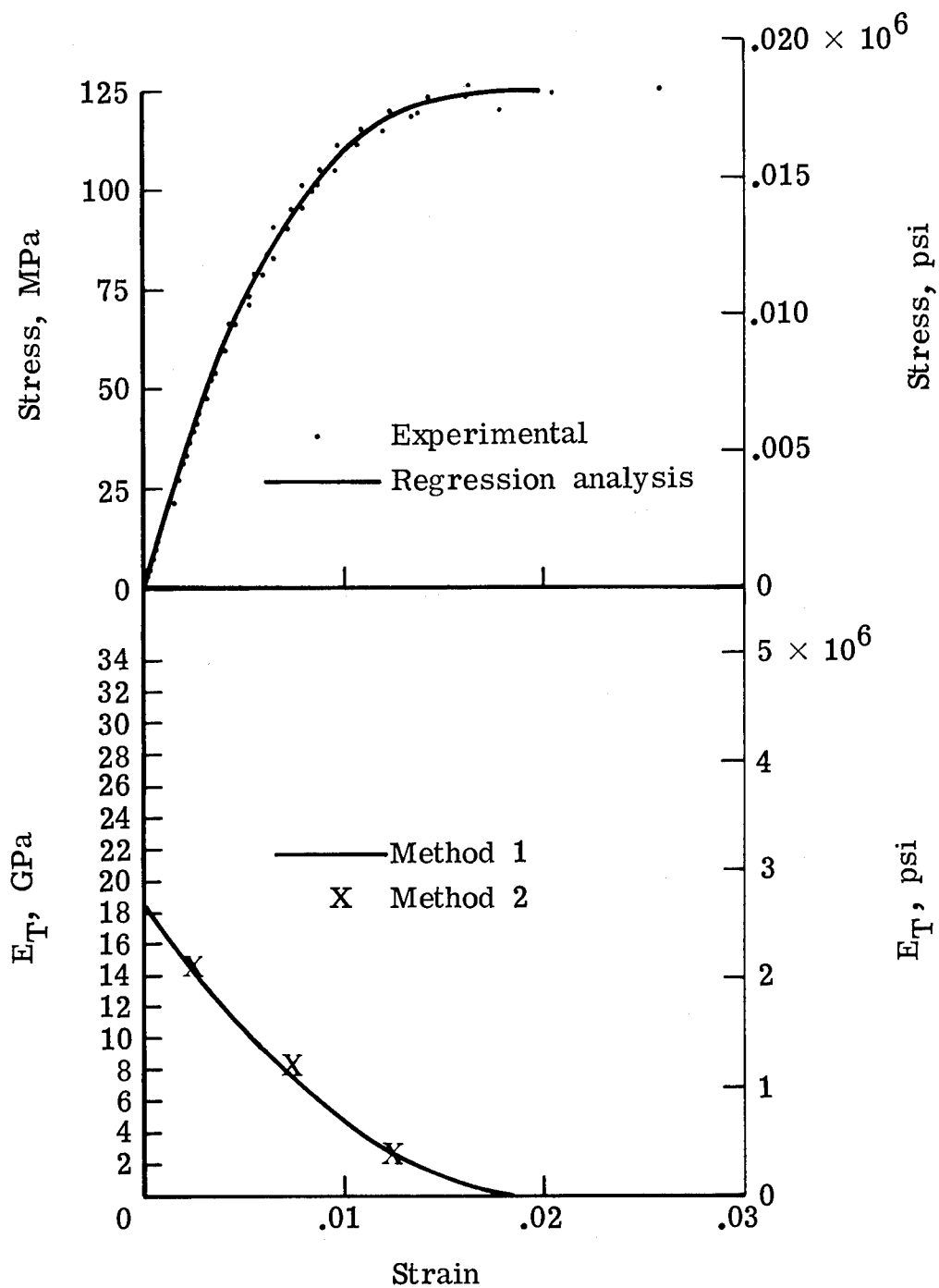
Figure 9.- Compression diagrams for [±45] 5S , HTS-2/PMR-15 composite at room temperature. w = 1.27 cm (0.5 in.); tests 69, 70, and 71.
