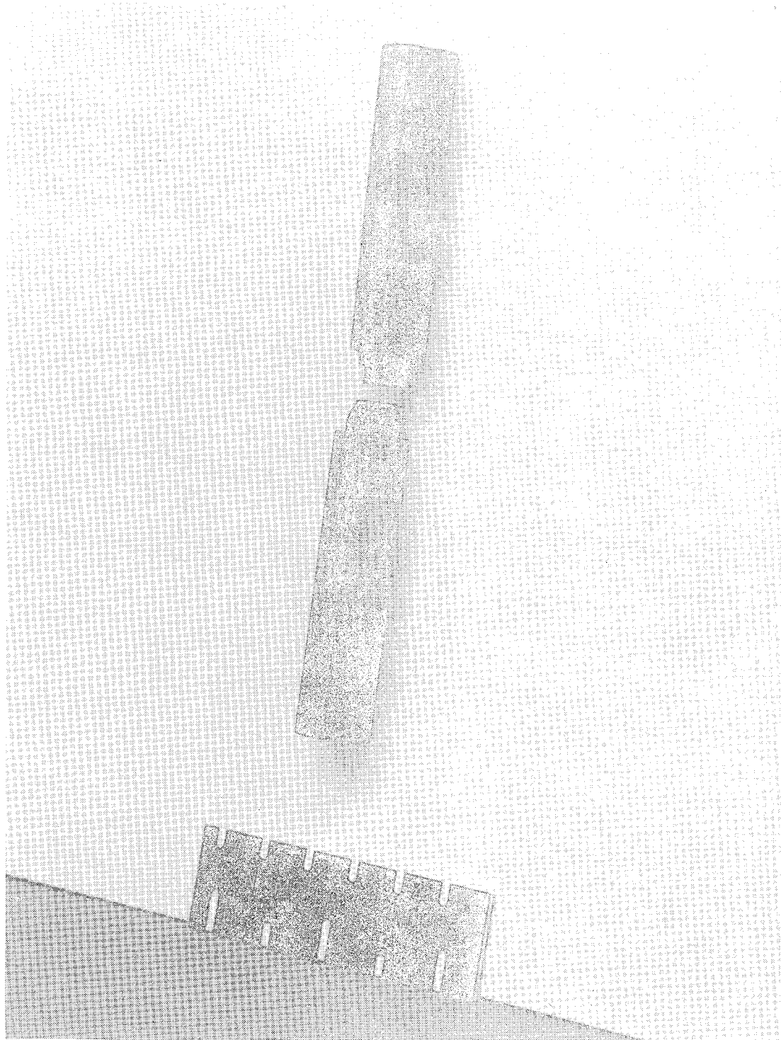
L-78-5076 Figure 20.- Failed [90] 20 , HTS-2/PMR-15 specimens. w = 1.27 cm (0.5 in.); 20 plies.
