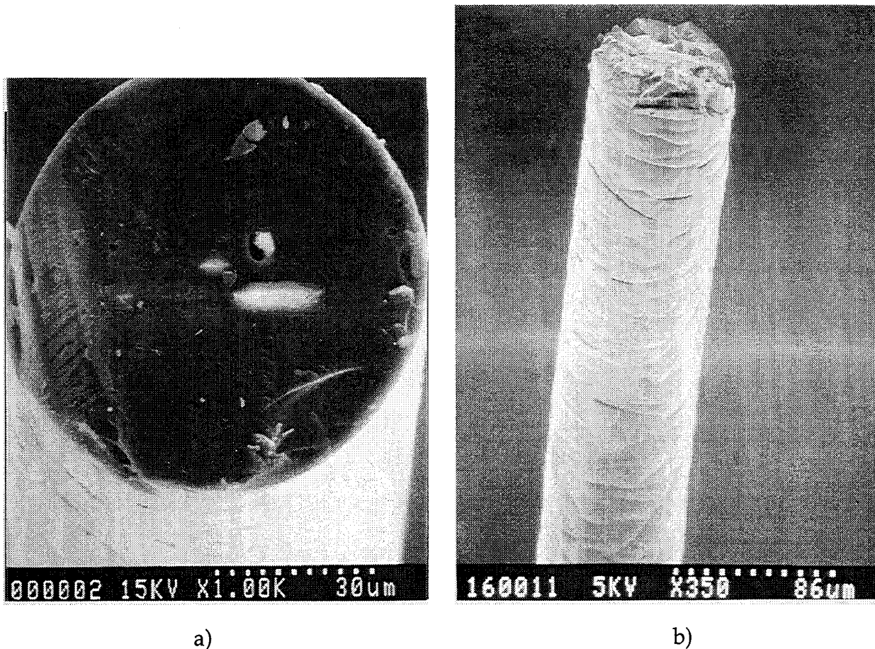
Figure 3.17: Isobutyrate-Derived YAG Fibers a) As Spun, b) After Heating Above 100°C
