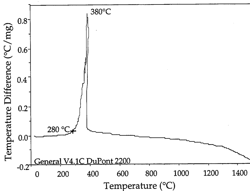
Figure 3.10: DTA of Yttrium Isobutyrate
