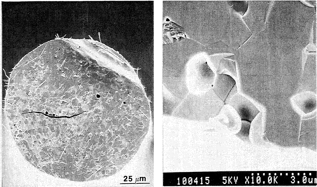
Figure 2.8: Typical Bend Stress Fracture Surface. (note fracture initiated at fiber surface)
