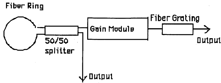
Fig 8. Experimental lay out of linear cavity laser terminated in a ring.
