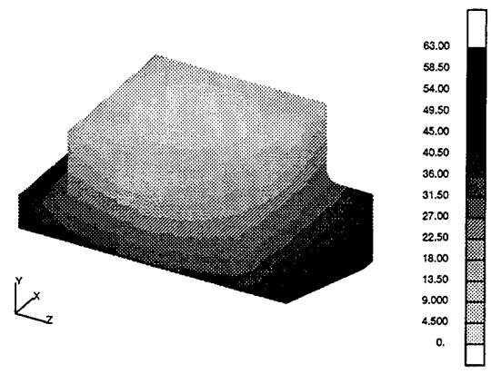
(b) Fill contours - view 2
