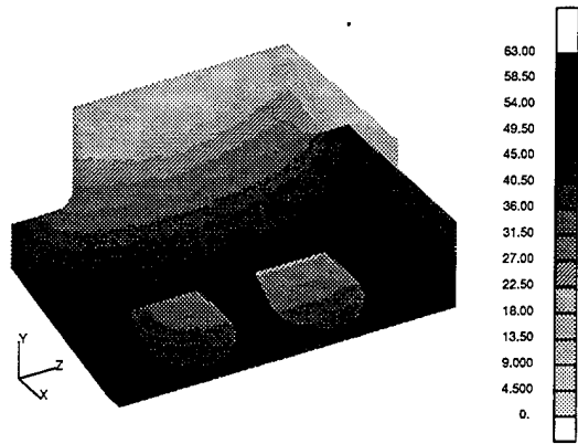
(a) Fill contours - view 1
