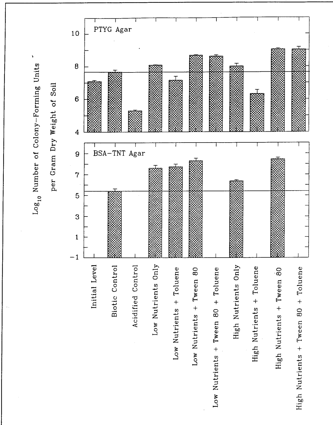
Figure 9. Response of native heterotrophic bacteria cultured on PTYG agar and bacteria cultured on BSA-TNT medium to treatment with various combinations of additives in the shake flask test with McAlester soil (Bars are the means of 3 replicates \pm standard error of the mean. The horizontal line marks total heterotrophs in the biotic control.)
