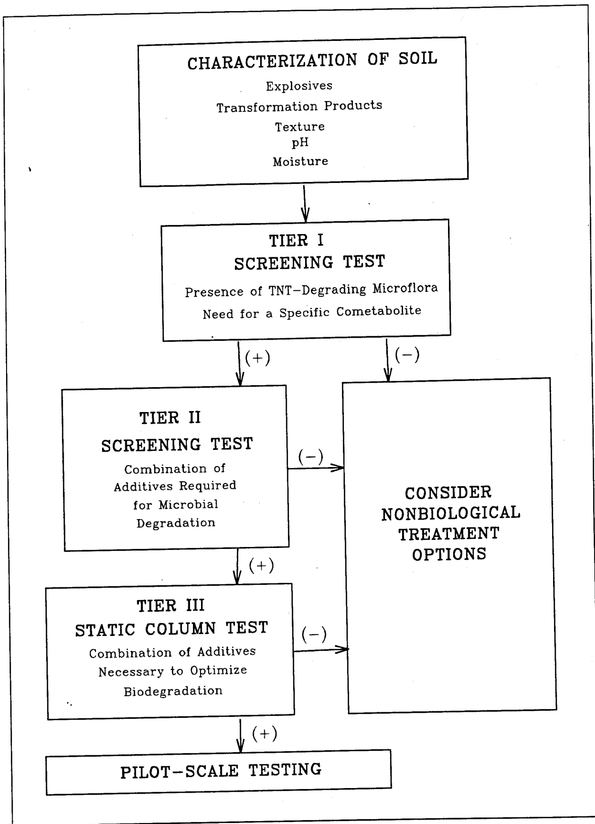
Figure 1. Three-tiered system to evaluate microbial requirements to support degradation of TNT during land-farming biotreatment of TNT-contaminated soils
