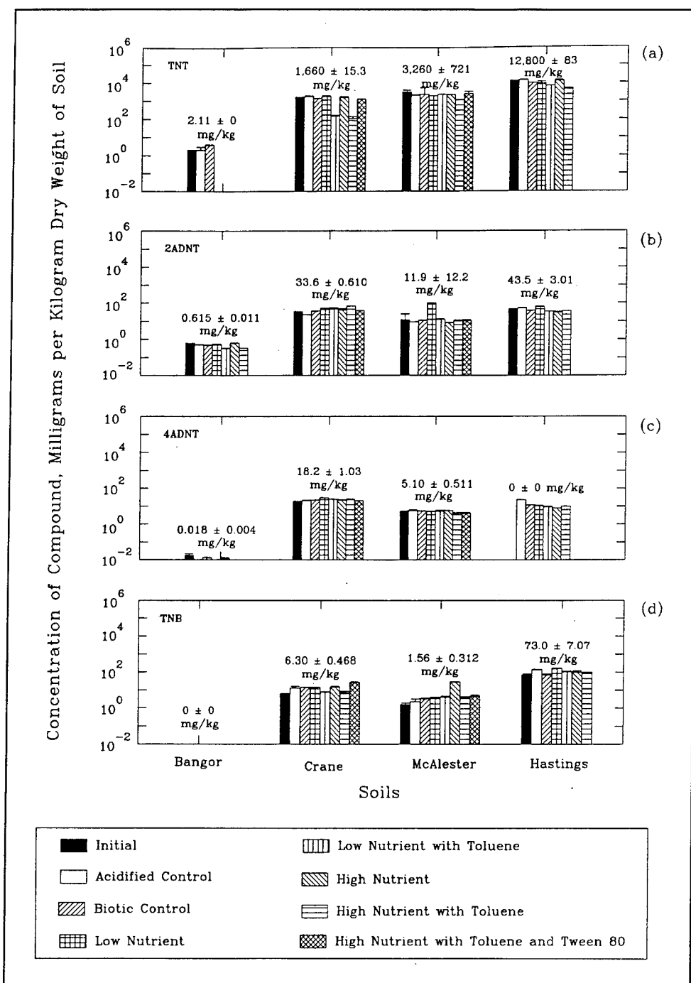
Figure 10. Comparison of removal of TNT and accumulation or removal of the TNT transformation products 2ADNT and 4ADNT and TNB in the shake test (Values given above each set of bars and the first bars in each set are the levels of each compound present at the start of treatment. The remaining bars in each set are the levels present at the end of 30 days of treatment, as indicated in the figure legend. Values given are the means of three replicates \pm the standard error of the mean.)
