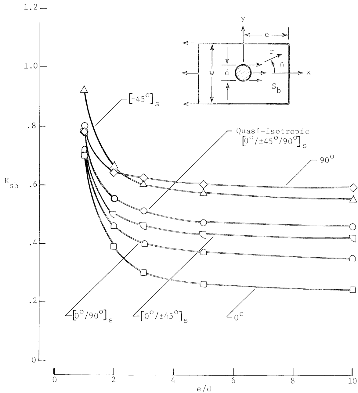
Figure 20.- \tau_{xy} stress-concentration factors for shear-out plane ( y = R ); w/d = 20 .
