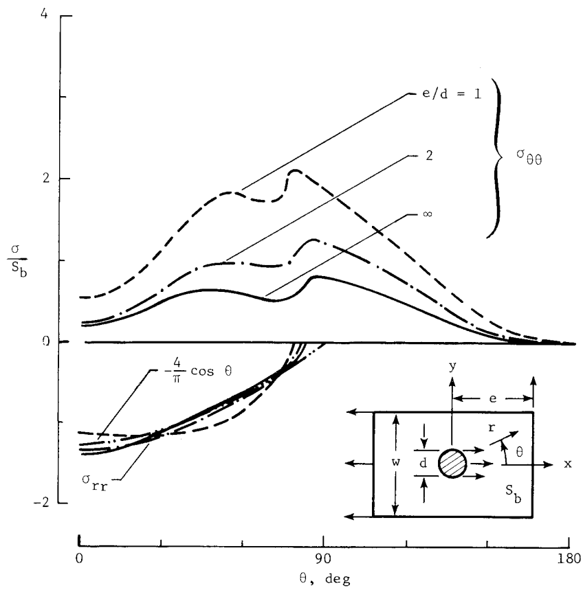
(a) Stresses along hole boundary.
