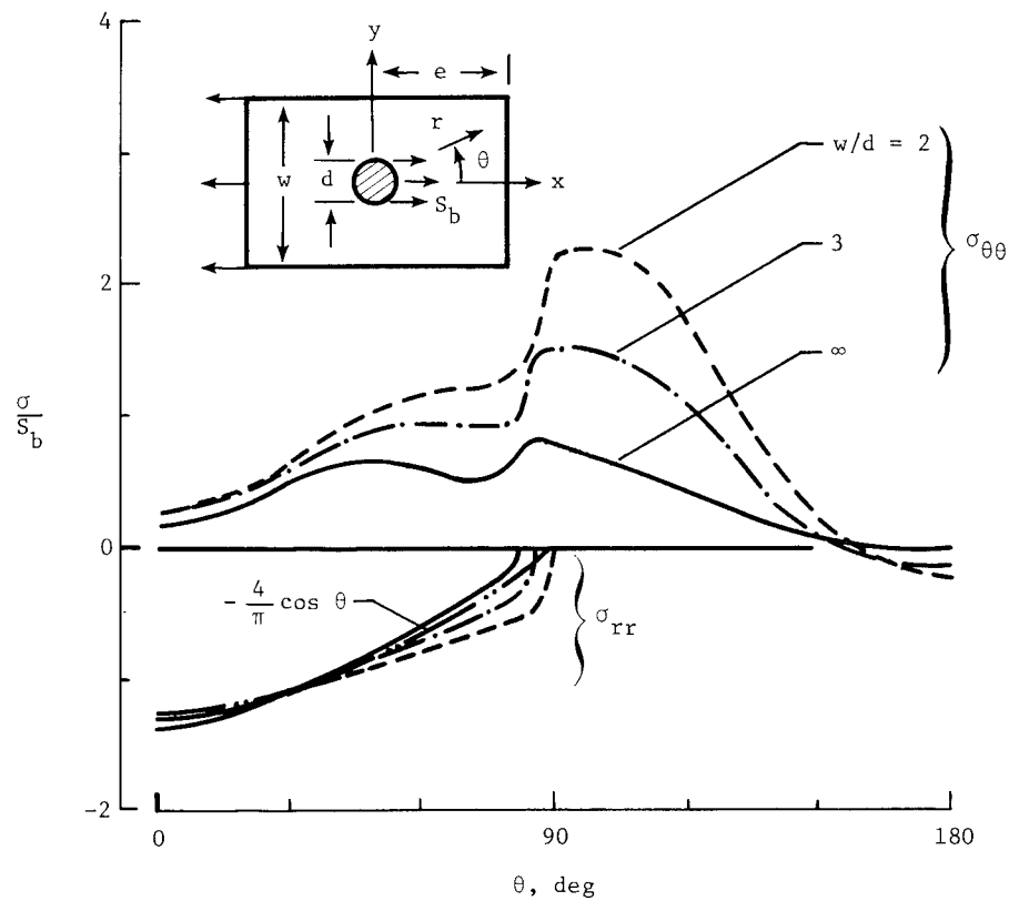
(a) Stresses along hole boundary ( r = R ).
