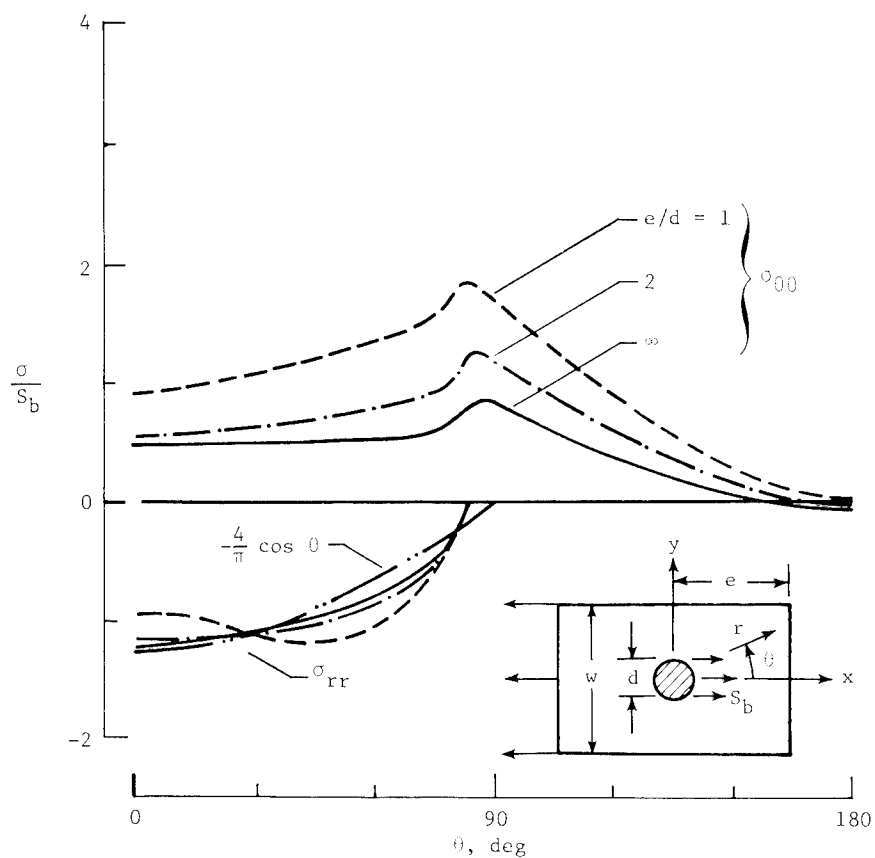
(a) Stresses along hole boundary.
