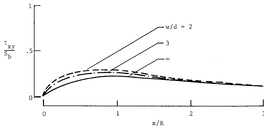
(b) Shear stress along shear-out plane.
