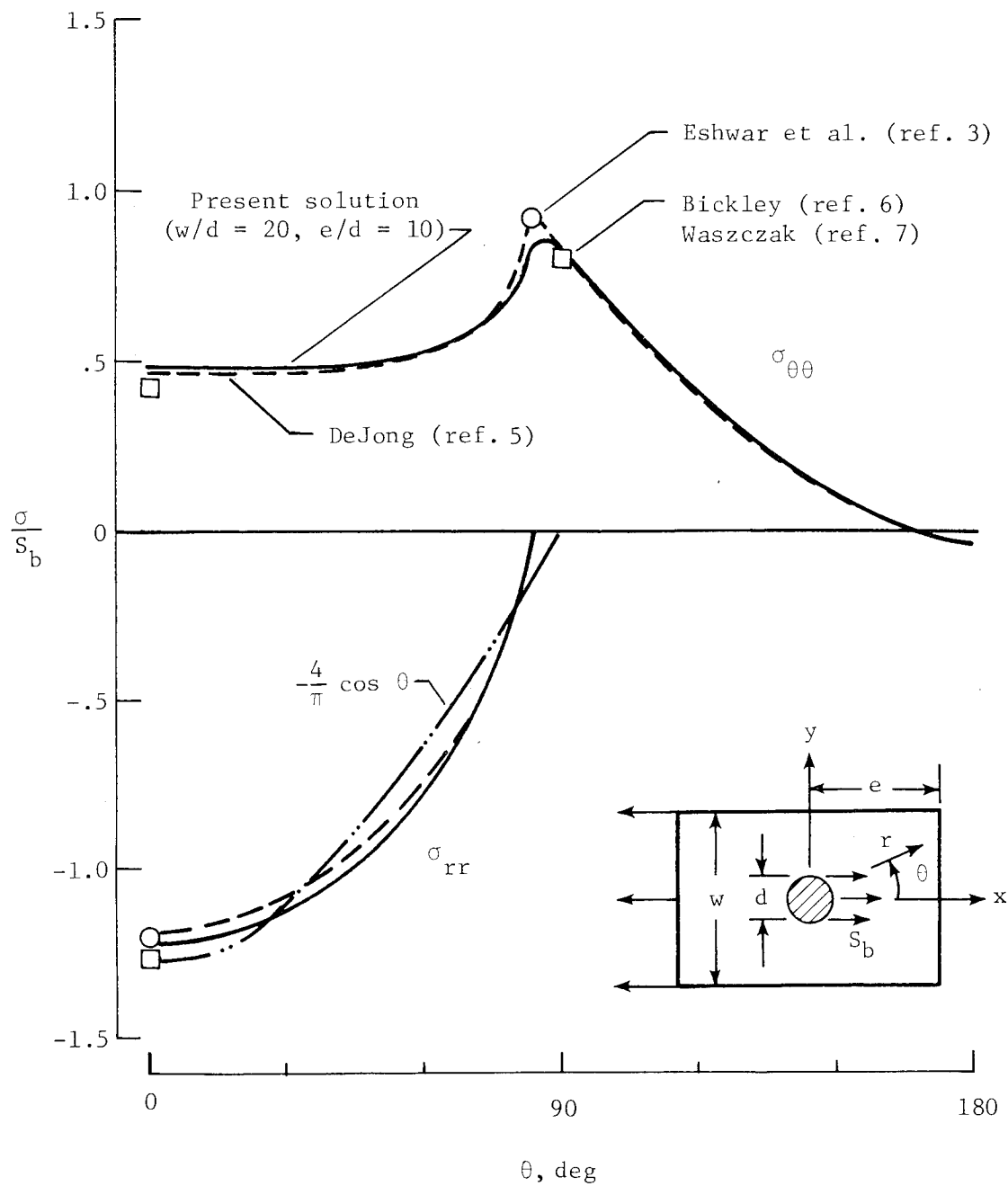
Figure 3.- Stresses in quasi-isotropic laminate loaded by a rigid pin; w/d = 20 , e/d = 10 .
