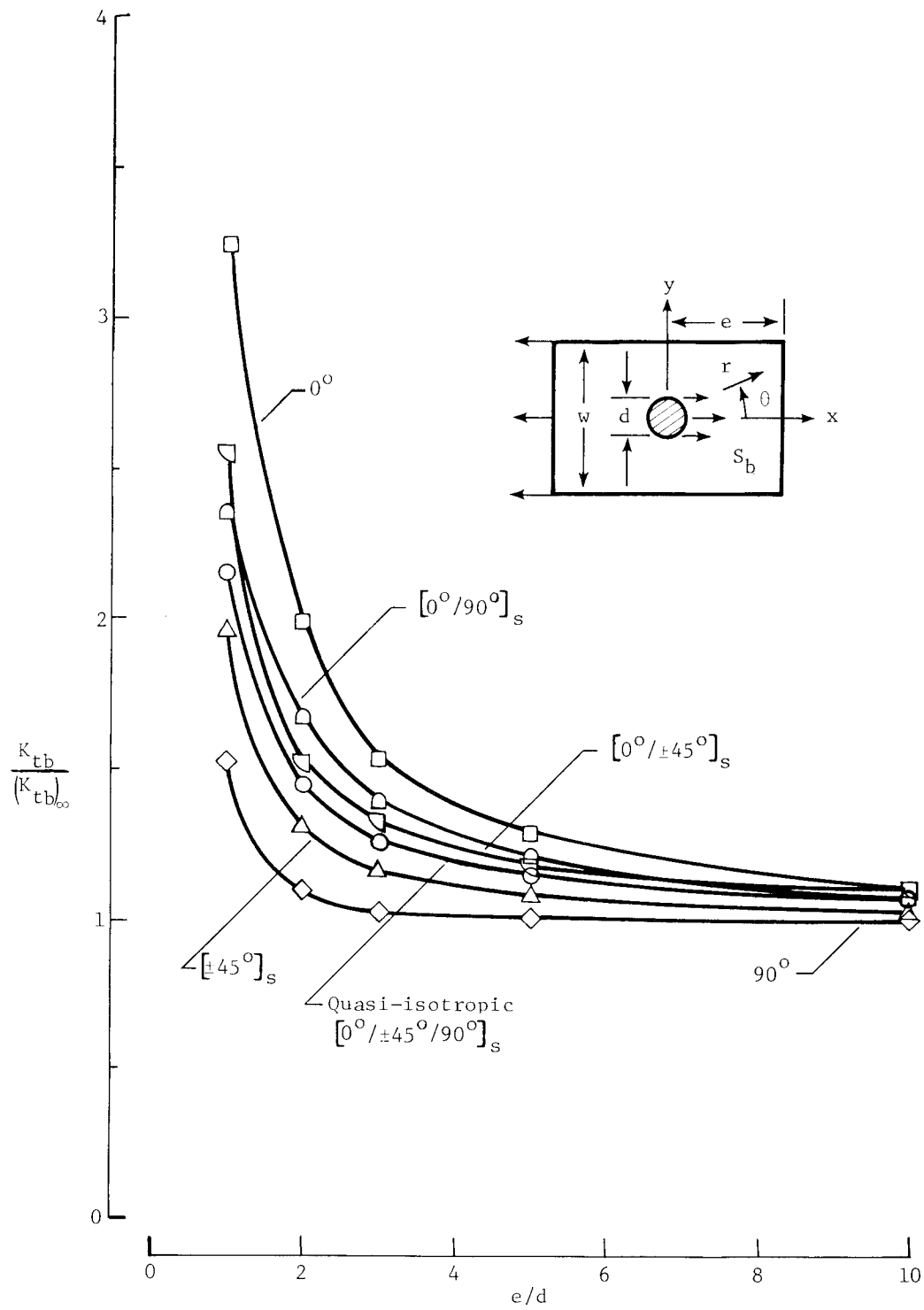
Figure 19.- Normalized \sigma_{\theta\theta} stress-concentration factors as a function of e/d ; w/d = 20 .
