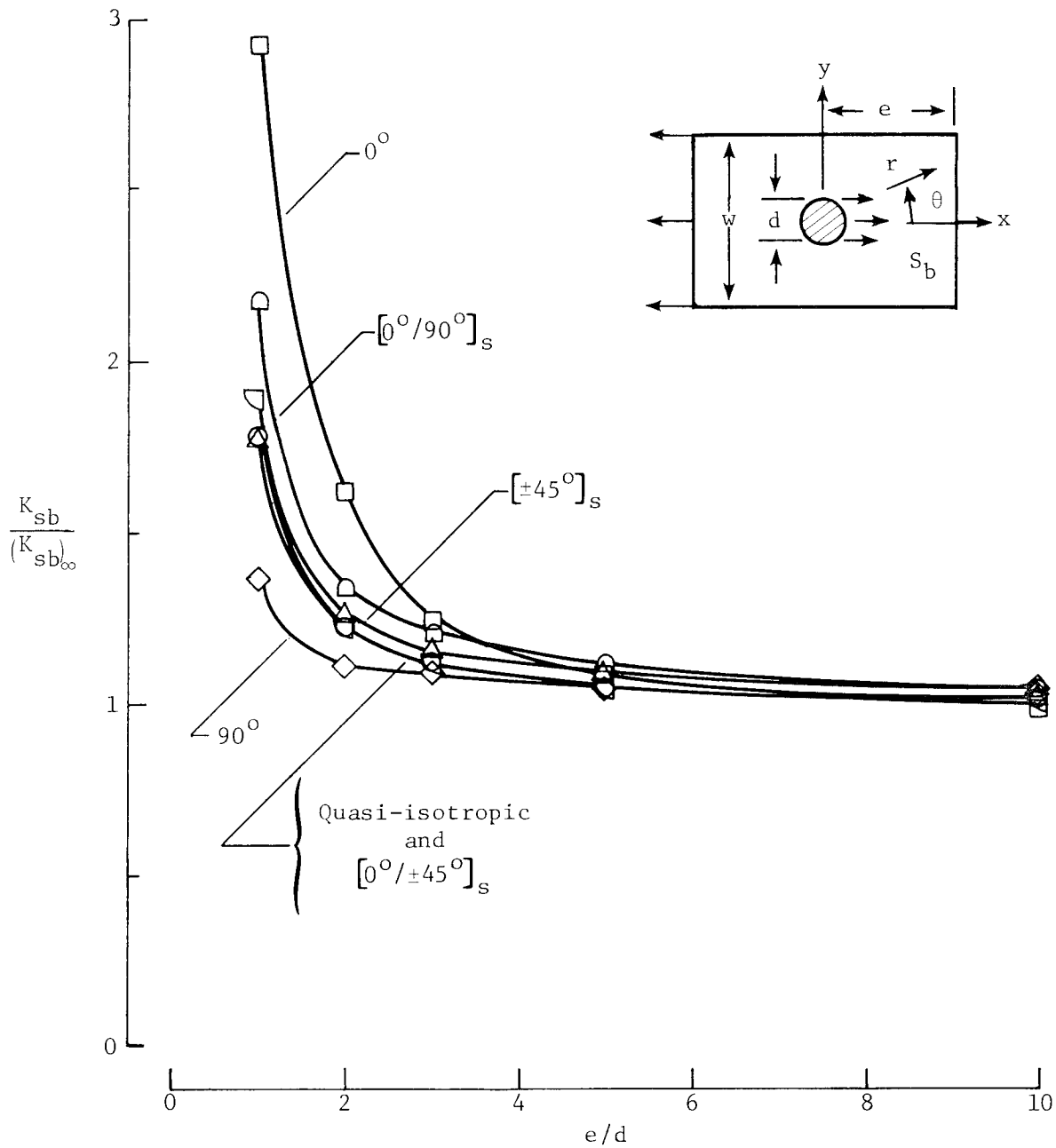
Figure 21.- Normalized \tau_{xy} stress-concentration factors for shear-out plane ( y = R ); w/d = 20 .
