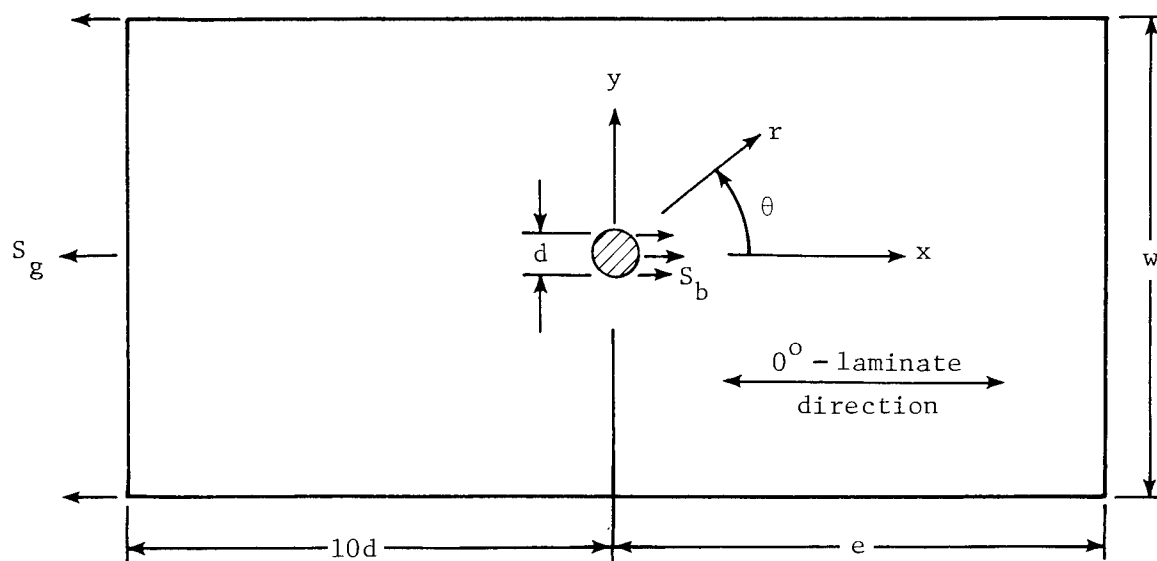
Figure 1.- Laminate configuration and loading.
