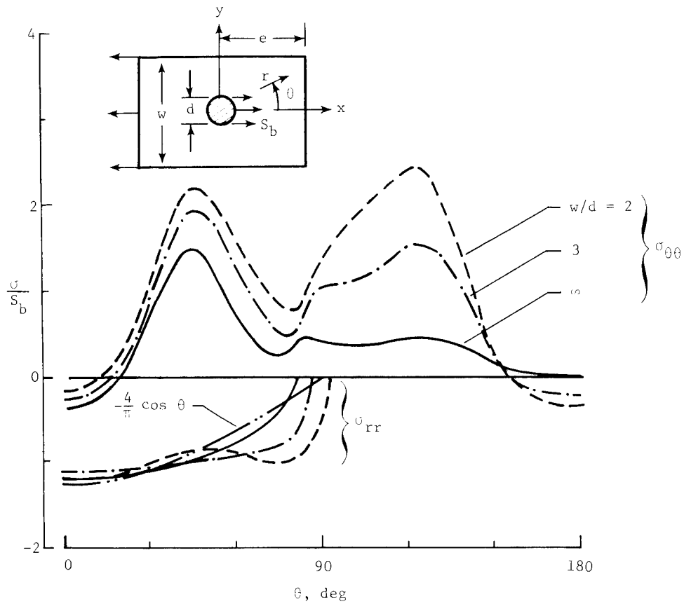
(a) Stresses along hole boundary ( r = R ).
