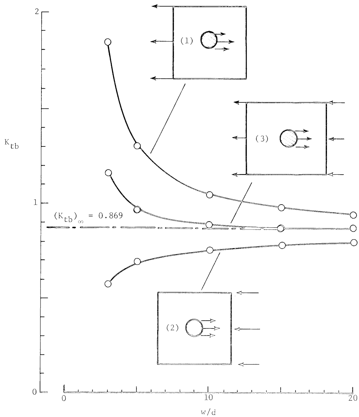
Figure 22.- \sigma_{\theta\theta} stress-concentration factors for a square quasi-isotropic laminate loaded by a rigid pin.
