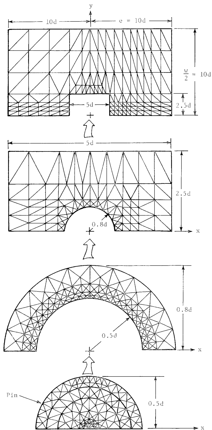
Figure 2.- Finite-element model.
