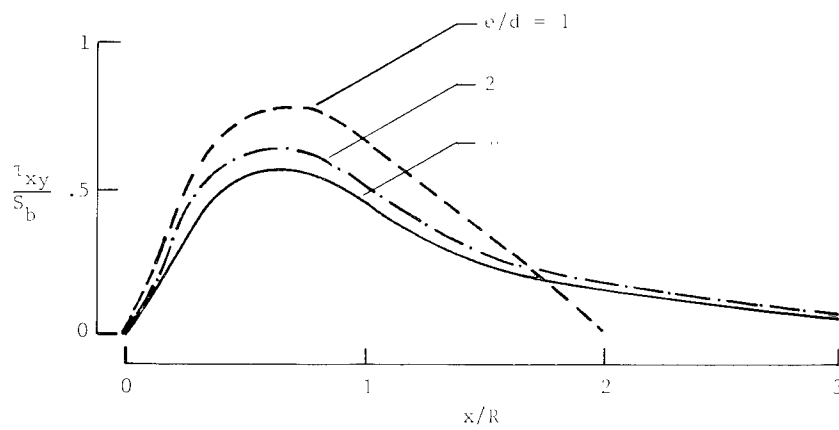
(b) Shear stress along shear-out plane ( y = R ).
