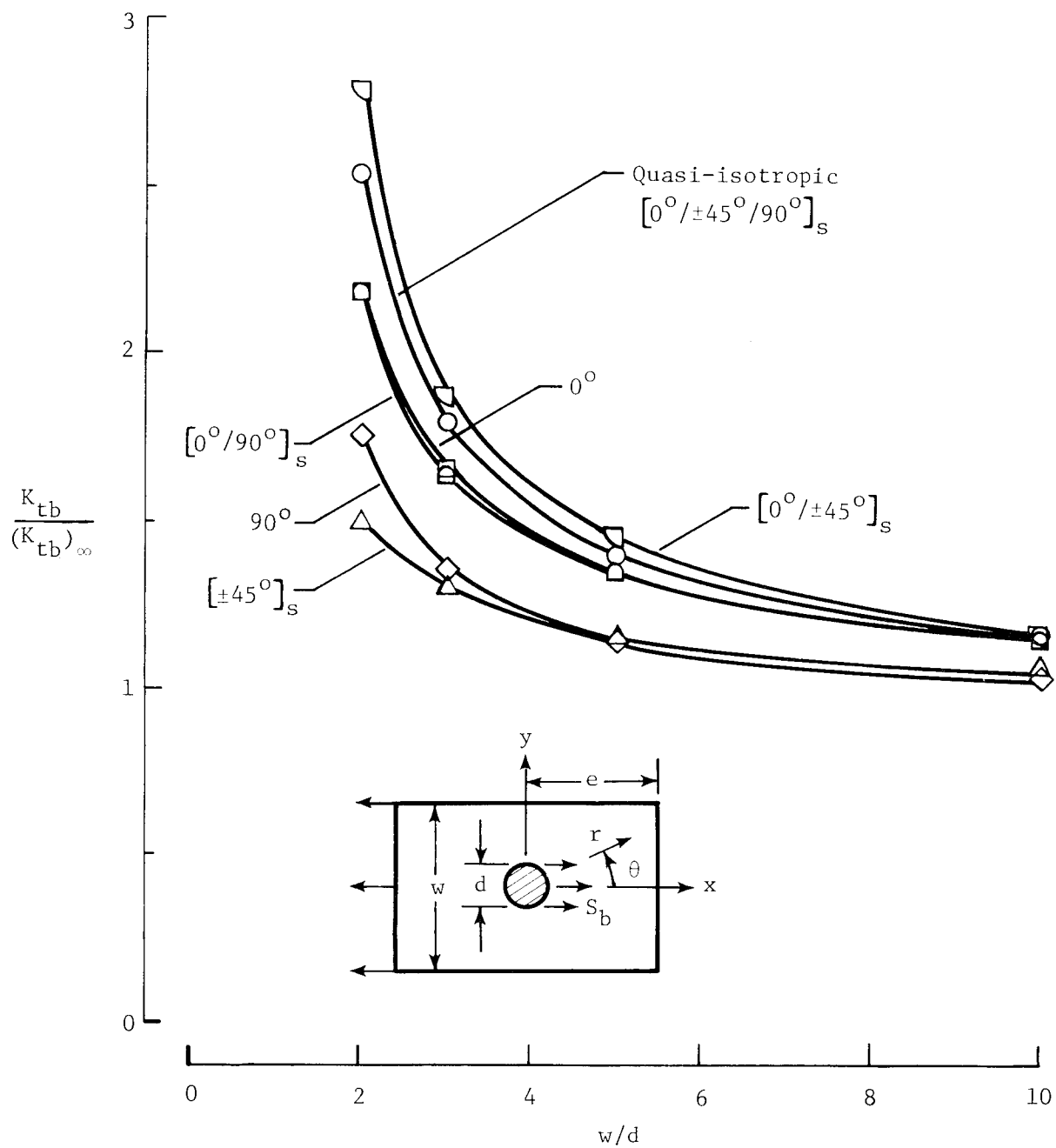
Figure 11.- Normalized \sigma_{\theta\theta} stress-concentration factors as a function of w/d ; e/d = 10 .
