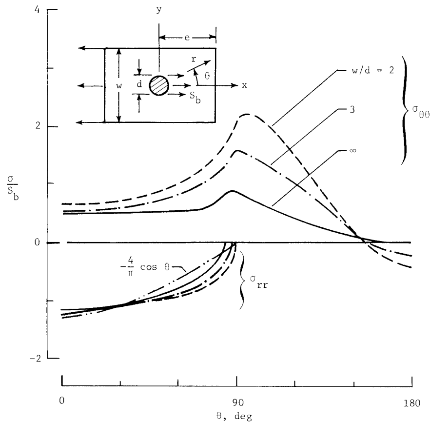
(a) Stresses along hole boundary ( r = R ).
