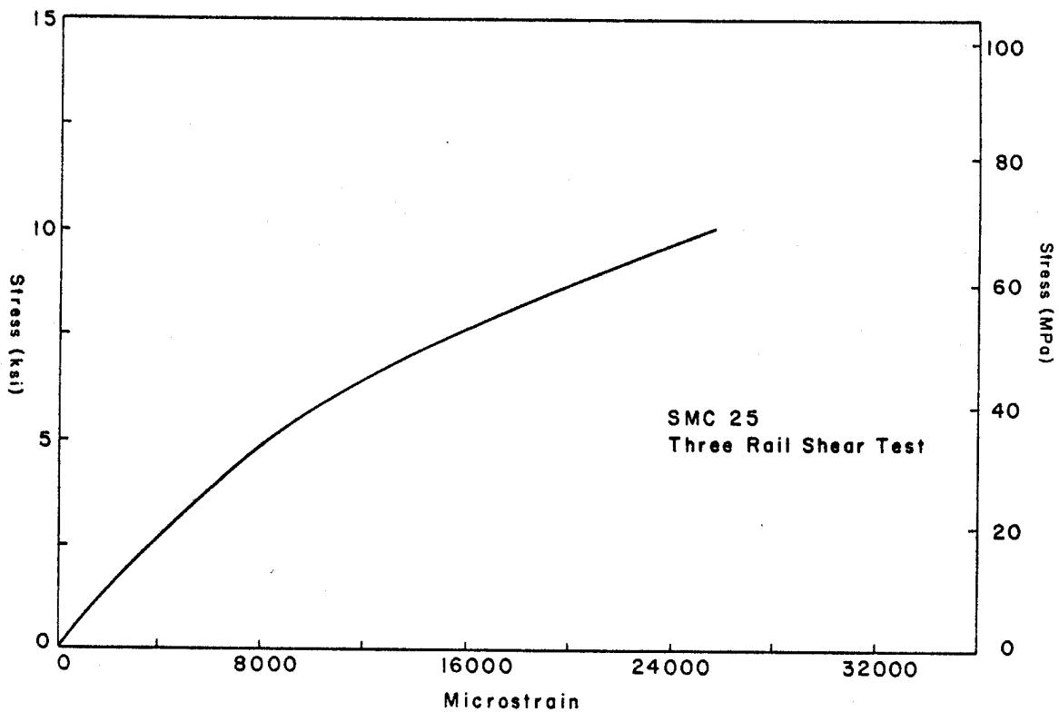
FIGURE 69. SHEAR STRESS-STRAIN RESULTS - THREE RAIL SMC-25
