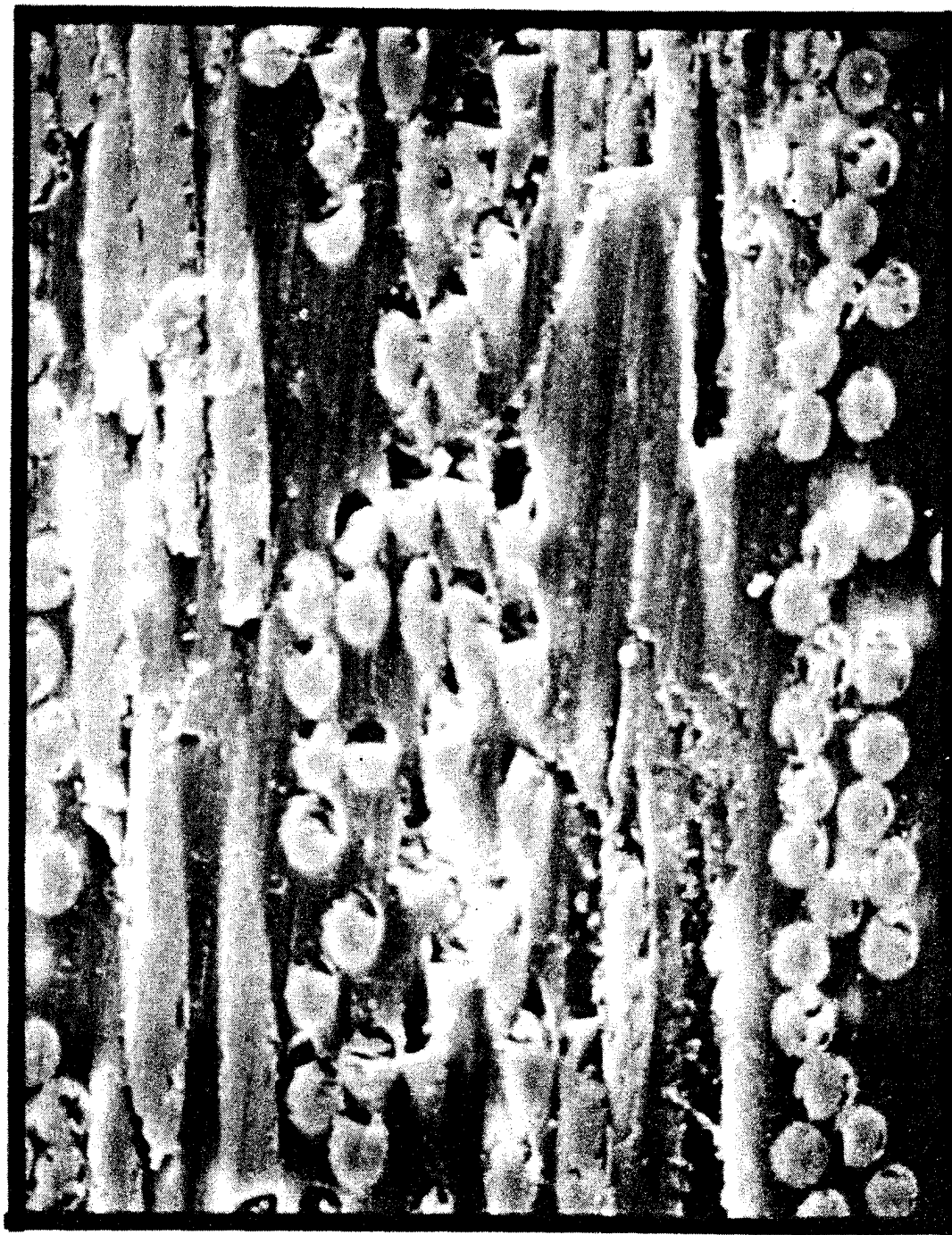
FIGURE 56. SCANNING ELECTRON MICROGRAPH - SMC - 65
