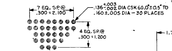
HOLE PLAN H SCALE 1/1
