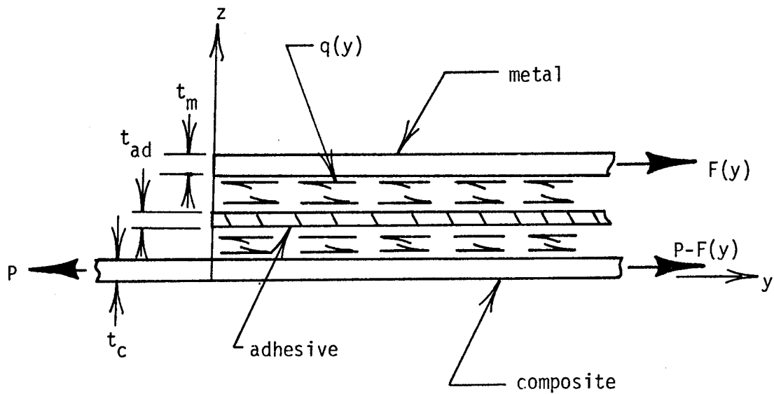
(b) Freebody for one-dimensional solution
