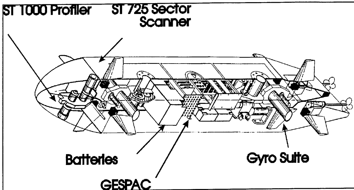
Figure 1.1 NPS Phoenix AUV
