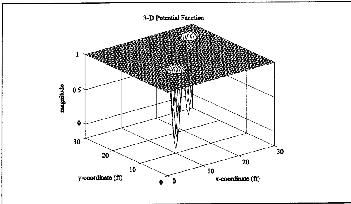
Figure 4.1 Open Environment Potential Function with Two Obstacles
