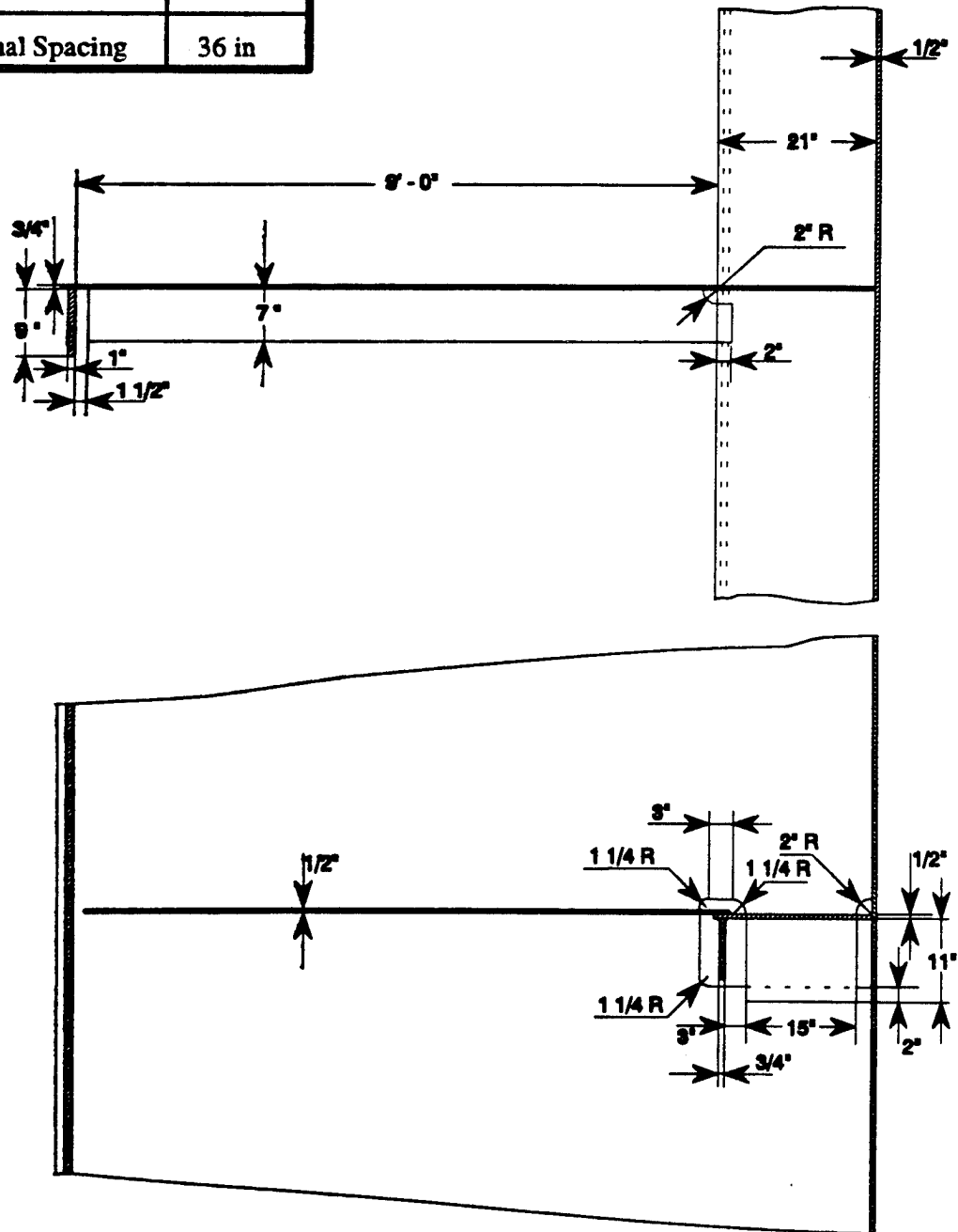
Figure 25: Case II: Construction Drawing for Detail 11-C
