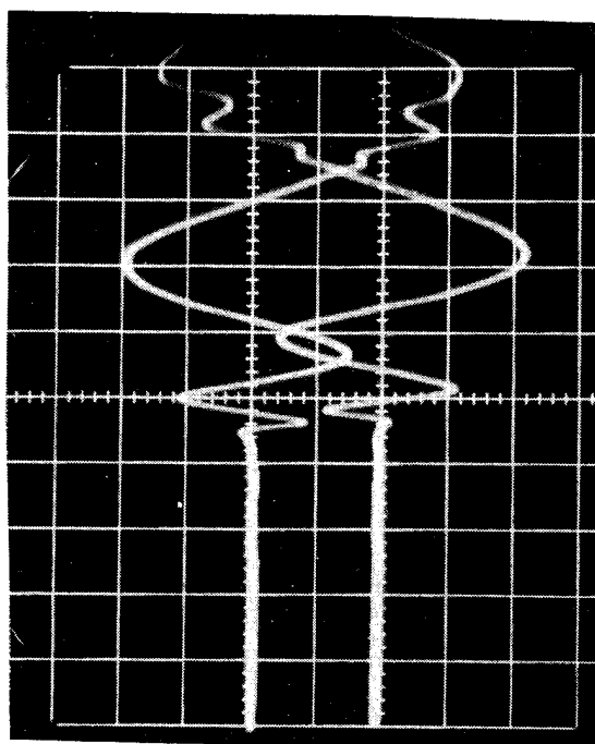
Fig. 35 STRAIN GAGE SIGNALS ON OPPOSITE FACES OF TRANSVERSELY IMPACTED [\text{O}_2/\text{+45}]_{2\text{s}} GRAPHITE/EPOXY SPECIMEN 9GA-1 ALONG x-AXIS (Sweep: 20 \mu\text{sec}/\text{div} )
