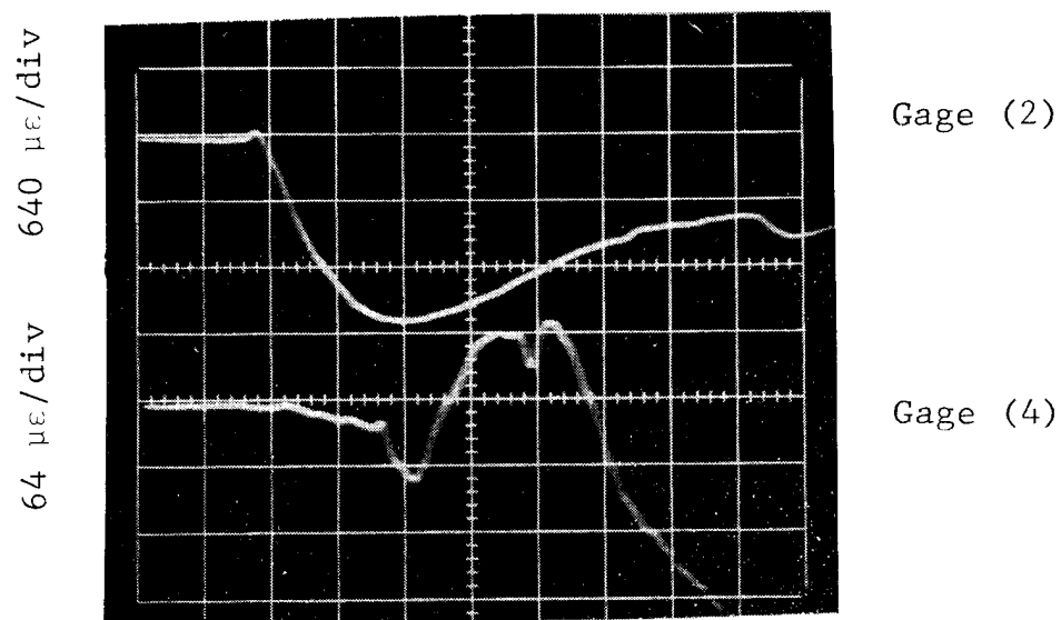
(b) 20 \mu\text{sec}/\text{div}
