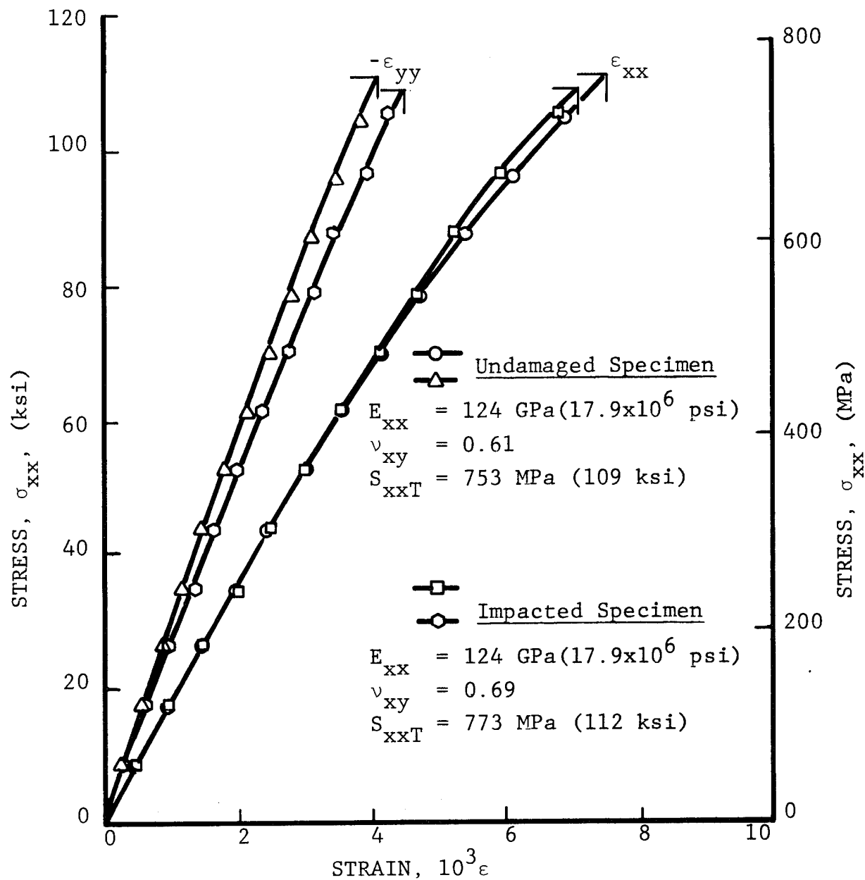
Fig. 44 STRAINS IN [0_2/+45]_{2s} BORON/EPOXY SPECIMENS UNDER UNIAXIAL TENSION FROM UNDATED AND IMPACTED LAMINATES (Impact Velocity: 210 \text{ ms}^{-1} ; 690 \text{ ft/sec} )
