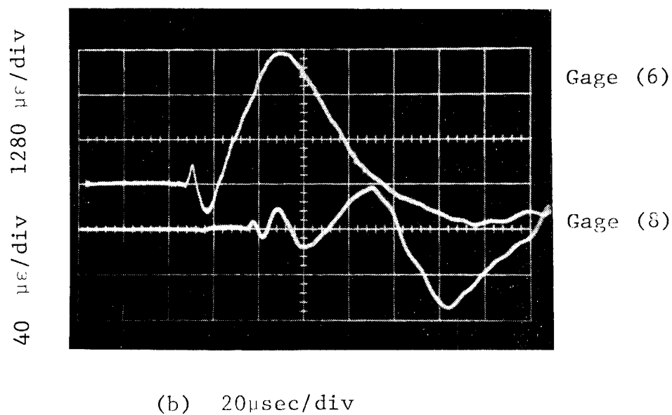
Fig. 29 STRAIN GAGE SIGNALS IN TRANSVERSELY IMPACTED [0_2/\pm 45]_{2s} BORON/EPOXY SPECIMEN 9BA-1 ALONG HORIZONTAL AXIS.
