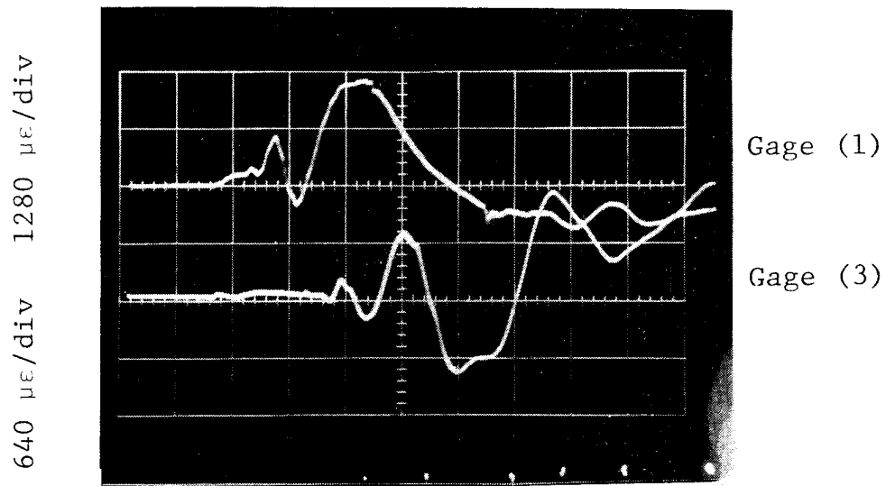
(a) 20 \mu\text{sec}/\text{div}
