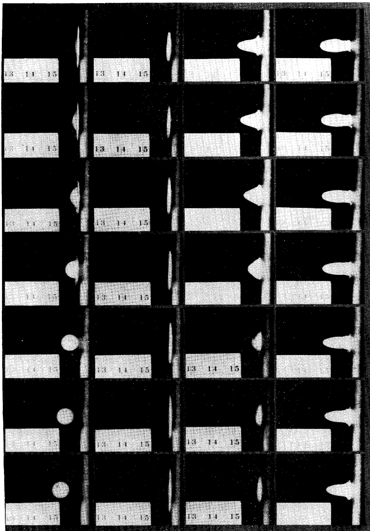
Fig. 62 IMPACT OF 7.9 mm (5/16 in.) DIAMETER SILASTIC SPHERE ON [0_2/\pm 45]_2s BORON/EPOXY PLATE AT 180 \text{ ms}^{-1} (590 ft/sec). (Camera Speed: 85,700 frames/second).
