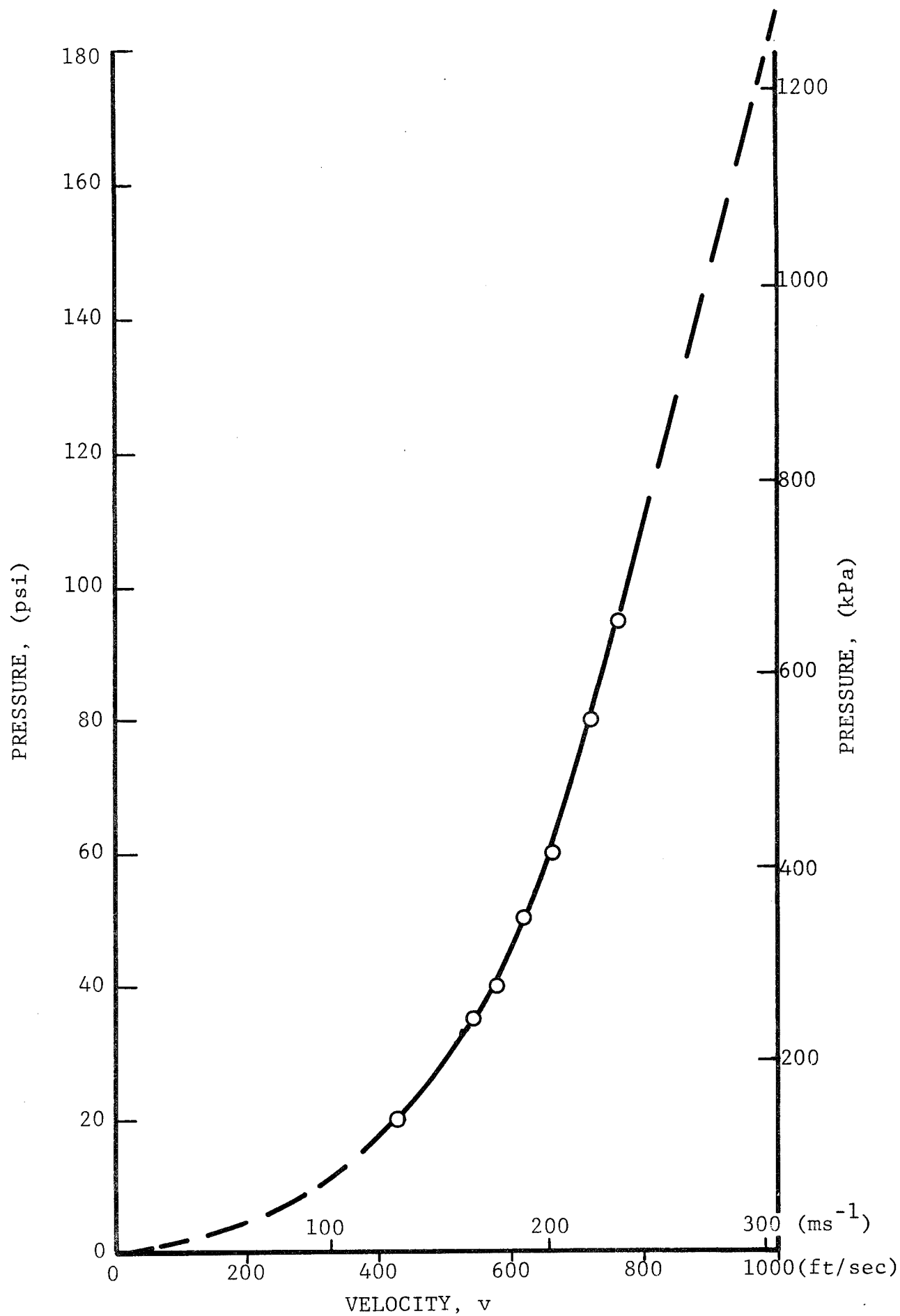
Fig. 7 VELOCITY OF 1.43 cm (9/16 in.) DIAMETER RTV PROJECTILE AS A FUNCTION OF CHAMBER PRESSURE
