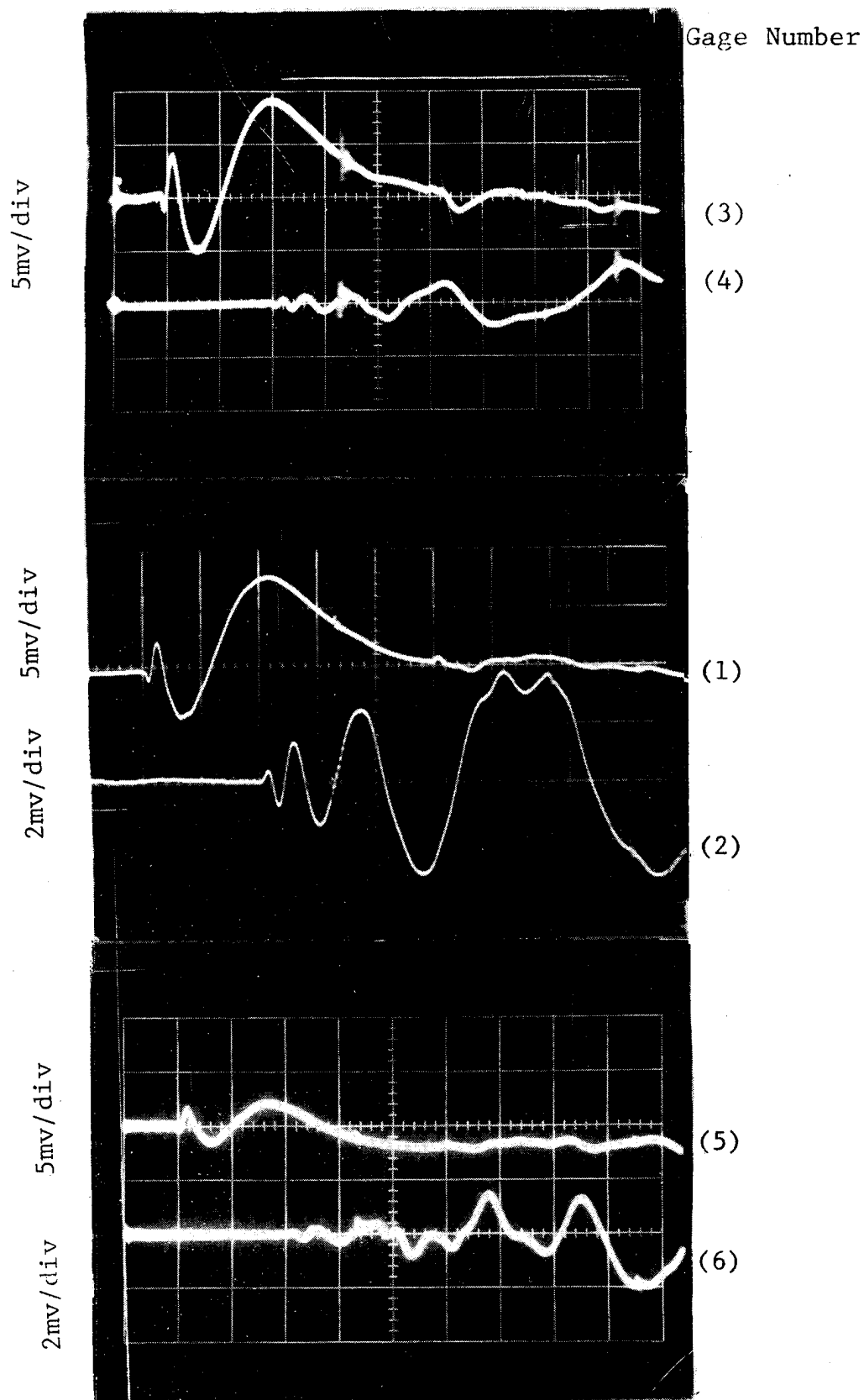
Fig. 13 STRAIN GAGE SIGNALS IN TRANSVERSELY IMPACTED [+45]_{2s} BORON/EPOXY LAMINATE (SWEEP: 20 \mu\text{sec/div} ; Refer to Fig. 3-2 for Gage Layout).
