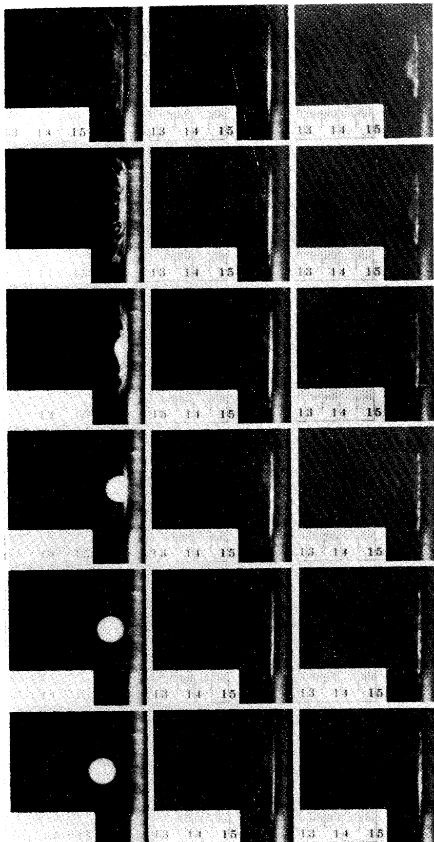
Fig. 64 IMPACT OF 7.9 mm (5/16 in) DIAMETER SILASTIC SPHERE ON [0 2 /+45] 2 s BORON/EPOXY PLATE AT 242 ms -1 (794 ft/sec). (Camera Speed: 85,700 frames/second)
