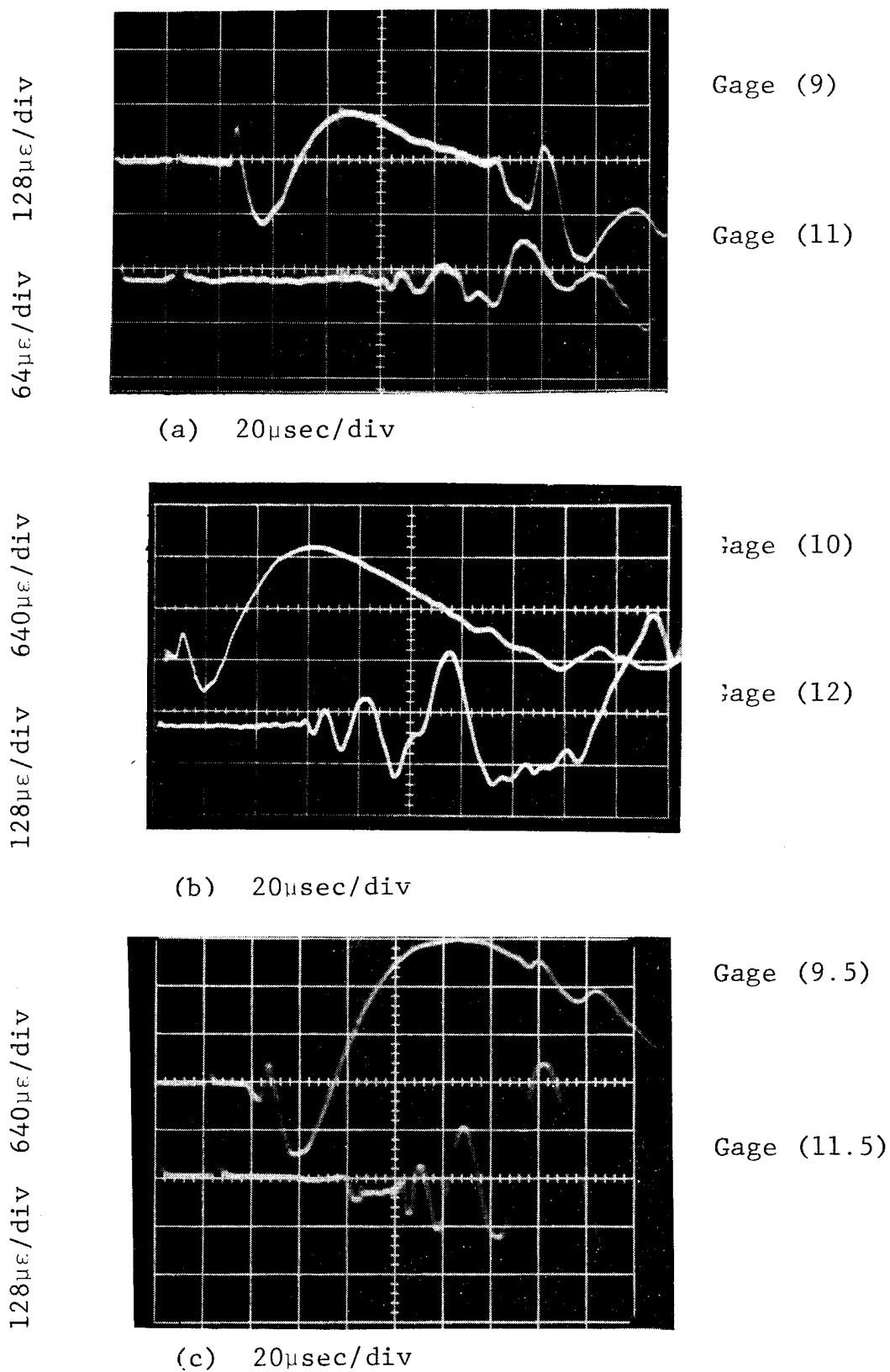
Fig. 27 STRAIN GAGE SIGNALS ALONG 45-DEGREE AXIS IN TRANSVERSELY IMPACTED [0 16 ] GRAPHITE/EPOXY SPECIMEN (a) Gages in y-direction 7.62 cm (3 in.) apart (b) Gages in x-direction 7.62 cm (3 in.) apart (c) Gages in 45-degree direction 7.62 cm (3 in.) apart
