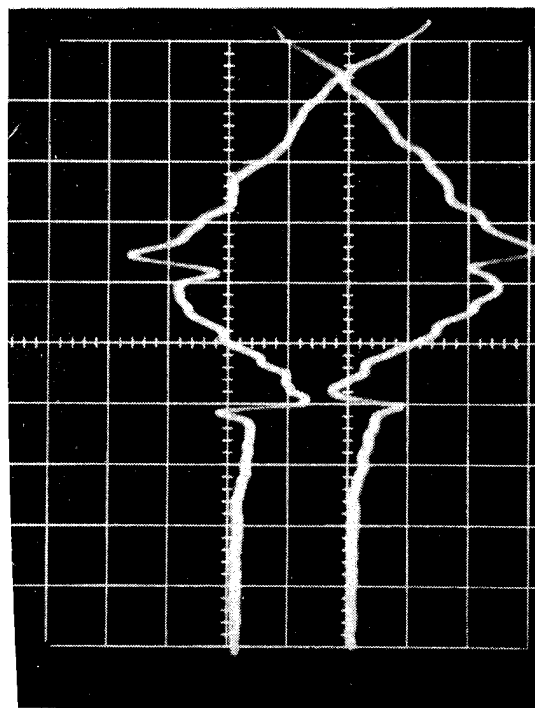
Fig. 34 STRAIN GAGE SIGNALS ON OPPOSITE FACES OF TRANSVERSELY IMPACTED [O_2/\pm 45]_{2s} GRAPHITE/EPOXY SPECIMEN 9CA-1 ALONG y-AXIS (Sweep: 20 \mu sec/div)
