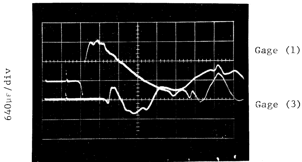
(a) 20 \mu\text{sec}/\text{div}
