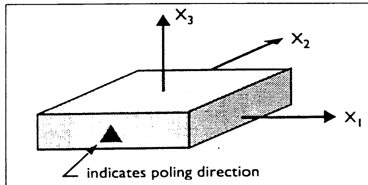
Figure 4.2. [Ref. 4] Typical Piezoceramic Coordinate System
