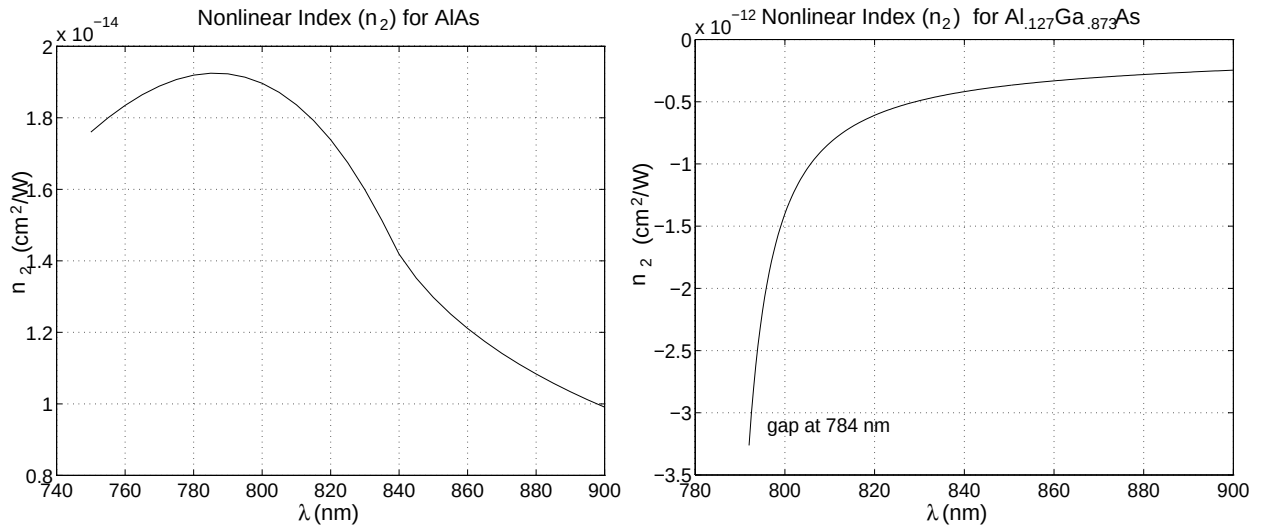
Figure 14. Calculated Nonlinear Index of Refraction ( n_2 ) for \text{Al}_x\text{Ga}_{1-x}\text{As}
