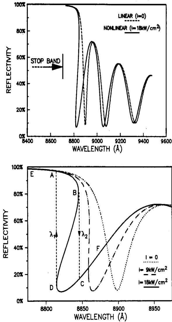
Figure 17. Plot of Linear vs Nonlinear Index Spectral Reflectivity in a DBR (top) and the Reflectivity Bistability Obtained (bottom) as Intensity is Increased (After He et al )
