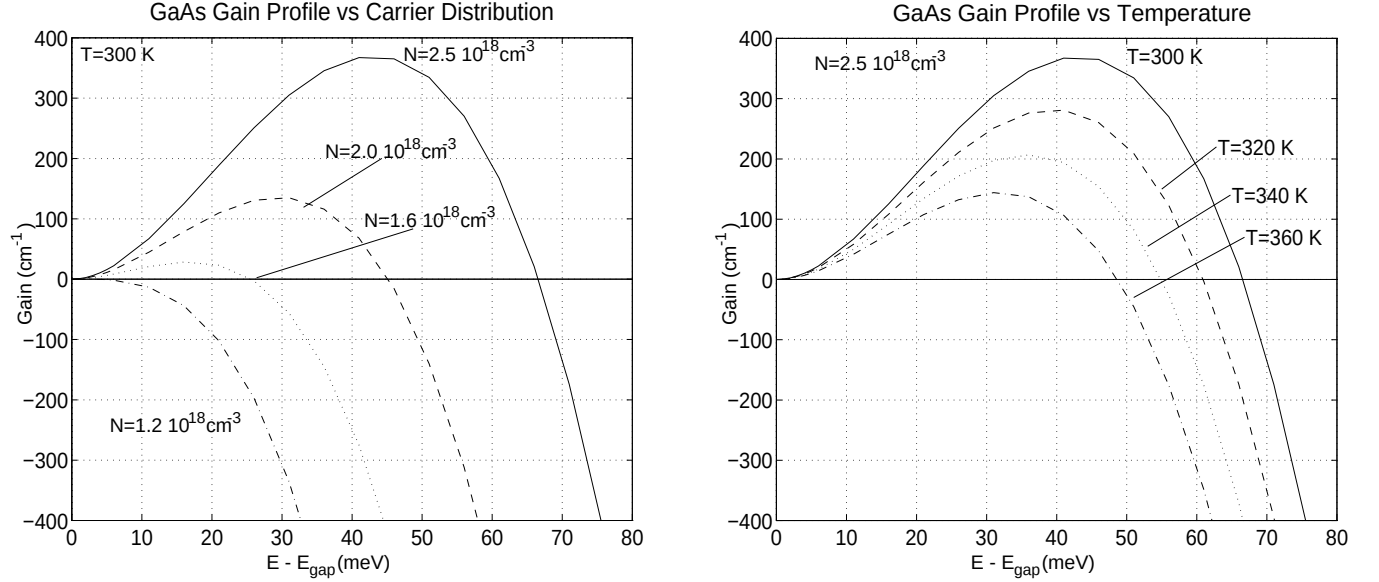
Figure 10. Effects of Carrier Density and Temperature
