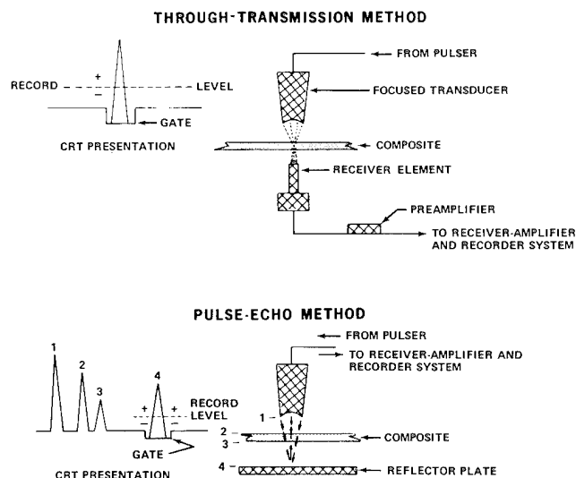
FIGURE 2. ULTRASONIC INSPECTION TECHNIQUES
