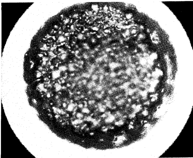
Figure 4. - Photomicrographs of PMMA surfaces exposed to glass bead impingement at 0.27-megapascal gas pressure as function of time.
