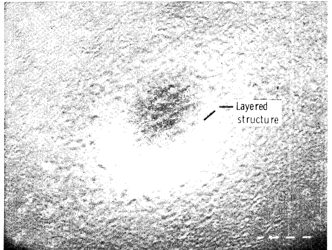
Figure 6. - Photomicrographs of PTFE surfaces exposed to glass bead impingement at 0, 27-megapascal gas pressure as function of time.
