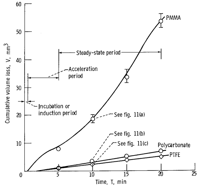
Figure 12. - Cumulative erosion - time curves for plastic materials at 0.27-megapascal gas pressure.
