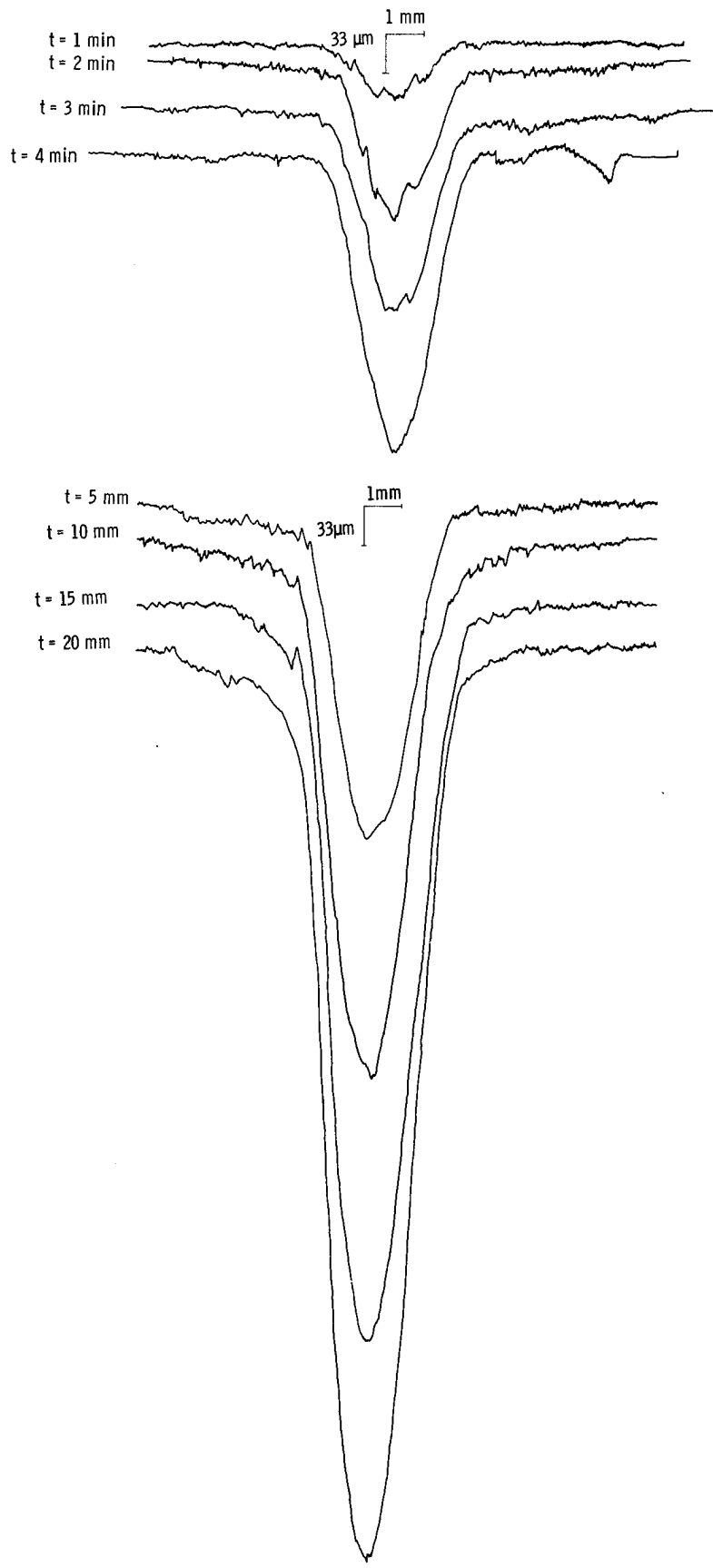
Figure 9. - Surface traces on PTFE as function of time.
