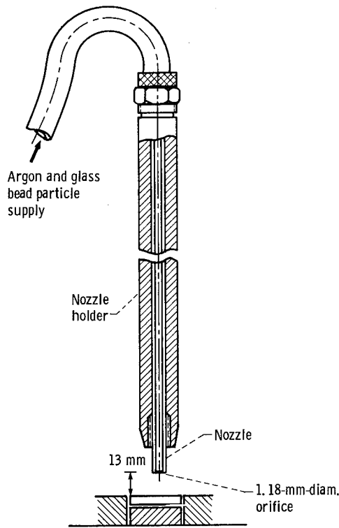
Figure 3. - Schematic diagram of nozzle holder arrangement for impingement apparatus at normal incidence.
