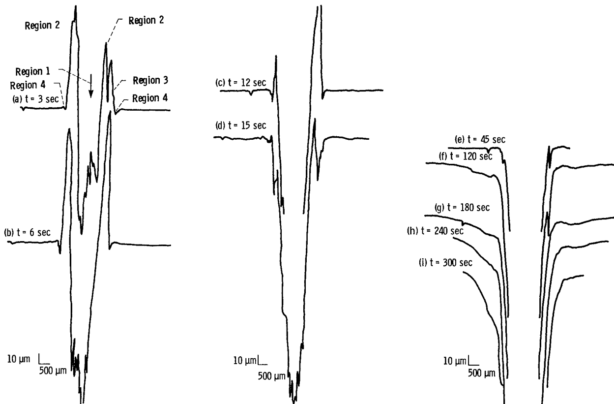
Figure 8. - Surface traces on polycarbonate as function of time.
