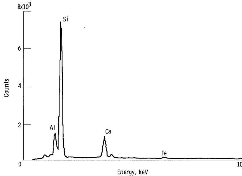
Figure 2. - EDS analysis of glass beads.
