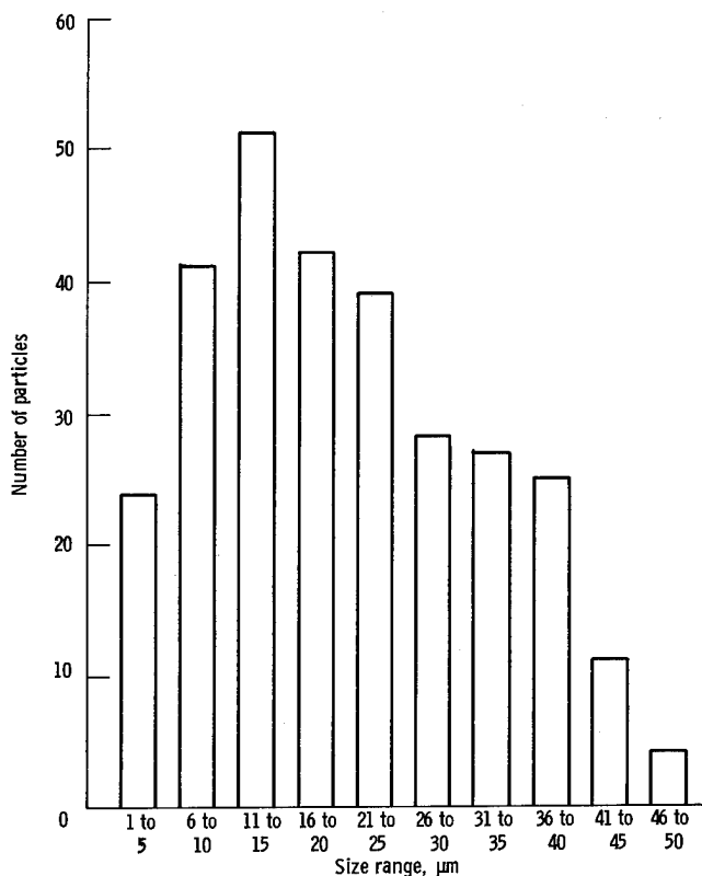
Figure 1. - Particle size distribution of glass beads.
