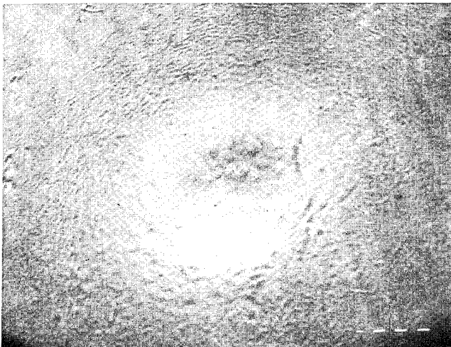
Figure 6. - Photomicrographs of PTFE surfaces exposed to glass bead impingement at 0, 27-megapascal gas pressure as function of time.
