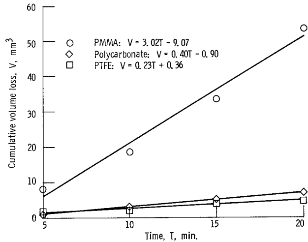
Figure 13. - Least squares fit of data derived from glass bead erosion of plastic materials at 0.27-megapascal gas pressure.
