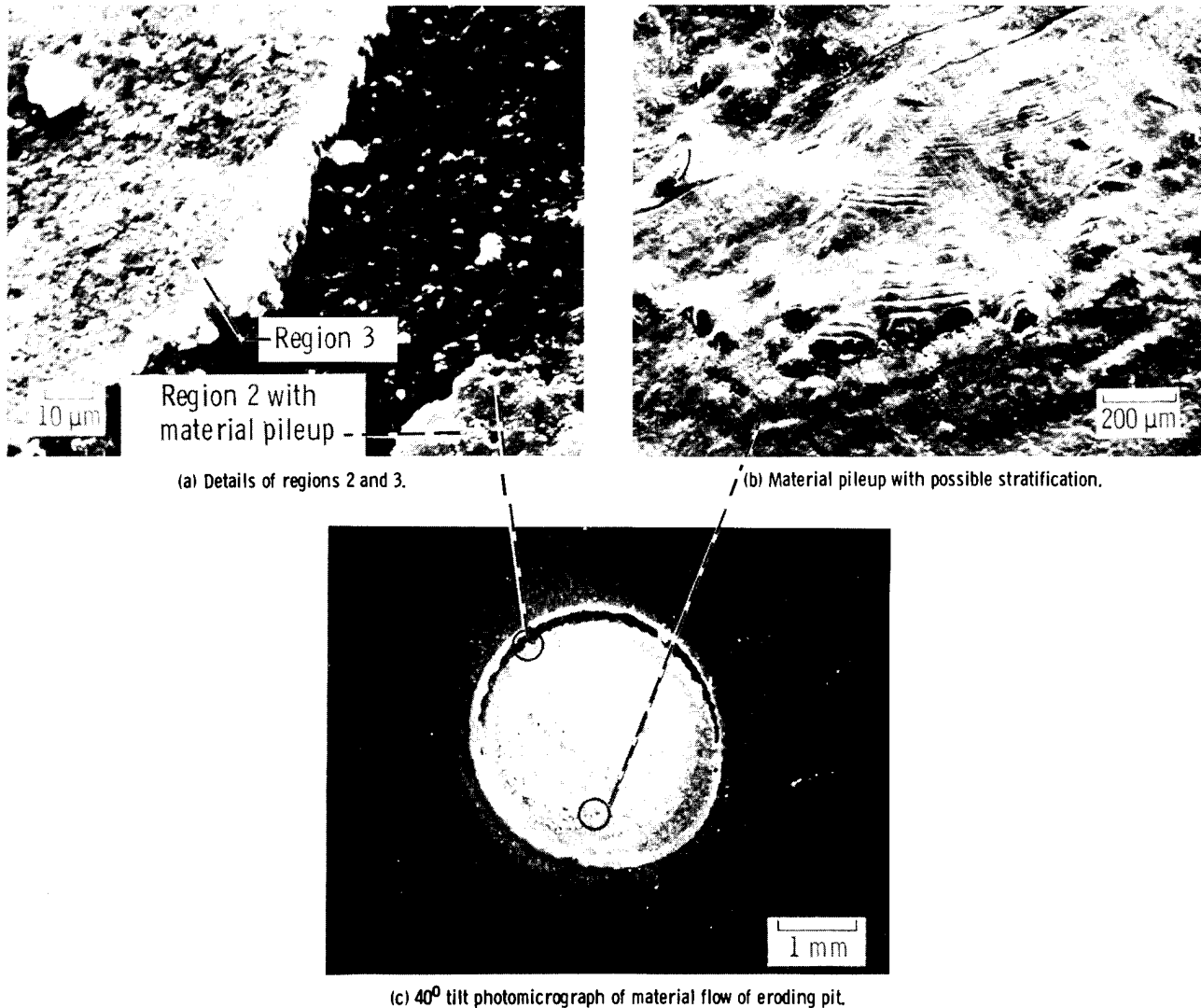
Figure 10. - SEM photomicrographs ( 40^\circ tilt) of PMMA specimen exposed to glass beads for 15 seconds at 0.27-megapascal gas pressure.
