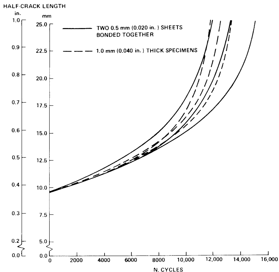
Figure 39. Crack Growth Behavior of Flat 2024-T3 Sheet 92.3 \pm 55.8 kPa ( 13,400 \pm 8,100 psi) (without coolant tubes or crack arrestors)
