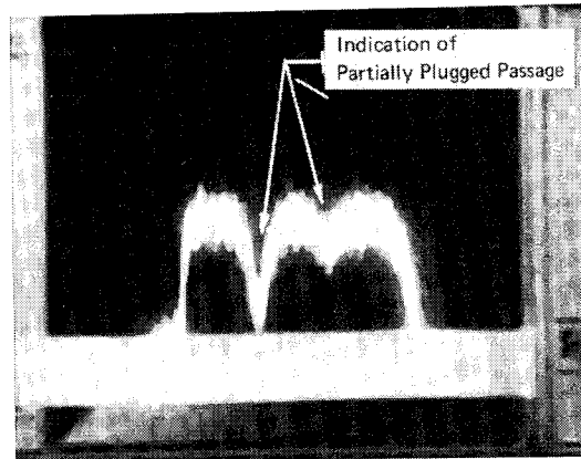
FLOW TO INBOARD MANIFOLD
