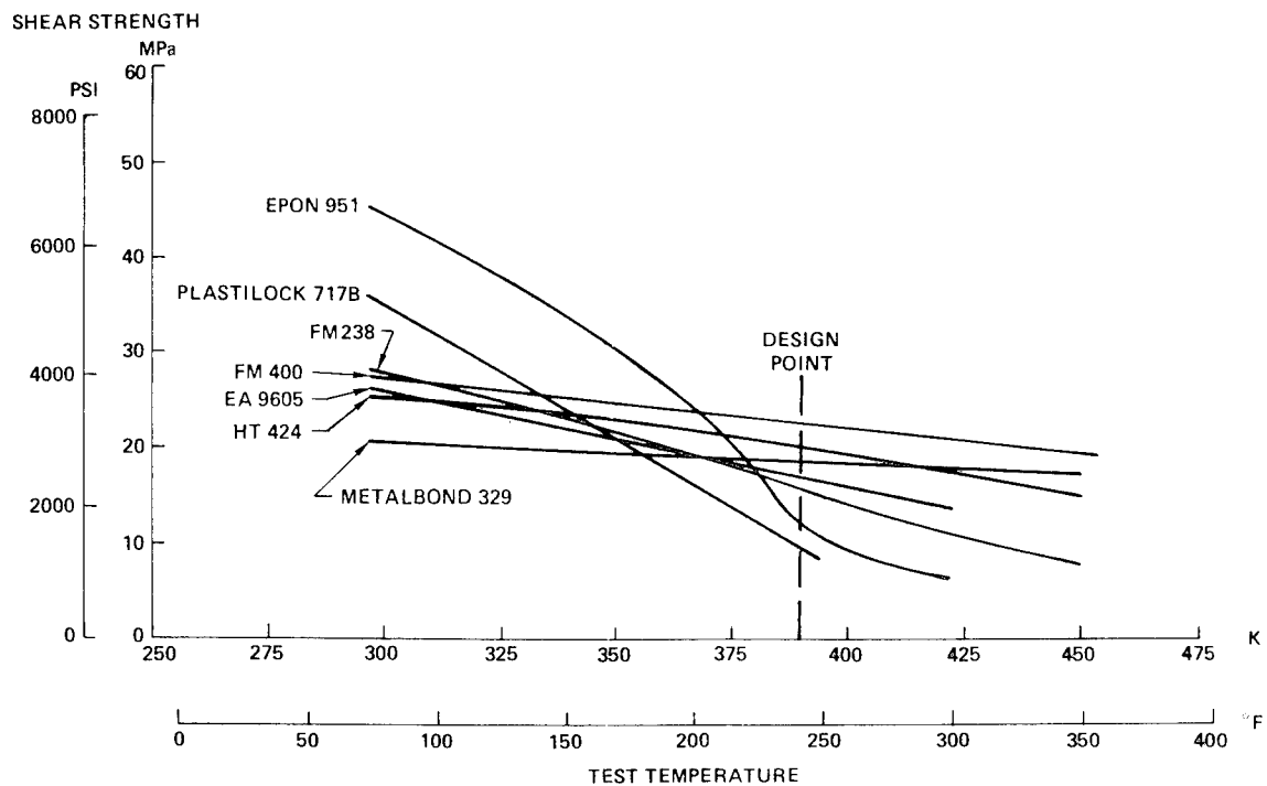
Figure 25. Tensile Lap Shear Strength of Various Adhesives
