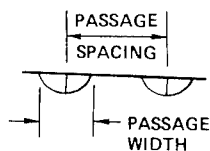
Figure 6. Maximum Panel Temperature Increases with Passage Spacing
