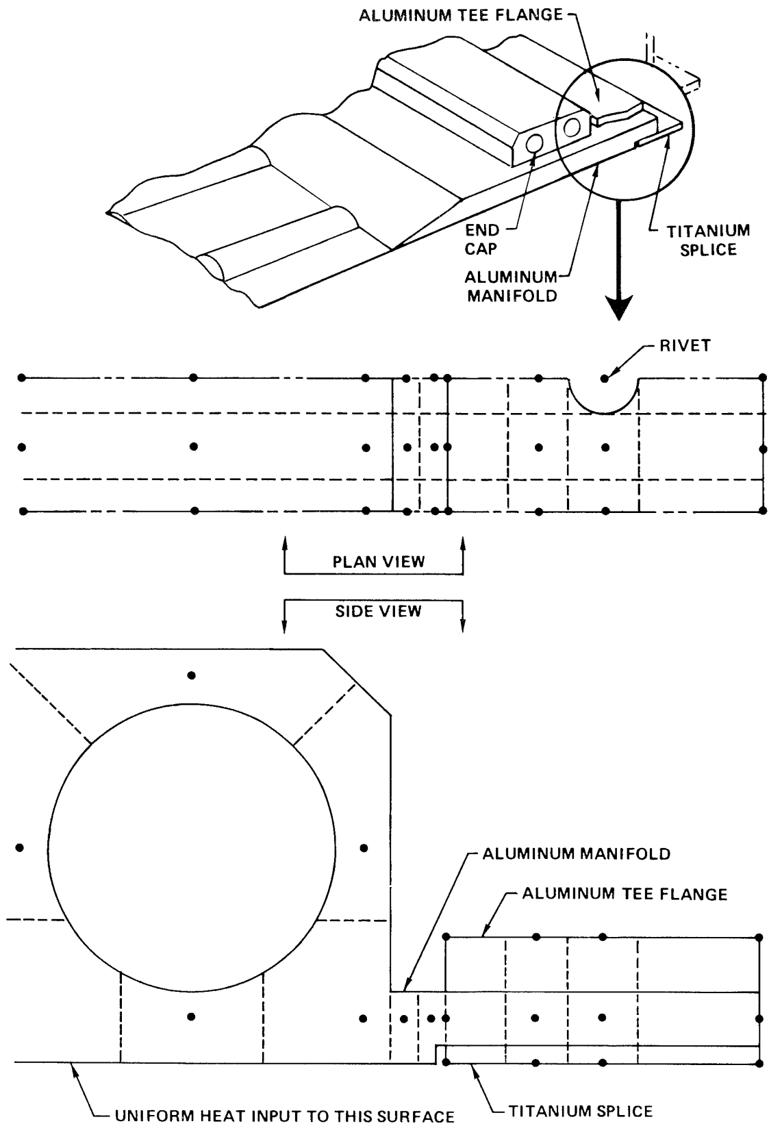
Figure 28. Manifold/Splice Thermal Model
