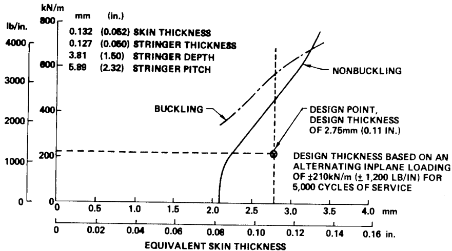
Figure 11. Panel Stability Characteristics
