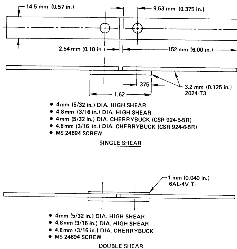
Figure 36. Joint Fatigue Test Specimens
