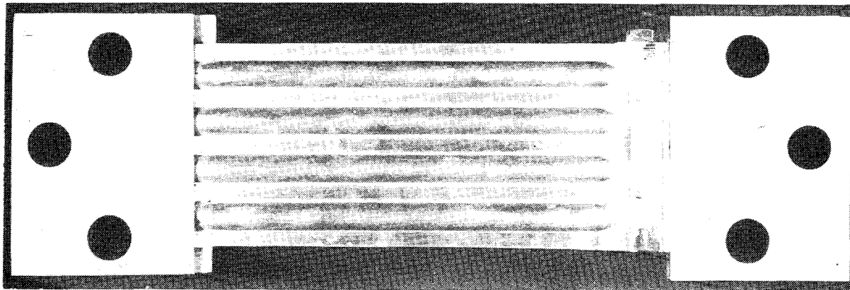
b. COOLANT PASSAGE/RAMP
