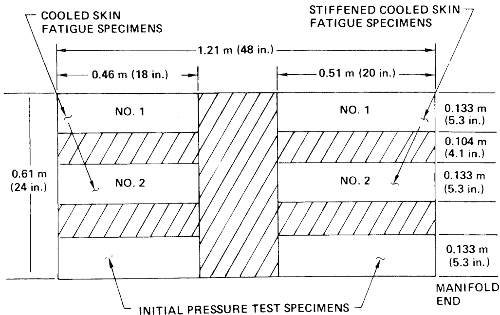
Figure 33. Fatigue and Pressure Test Specimens Were Cut From a Cooled Skin Panel
