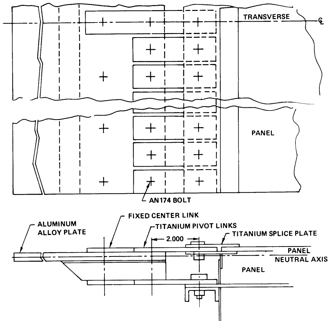
Figure 24. Load Adapter
