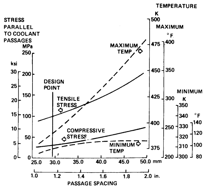
Figure 10. Temperature and Stress Trends
