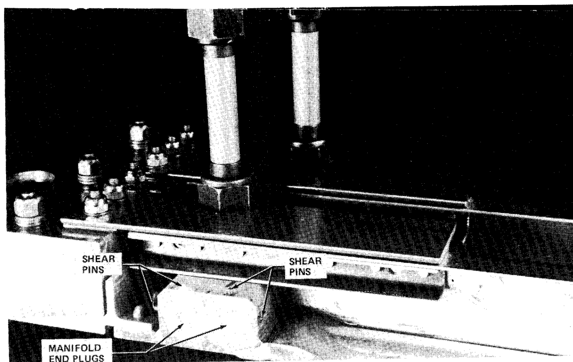
SPLICE/MANIFOLD END
