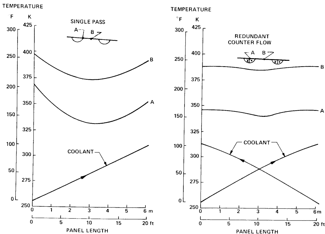
Figure 5. Counterflow of Coolant Minimizes Axial Temperature Differences
