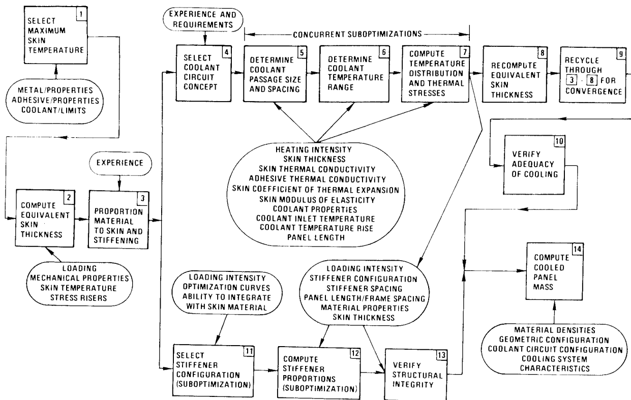
Figure 3. Repetition of Design Process Relates Skin Temperature and Panel Mass
