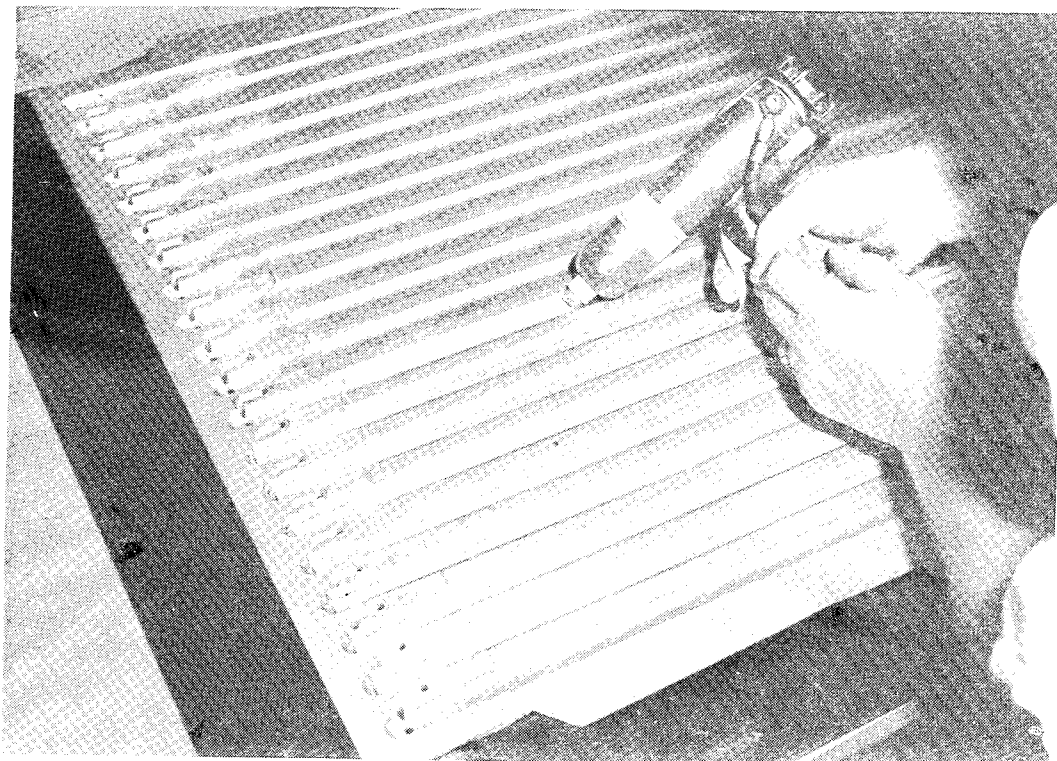
Figure 21. Application of Silver Filled Epoxy
