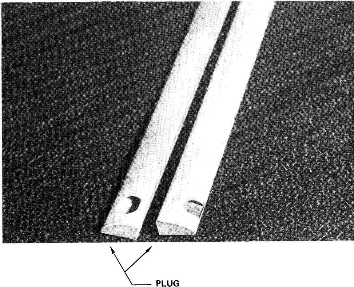
Figure 35. Coolant Passage Tube End Plug (Test Specimens Did Not Have Holes to Match Manifolding)
