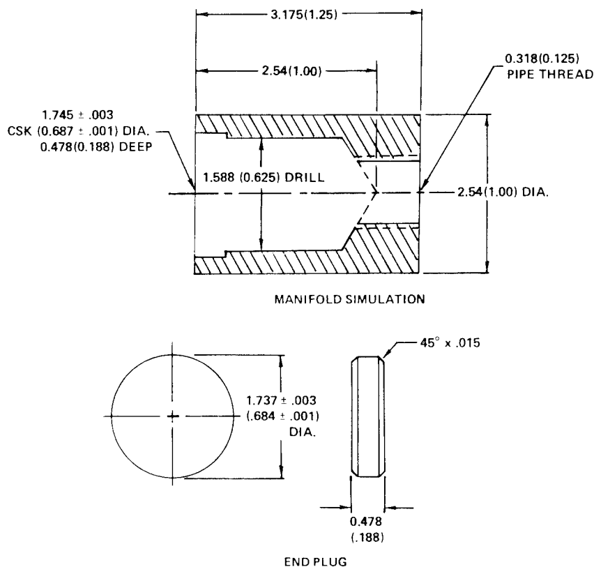
Figure 34. Manifold End Plug Test Specimen 2024-T3 Aluminum Alloy
