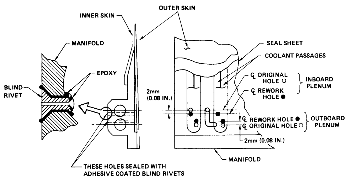
Figure 22. Rework of Plugged Interconnect Holes
