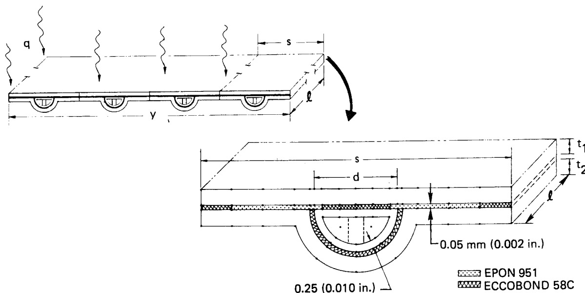
Figure 27. Panel and Discrete Passage Thermal Models
