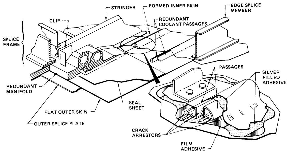
Figure 15. Details of Panel Design
