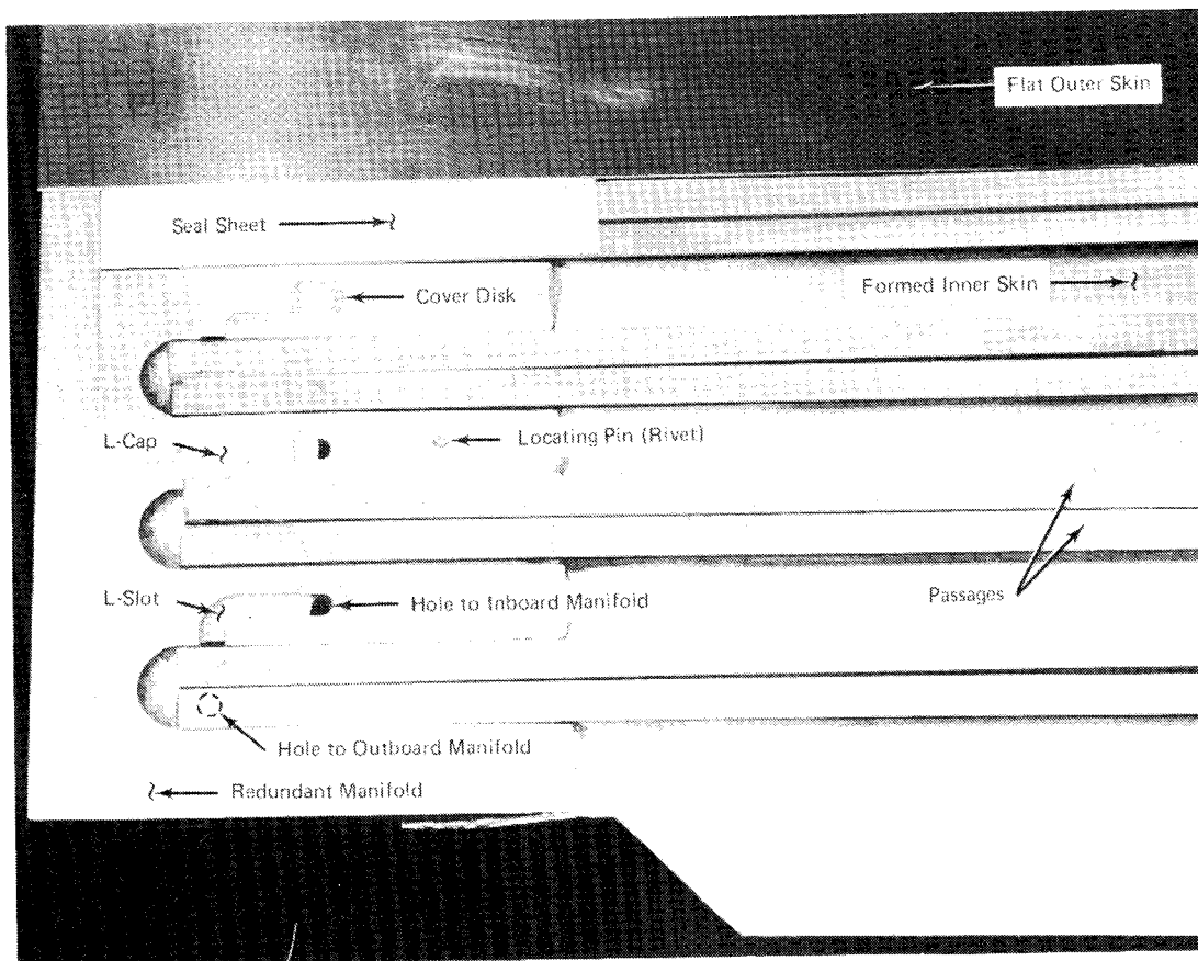
Figure 20. Tubing Installation Details
