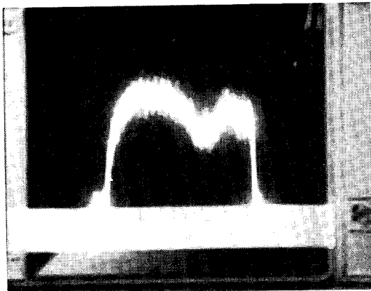
FLOW TO OUTBOARD MANIFOLD
