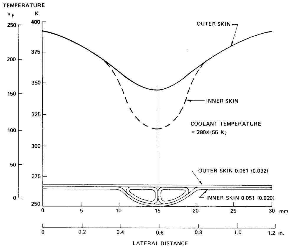
Figure 16. Temperature Distribution at Mid-Length (Stiffener not Included)
