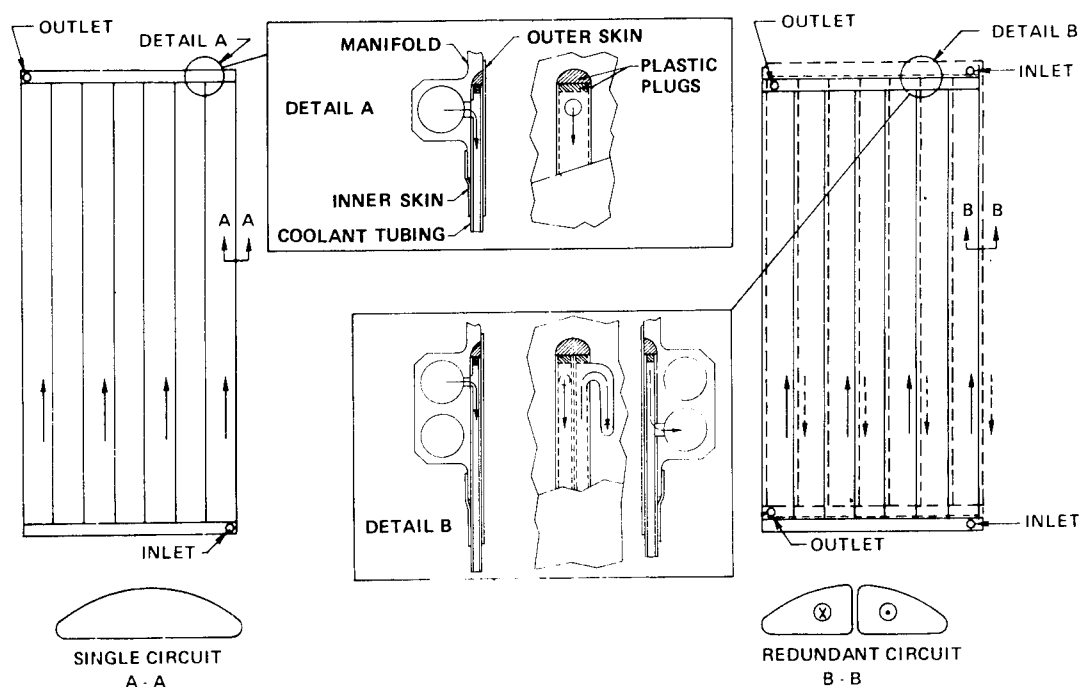
Figure 4. Two Coolant Circuits Were Compared
