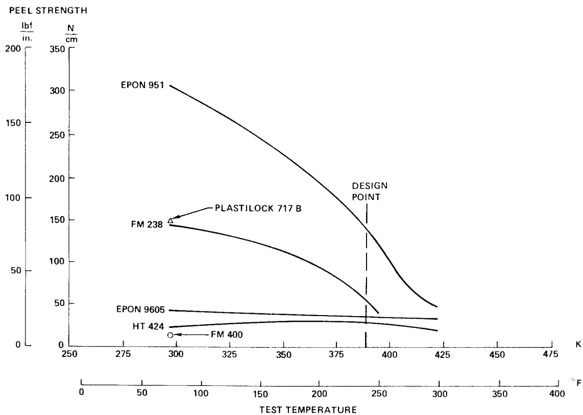
Figure 26. Peel Strength of Various Adhesives
