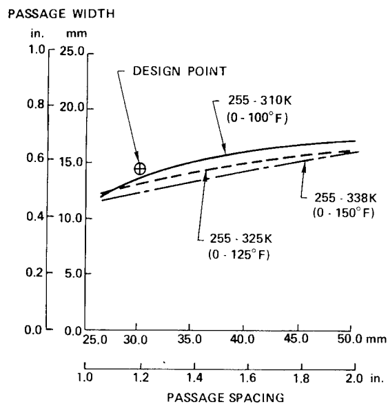
Figure 7. Optimum Passage Width Increases with Passage Spacing
