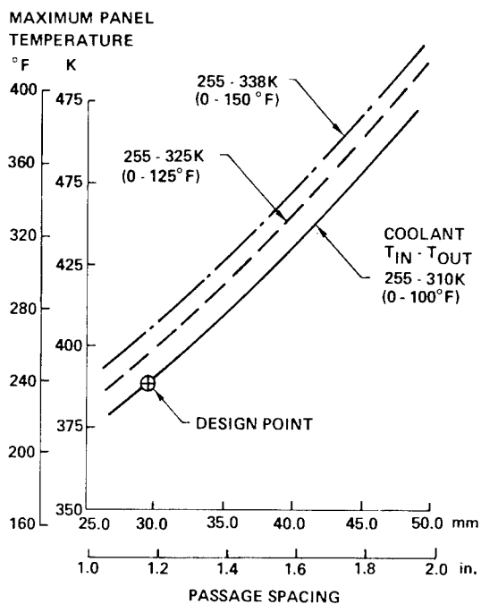
Figure 6. Maximum Panel Temperature Increases with Passage Spacing
