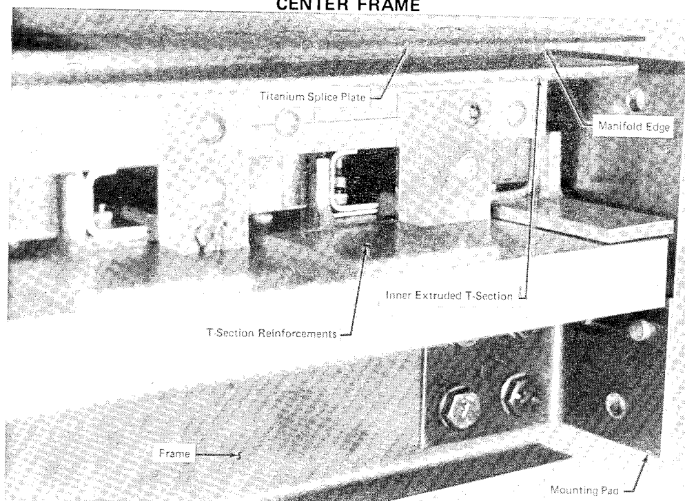
Figure 19. Test Panel Details
