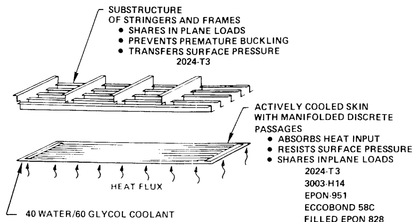
Figure 1. Actively Cooled Structural Panel
