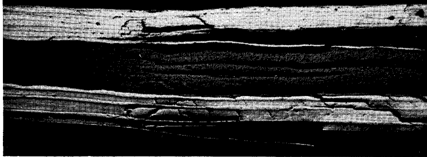
(a) MAGNIFICATION 8X 16 S-GLASS PLYS PLACED IN THE MIDDLE WITH 8 PLYS OF GRAPHITE COVERING
