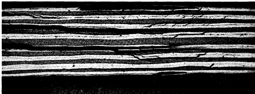
(b) MAGNIFICATION 8X S-GLASS AND GRAPHITE PLYS ALTERNATELY PLACED
