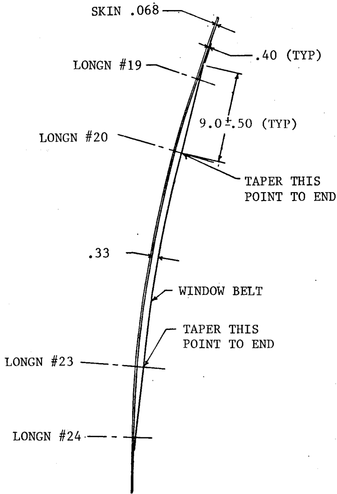
WINDOW BELT REINFORCEMENT
