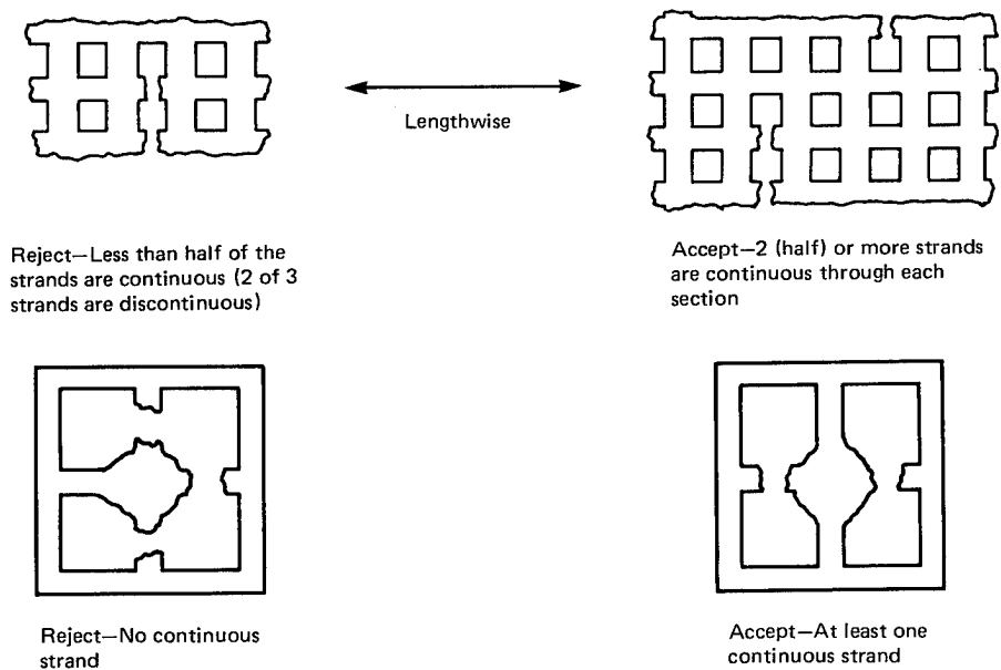
Figure 69. Visual criteria for mesh bonds.
