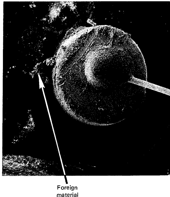
Figure 73. Attached foreign material next to a bonding post. Note the unacceptable rework attachment of a wire by adhesive.
