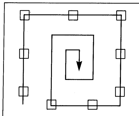
Figure 74. Sample pattern for inspecting a die.
