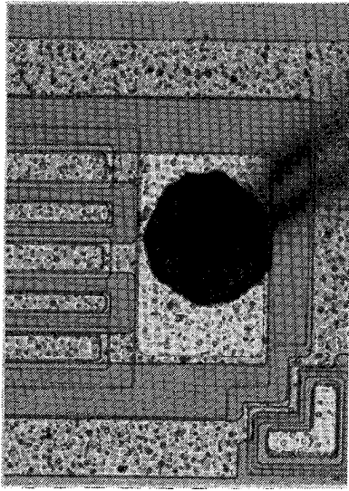
(a) Acceptable intermetallic growth (<1 mil)
