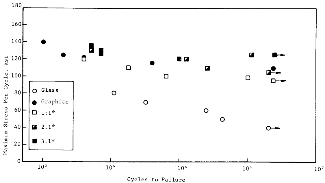
Figure 21b Comparison of the Fatigue S-N Behavior of Unidirectional T300 Graphite/S-Glass/Narmco 5208 Hybrid Composites after Conditioning at 98% RH and 120°F for 1000 Hours. *Ratio of Graphite to Glass
