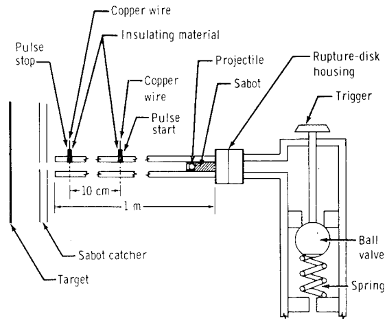
Figure 1. - Air-gun apparatus.
