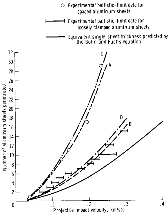
Figure 11. - Comparison of the Bohn and Fuchs equation with the experimental ballistic-limit data for a layered target made up of aluminum sheets. The target was impacted by steel projectiles.
