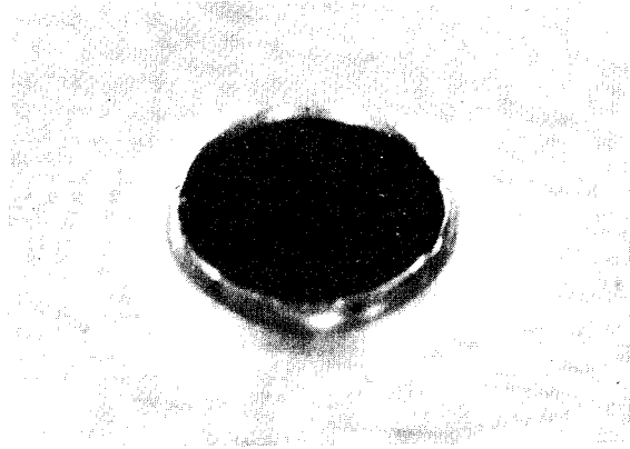
(a) Single layer perforated by a steel projectile with an impact velocity of 0.300 km/sec.
