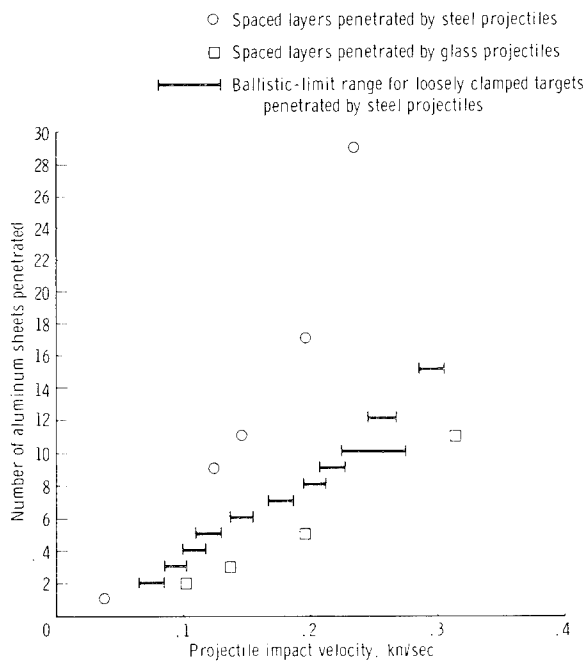
Figure 2. - Penetration of aluminum sheets by glass and steel projectiles.
