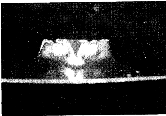
(b) Single layer perforated by a glass projectile with an impact velocity of 0.185 km/sec.
