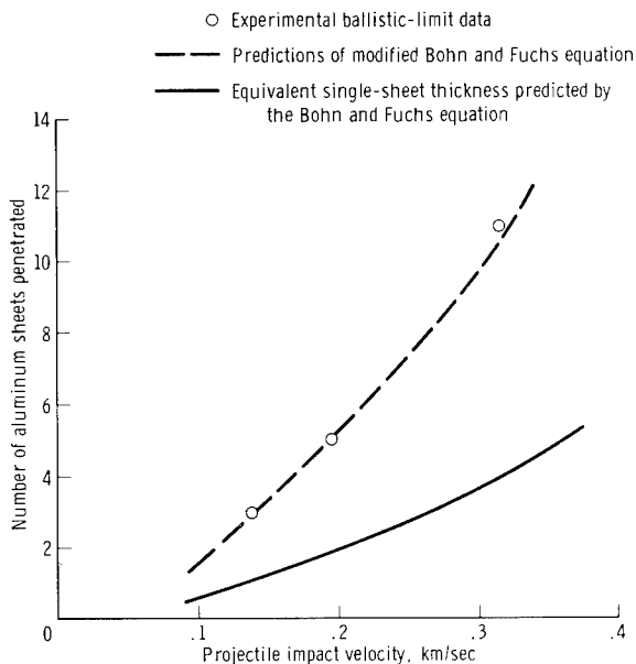
Figure 9. - Comparison of the predictions of the Bohn and Fuchs equation and the modified Bohn and Fuchs equation with experimental ballistic-limit data for glass projectiles impacting a layered target made up of aluminum sheets separated by 4.76 millimeters (three-sixteenths inch).
