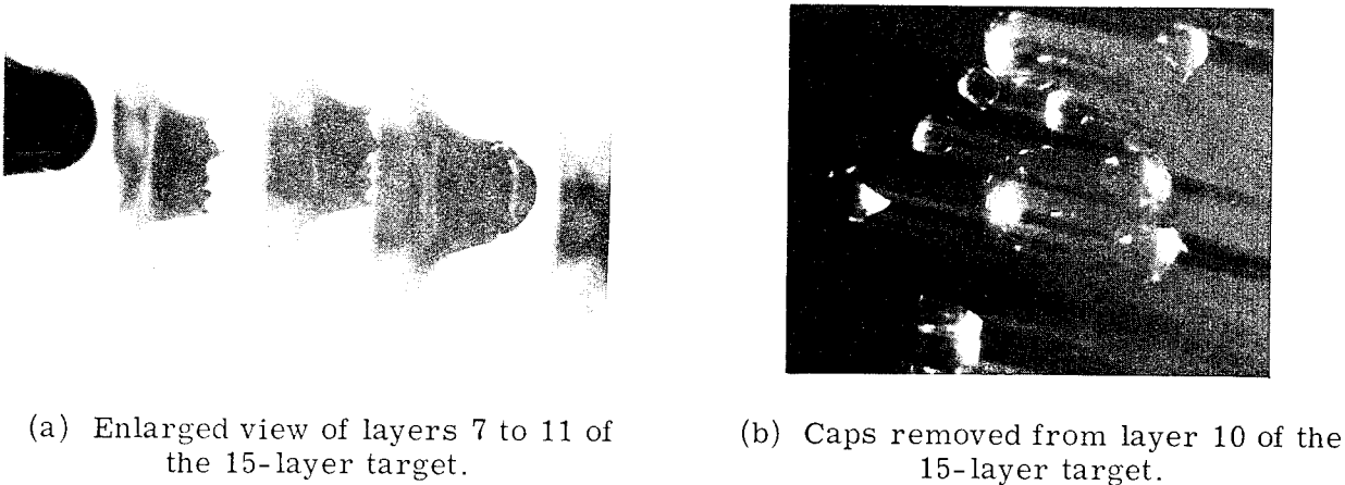
Figure 7. - Enlarged view of layers 7 to 11 of the 15-layer target and the caps removed from layer 10.
