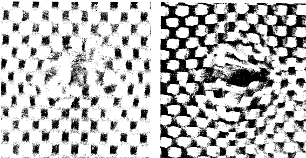
(a) First layer impacted; area density, 0.1791\text{ kg/m}^2 ( 6.04\text{ oz/yd}^2 ).
