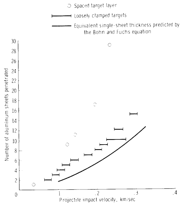
Figure 10. - Ballistic-limit data for a layered target made up of aluminum sheets. The target was impacted by steel projectiles.
