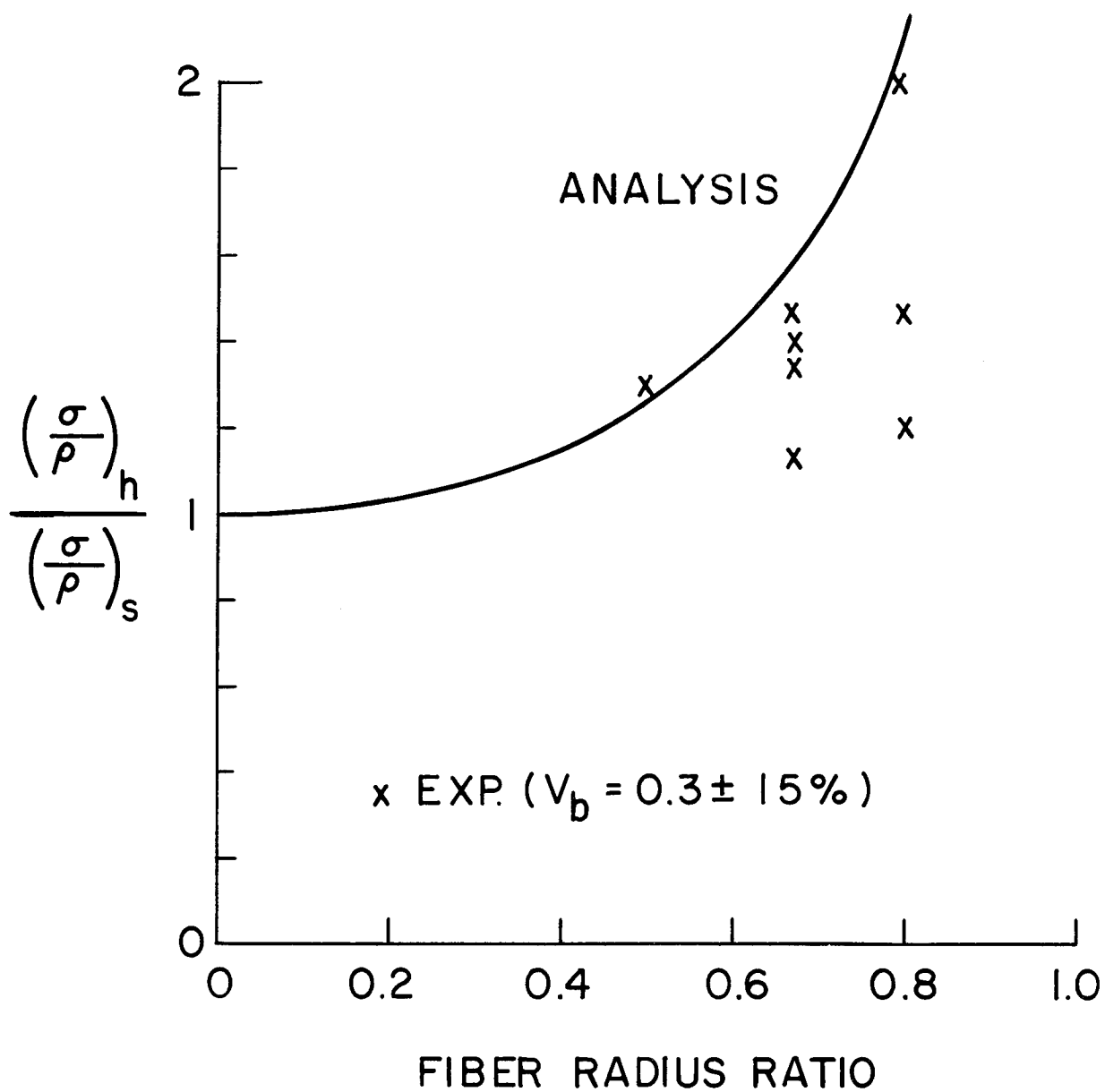
Figure 23. Comparison of Theory and Experiment for Compressive Strength to Density Ratio of Hollow Glass Fiber Composites.
