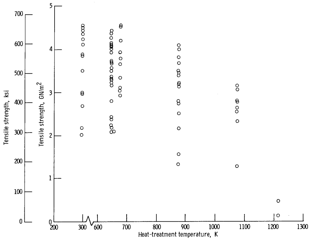
Figure 8. - Tensile strength of B/W fibers at 295 K as function of heat-treatment temperature. Heat treatment in vacuum of \approx 10^{-6} newton per square meter for 1.5 hours; fiber diameter, 203 micrometers (7.98 mils).
