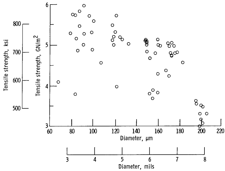
Figure 7. - Tensile strength as function of B/W fiber diameter after retrieval from aluminum matrix and etching in hot 2\text{HNO}_3 + 1\text{H}_2\text{O} . Diameter prior to etching, 203 micrometers (7.98 mils).
