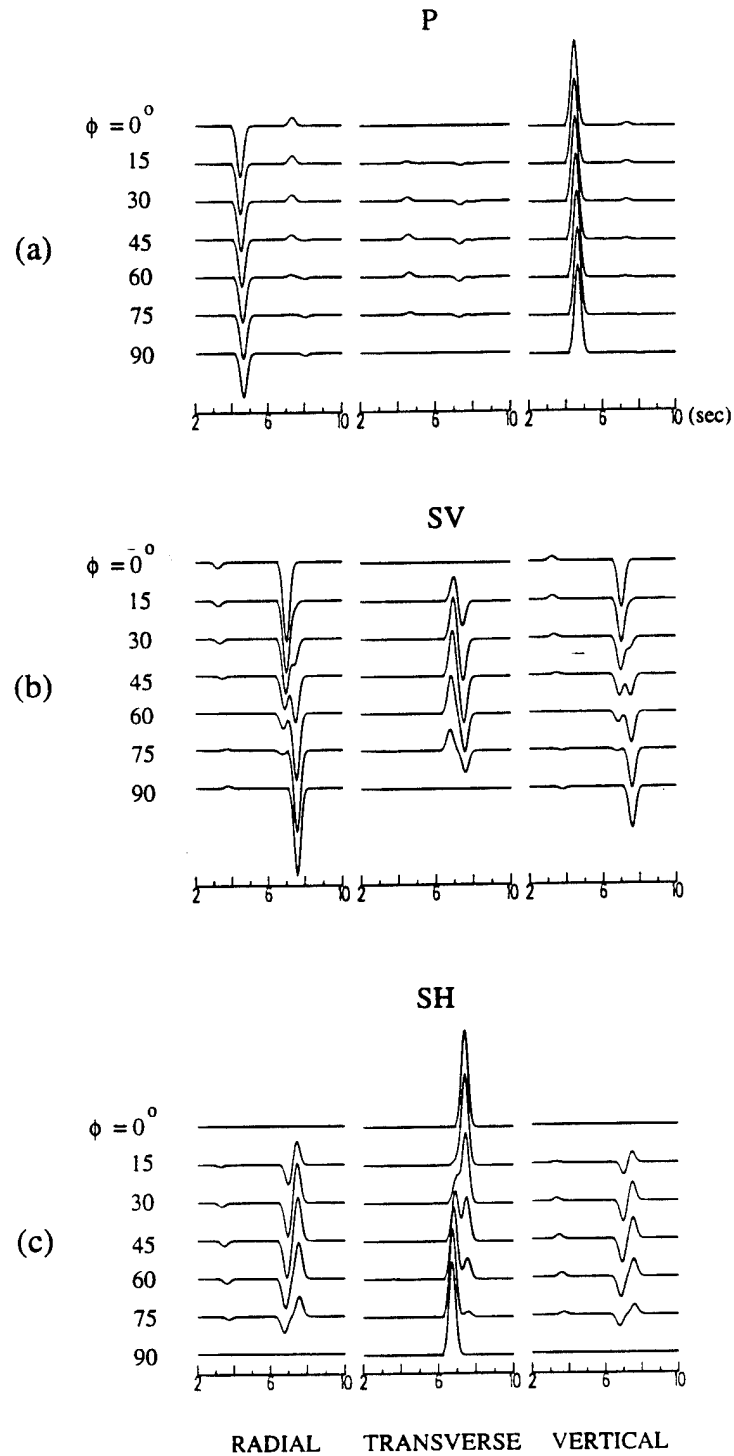
Figure 4. Displacements of the free surface produced by (a) P, (b) SV, (c) SH at 25° angle of incidence on transversely isotropic layer in Model 1 of Table 1. \phi is angle between the axis of symmetry of the transversely isotropic layer and the horizontal projection of the wave propagation direction. The input pulse used here is given by figure 1(a).
