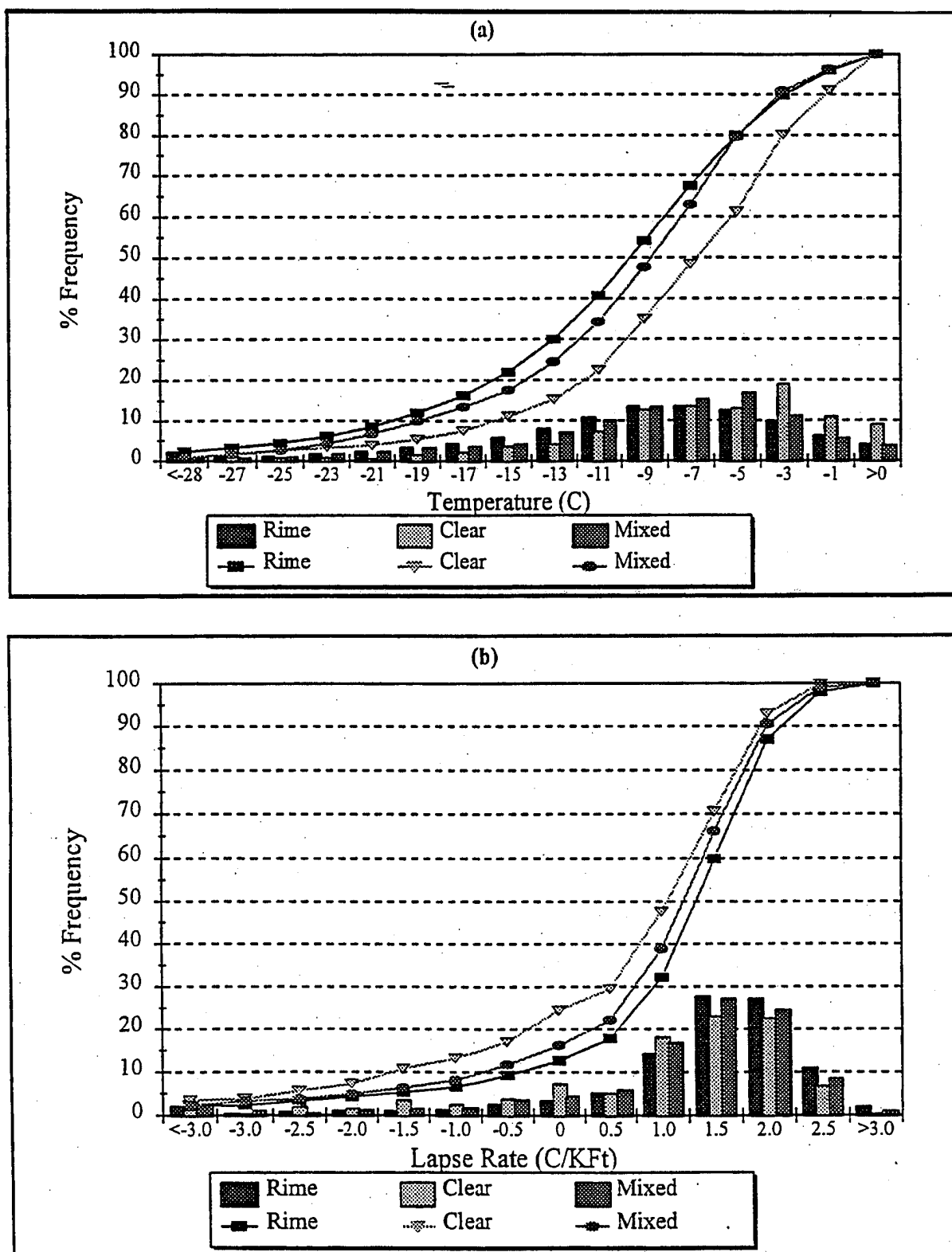
Figure 1. Percent and cumulative percent frequency of occurrence of icing type as a function of (a) temperature and (b) lapse rate. The temperature data is binned in 2 degree intervals, the lapse rate data in 0.5 degree intervals.
