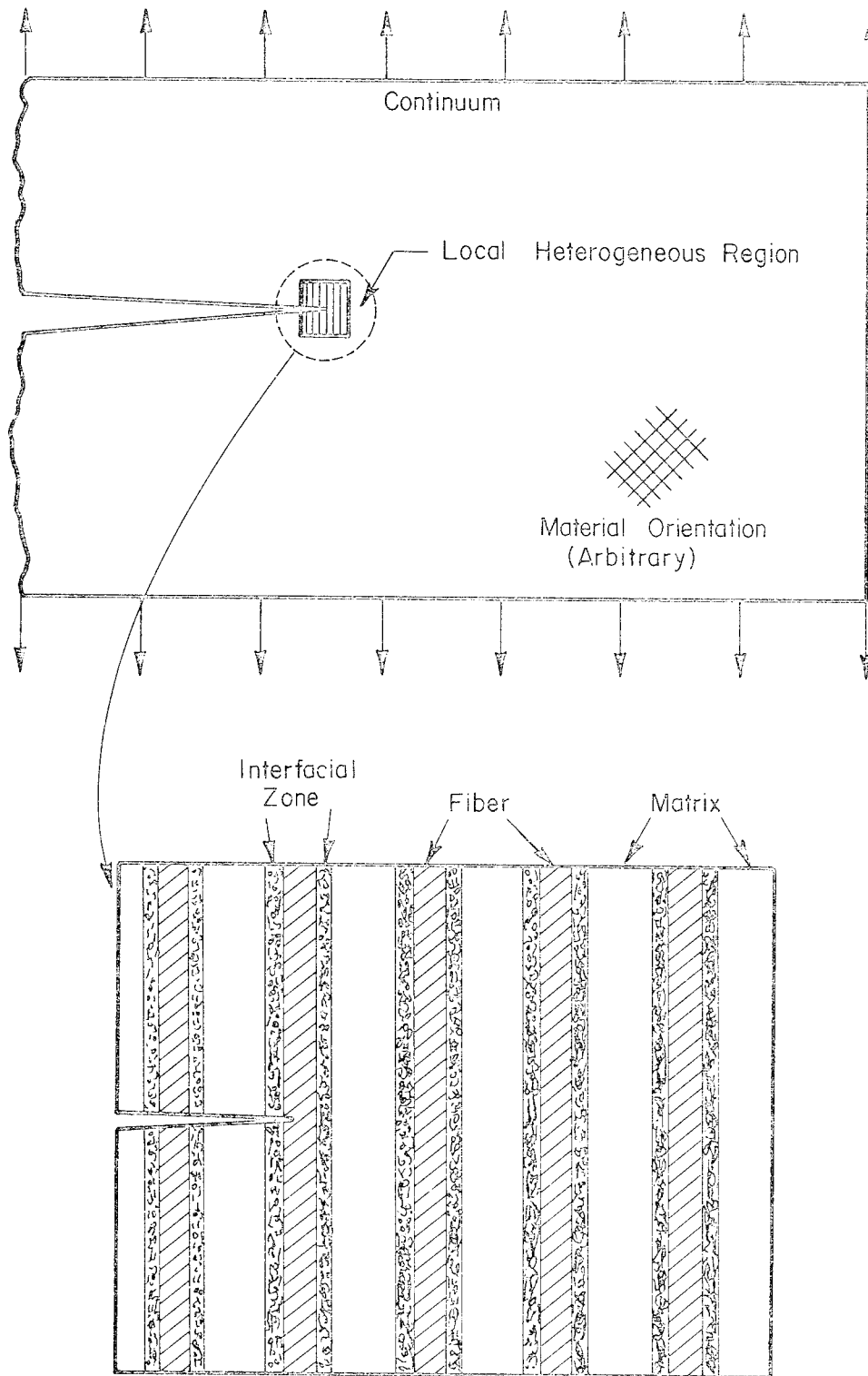
FIGURE 1. THE LHR CONCEPT
