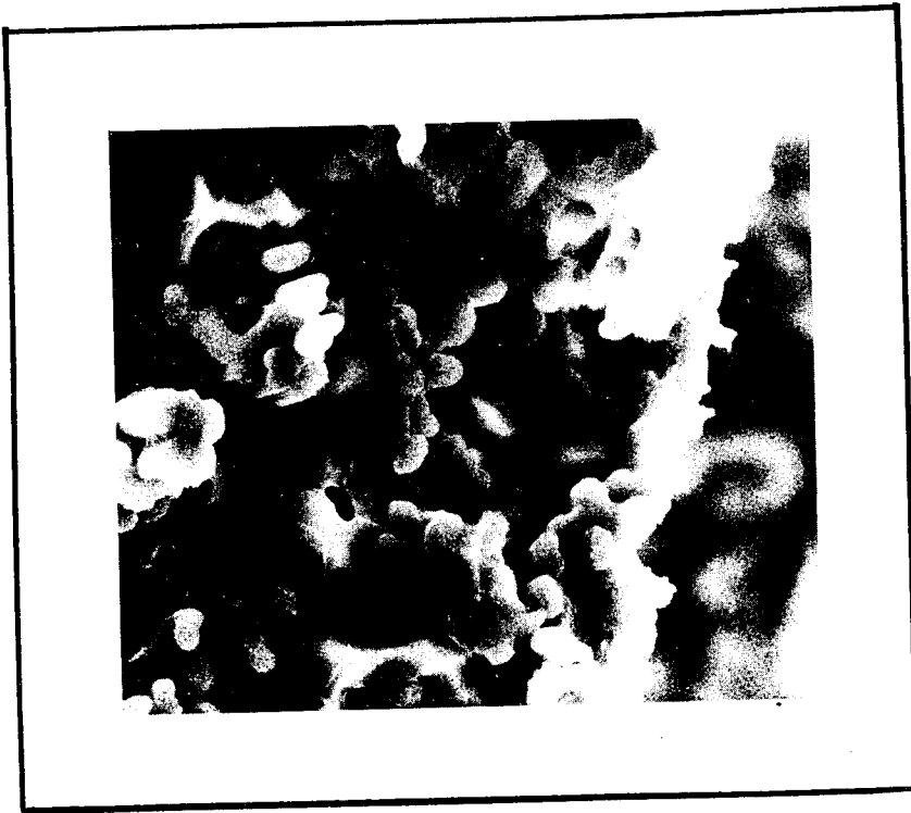
Figure 16. Fracture Surface of Unidirectional Sample 100 Cycles 1000X
