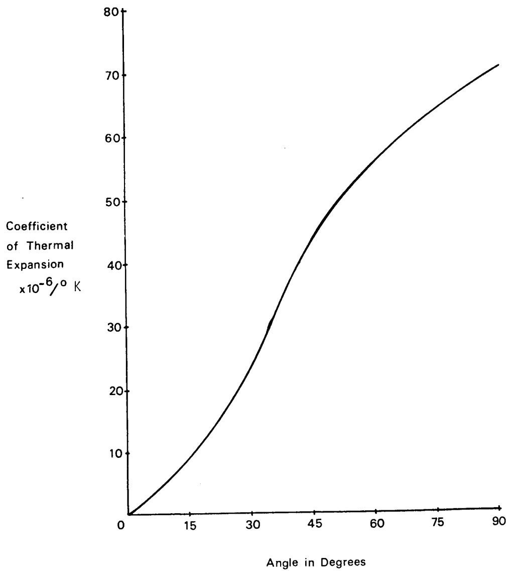
Figure 15. Thermal Expansion vs Angle from Fiber Direction in Unidirectional Sample
