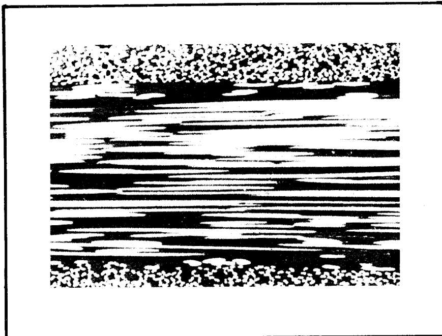
Figure 9. Uncycled [[+45_3]_2]_T Sample, 300X
