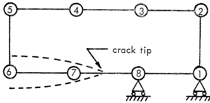
(a) 8-node Symmetric Cracked Element
