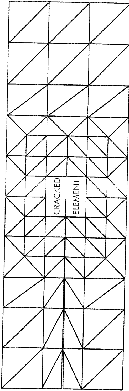
DETAIL MODEL
