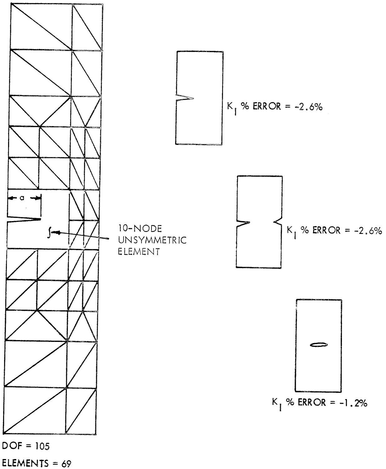
FIGURE 13. UNSYMMETRIC CRACKED ELEMENT MODEL FOR SINGLE-EDGE, DOUBLE-EDGE, AND CENTER CRACKED TENSION PANELS ( \sigma/w = 1/3 )
