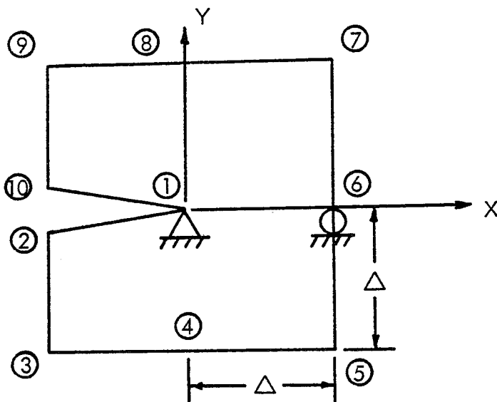
FIGURE A-7. LOCAL COORDINATE SYSTEM FOR TEN-NODE CRACKED ELEMENT
