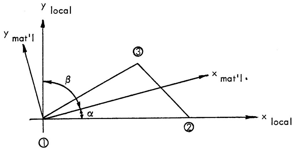
FIGURE 1. TRIANGULAR ELEMENT MATERIAL AXIS
