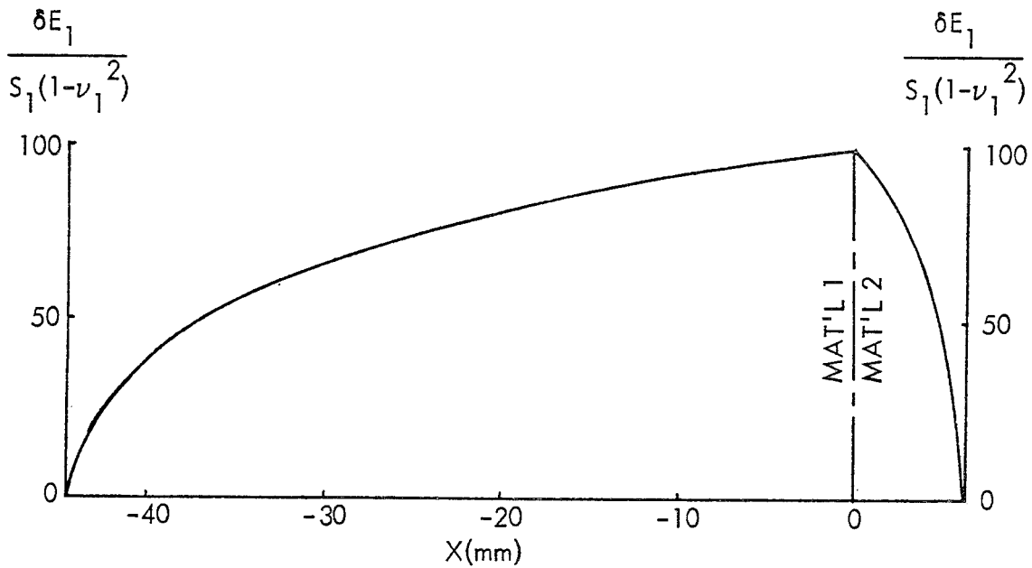
FIGURE 18. DISPLACEMENTS OF CRACKED FACES IN BI-MATERIAL PLATE
