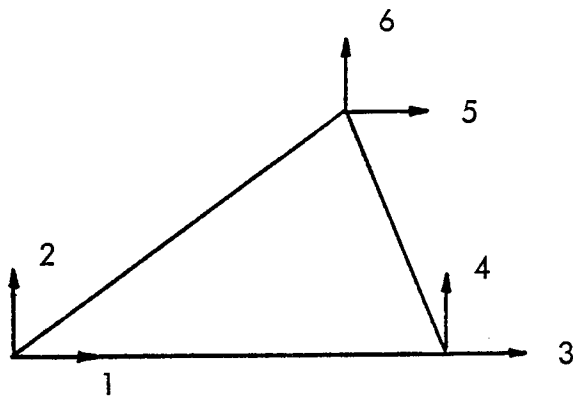
FIGURE A-3. CONVENTION FOR DEGREES OF FREEDOM
