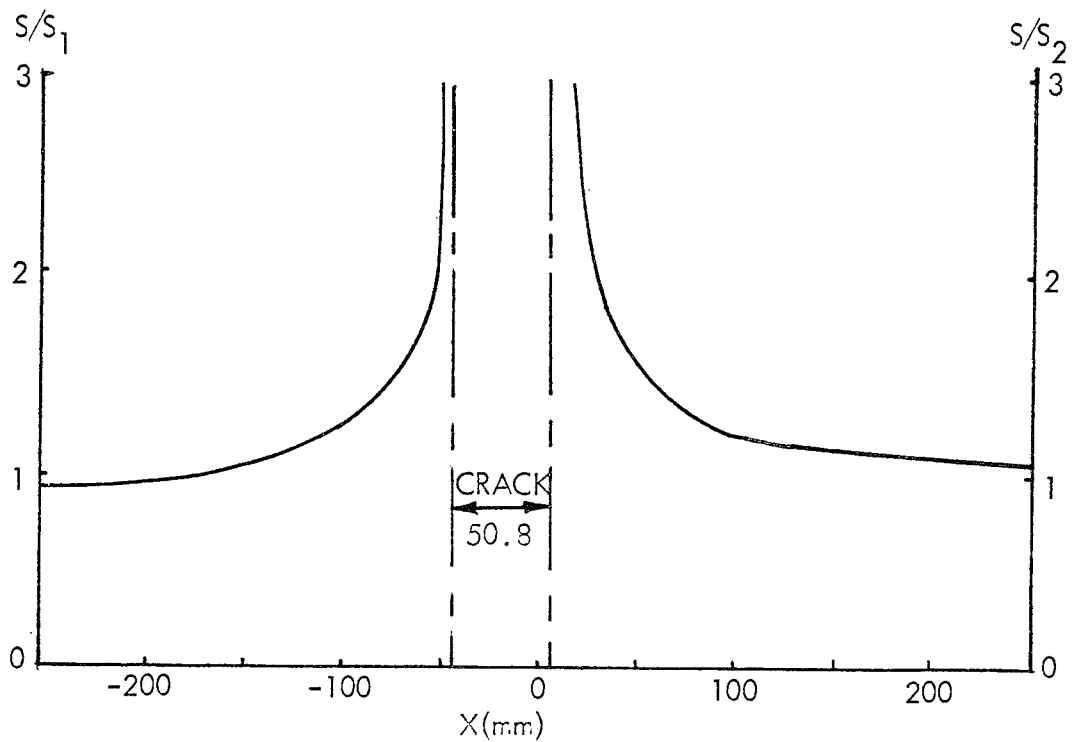
FIGURE 17. STRESS IN BI-MATERIAL CRACKED PLATE
