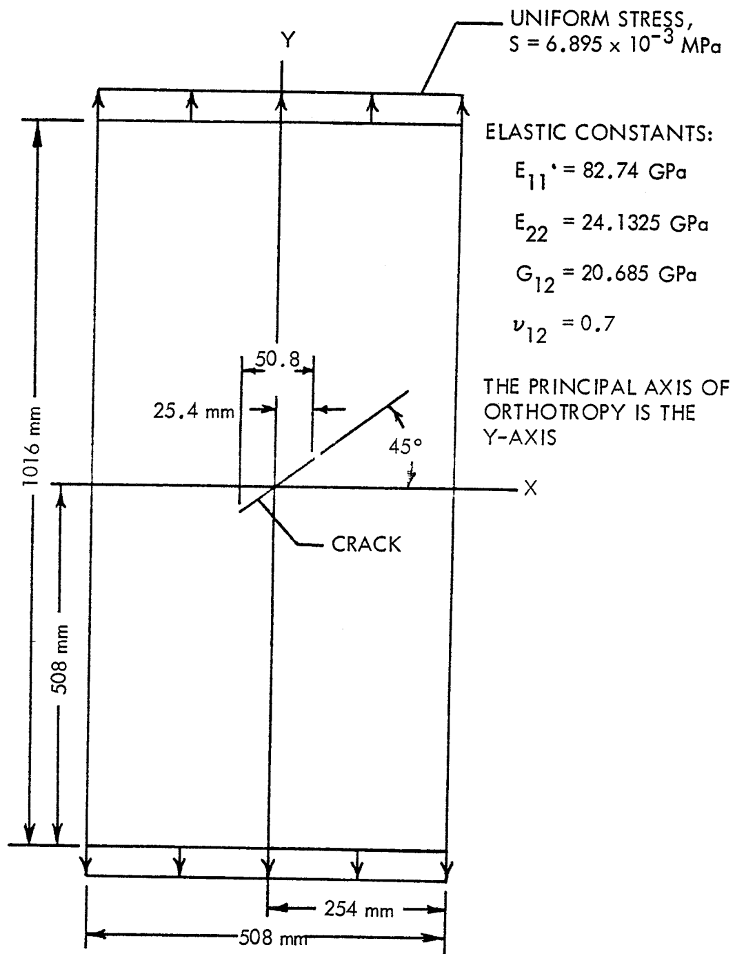
FIGURE 10. 45° CRACKED FINITE ORTHOTROPIC PLATE
