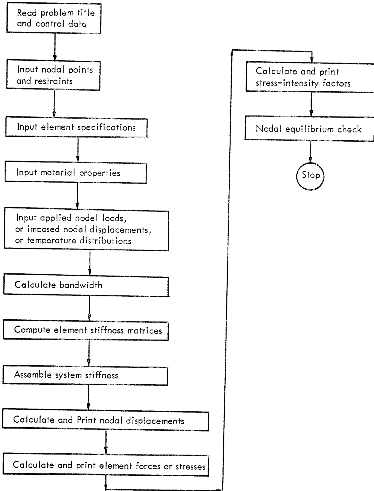
FIGURE 5. OVERALL LOGIC FLOW OF COMPUTER PROGRAM
