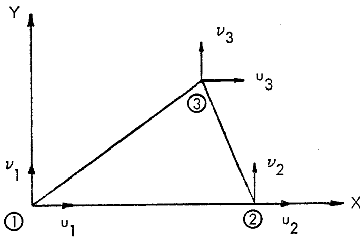
FIGURE A-2. TRIANGULAR ELEMENT MEMBRANE DISPLACEMENTS
