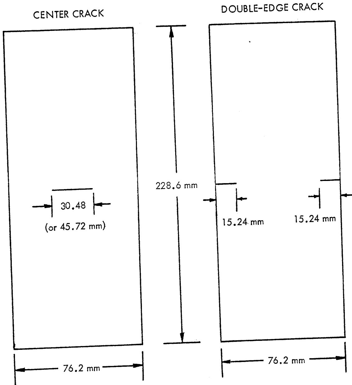
FIGURE 6. CENTER-CRACKED AND DOUBLE-EDGE-CRACKED ORTHOTROPIC TENSION PLATE
