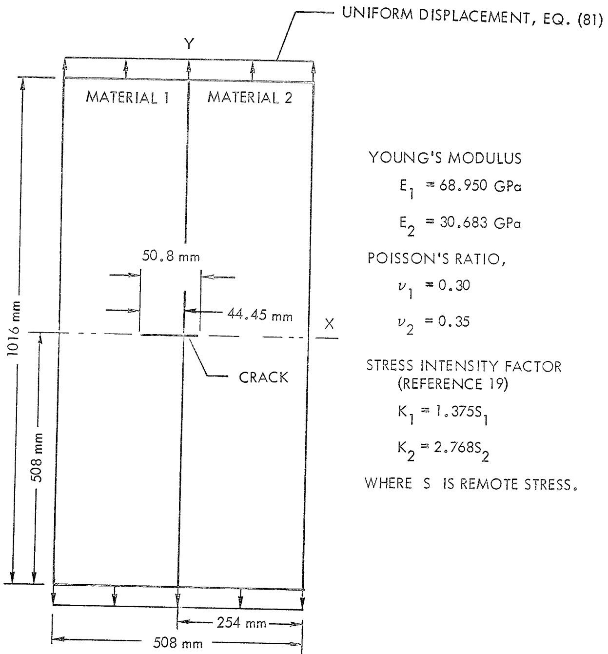
FIGURE 15. BI-MATERIAL CRACKED PLATE
