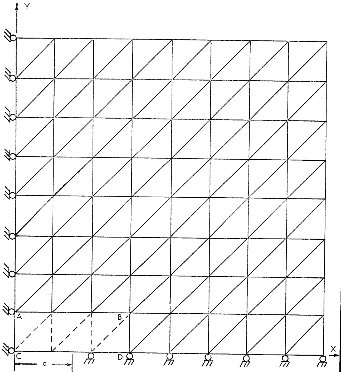
FIGURE 23. FINITE-ELEMENT REPRESENTATION OF THERMAL STRESS PROBLEM
