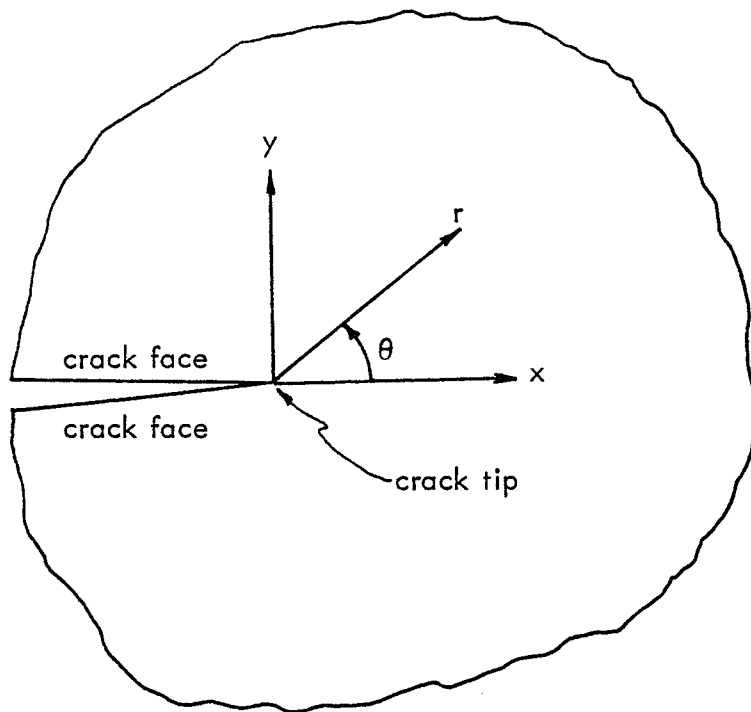
FIGURE 2. CRACK-TIP NEIGHBORHOOD
