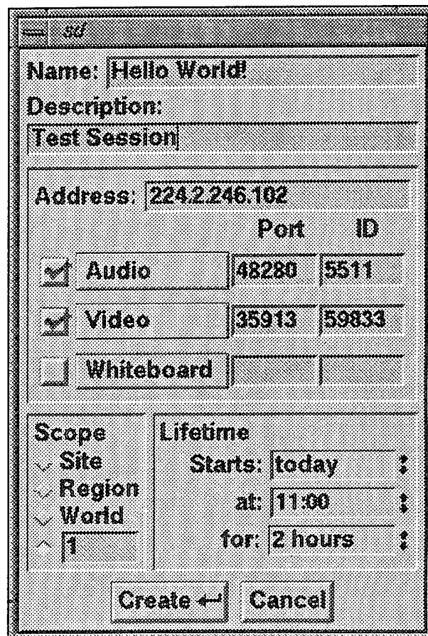
Figure 2. New Session Directory ( sd ) window
