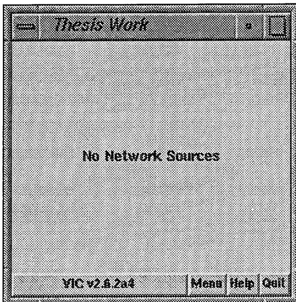
Figure 8. vic window
