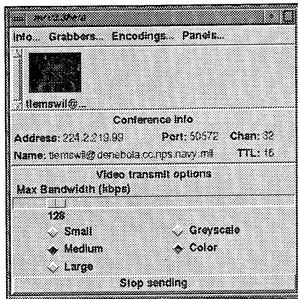
Figure 3. nv Tool
