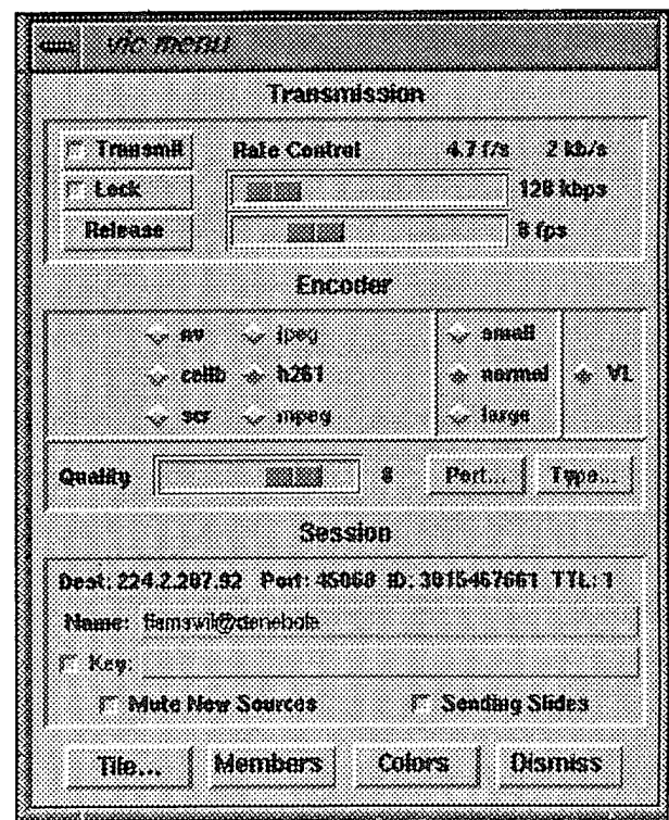
Figure 9. vic menu
