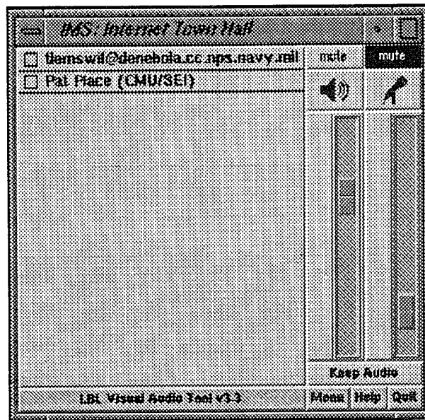
Figure 6. vat window
