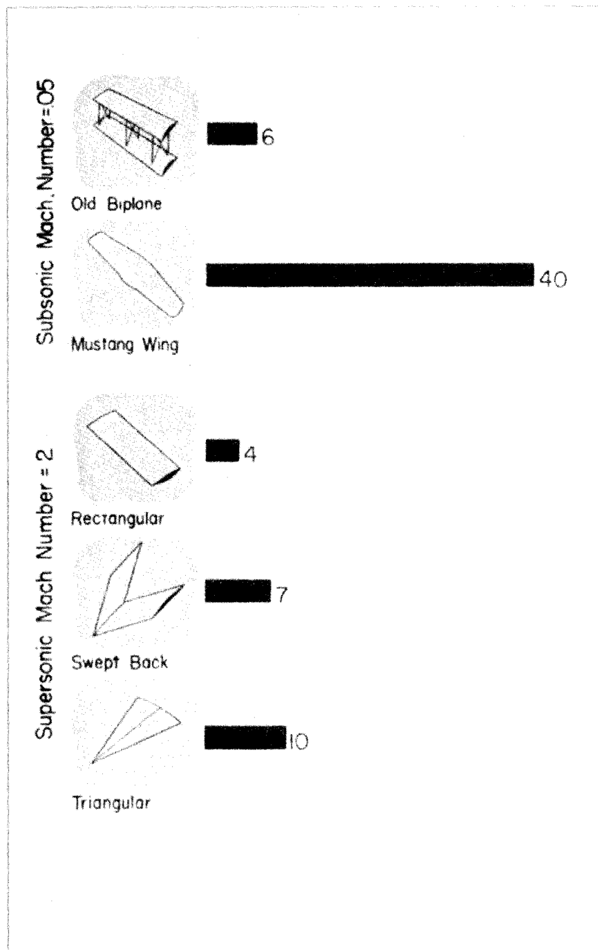
Figure 3—Optimum Lift-Drage Ratios
