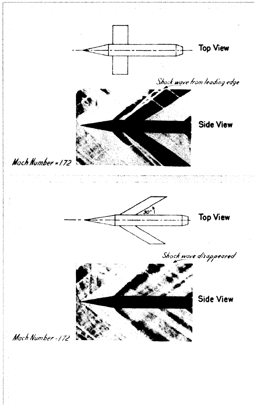
Figure 4—Sweepback Effect on Shock Waves
