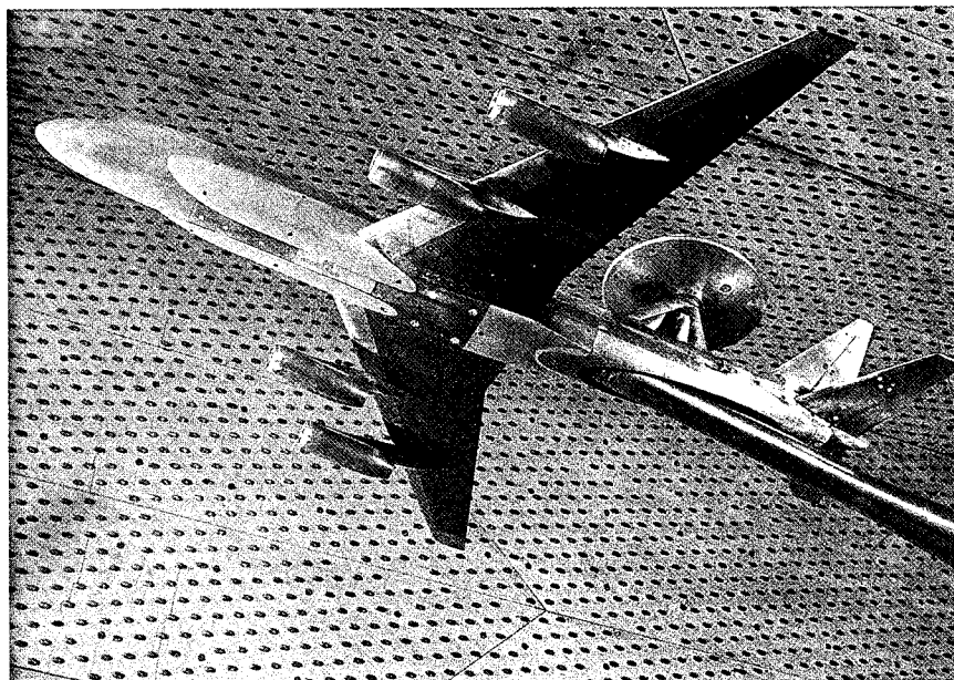
Developing wind tunnels and testing aircraft design models was important to Kármán's vision of aircraft development and testing methods. Above is an E-3A Airborne Warning and Control (AWAC) model undergoing wind tests at the Arnold Engineering and Development Center (AEDC), Tullahoma, Tennessee.
