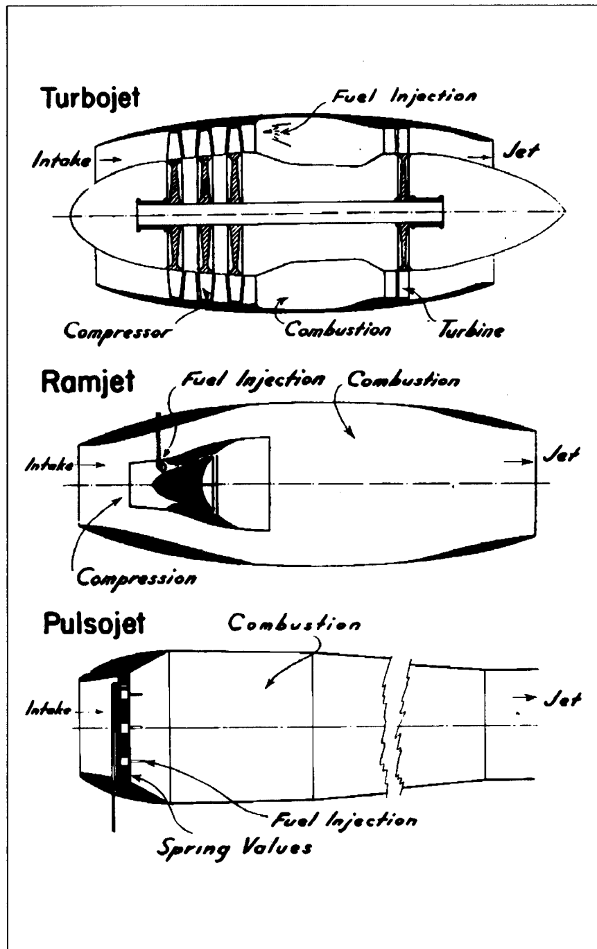
Figure 10-B—Various Propulsion Systems
