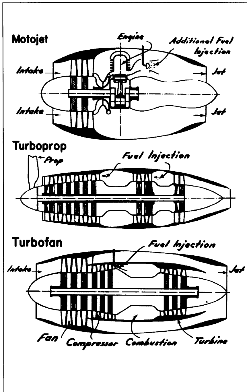
Figure 10-A-Variety Propulsion Systems
