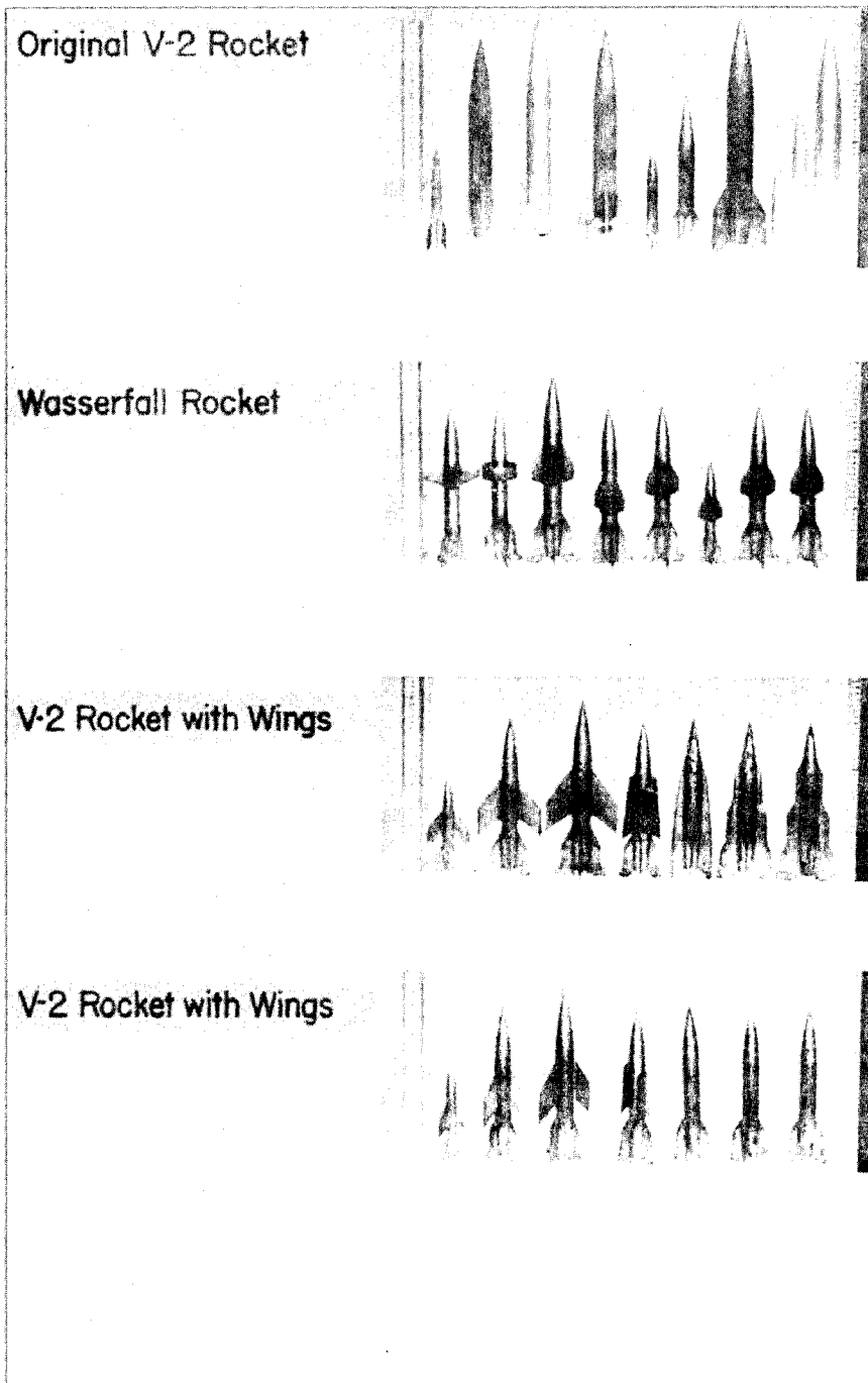
Figure 7—Rocket Models for Supersonic Wind-Tunnel Tests
