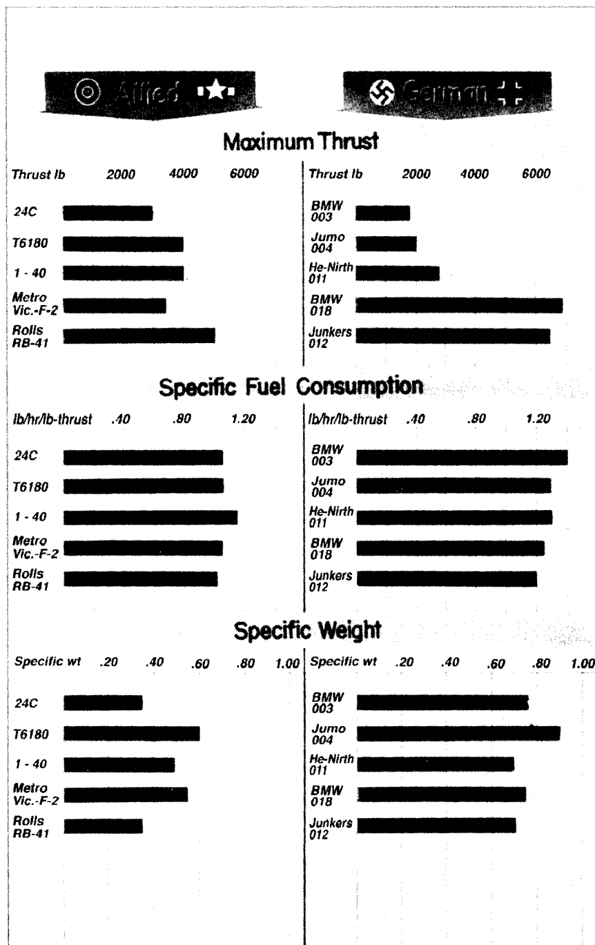
Figure 13—Characteristics of Turbojets
