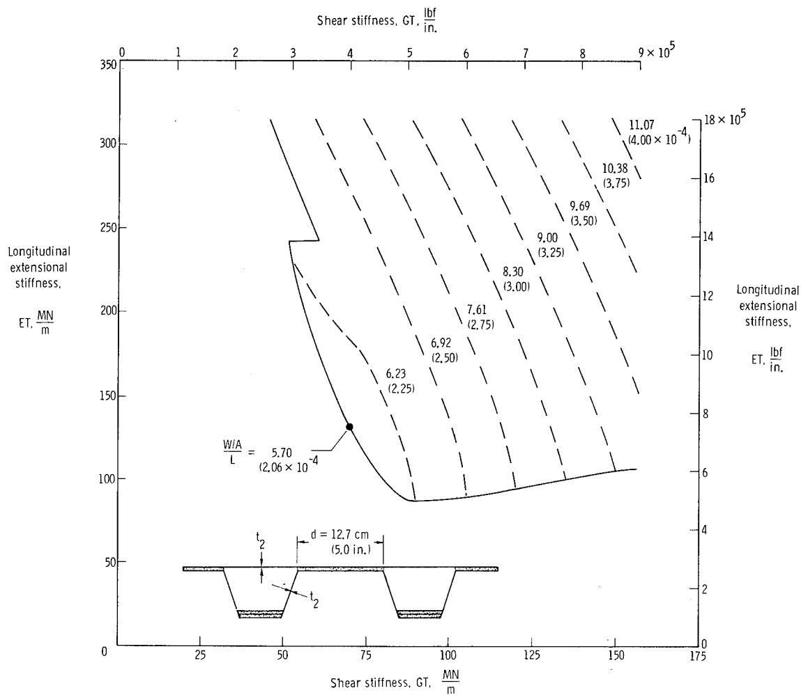
Figure 16.- Panel structural efficiency as function of longitudinal-extensional-stiffness and shear-stiffness requirements for minimum-mass, hat-stiffened, graphite-epoxy compression panels designed to support loading of \frac{N_x}{L} = 689 \text{ kPa (100 lbf/in}^2\text{)} . Thickness t_2 varies continuously. Mass index \frac{W/A}{L} given in \text{kg/m}^3 ( \text{lbm/in}^3 ).
