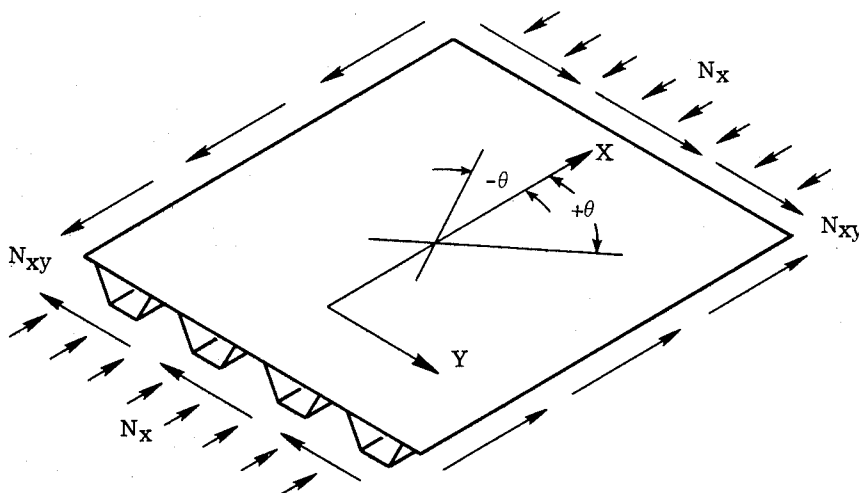
Figure 1.- Loadings considered.
