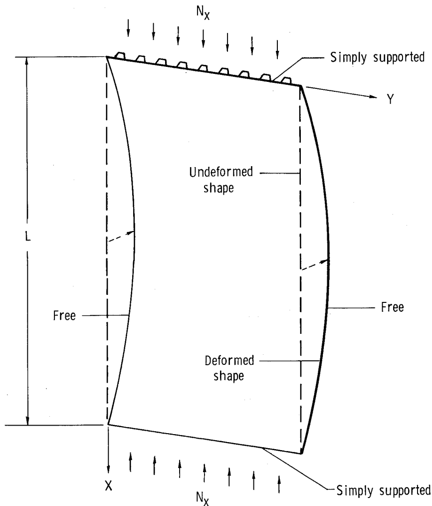
Figure 4.- Wide-column or Euler buckling is assumed for overall buckling in axial compression.
