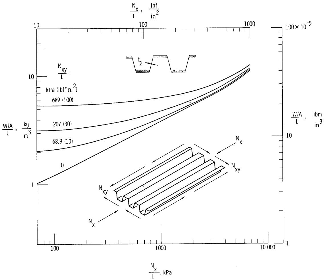
Figure 20.- Effect of shear loading on structural efficiency of corrugated, graphite-epoxy compression panels; L = 0.76 \text{ m} (30 in.); t_2 varies continuously.
