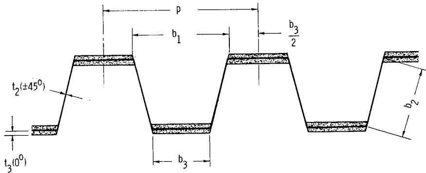
(b) Corrugated panel.
