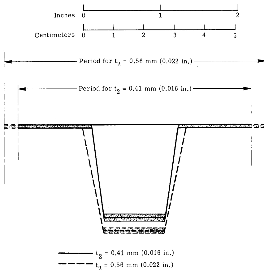
Figure 8.- Cross sections for two hat-stiffened panels designed for \frac{N_x}{L} = 689 \text{ kPa (100 lbf/in}^2\text{)} ; L = 0.76 \text{ m} (30 in.).
