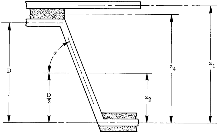
Figure 23.- Additional dimensions for hat-stiffened panel.
