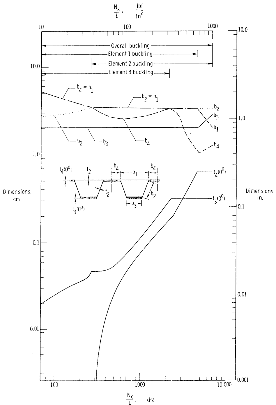
Figure 9.- Variation of cross-sectional dimensions as function of loading for minimum-mass, hat-stiffened, graphite-epoxy compression panels; t_2 = 0.56 mm (0.022 in.); L = 0.76 m (30 in.).
