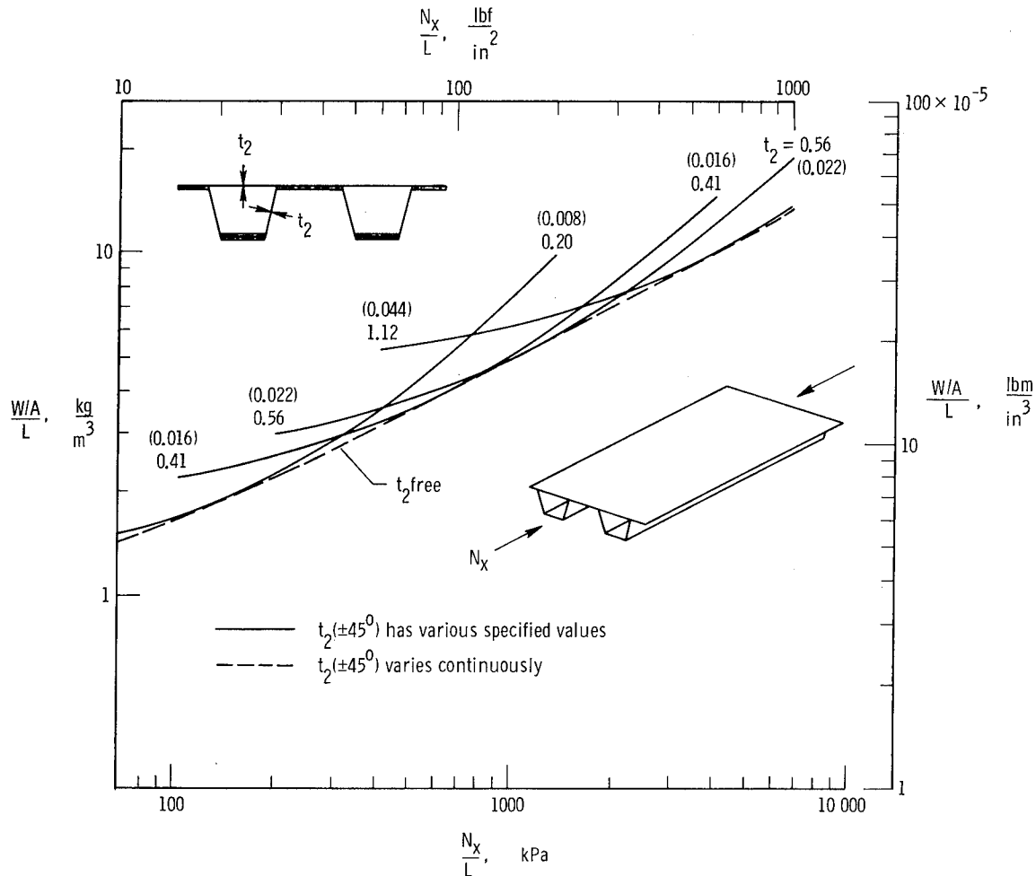
Figure 7.- Structural efficiency of graphite-epoxy, hat-stiffened compression panels for various prescribed values of thickness t_2 and for t_2 varying continuously; L = 0.76 m (30 in.); thickness t_2 is shown in mm (in.).
