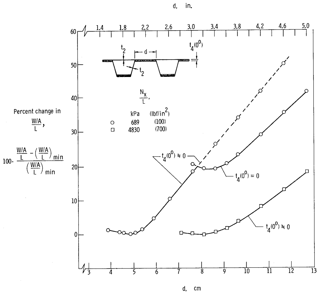
Figure 12.- Effect on structural efficiency of increasing stiffener spacing d of hat-stiffened, graphite-epoxy compression panels; t_2 varies continuously; L = 0.76 m (30 in.).
