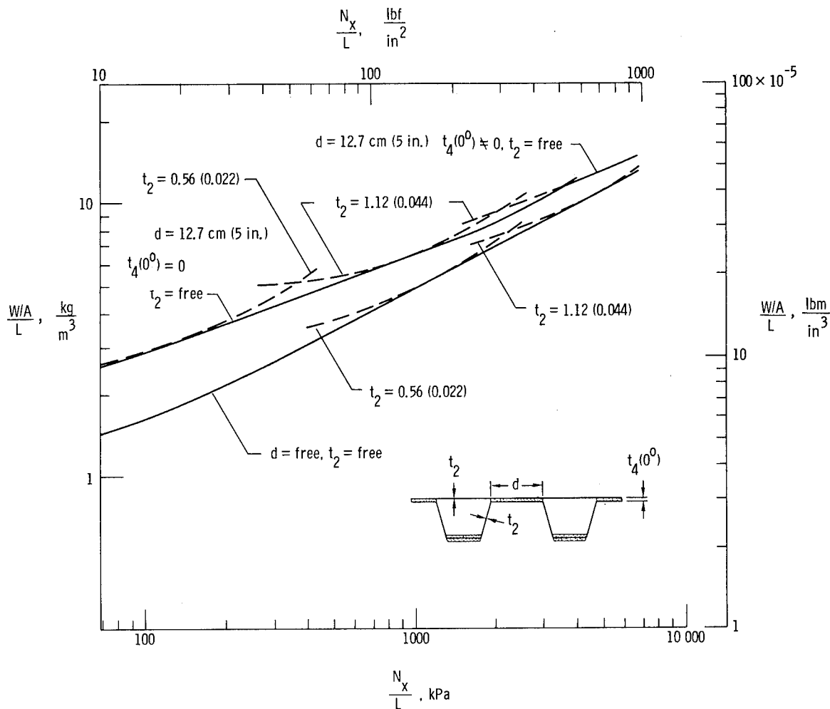
Figure 13.- Effect of d = 12.7 \text{ cm} (5 in.) stiffener spacing requirement on structural efficiency of hat-stiffened, graphite-epoxy compression panels. Thicknesses are shown in mm (in.); L = 0.76 \text{ m} (30 in.).
