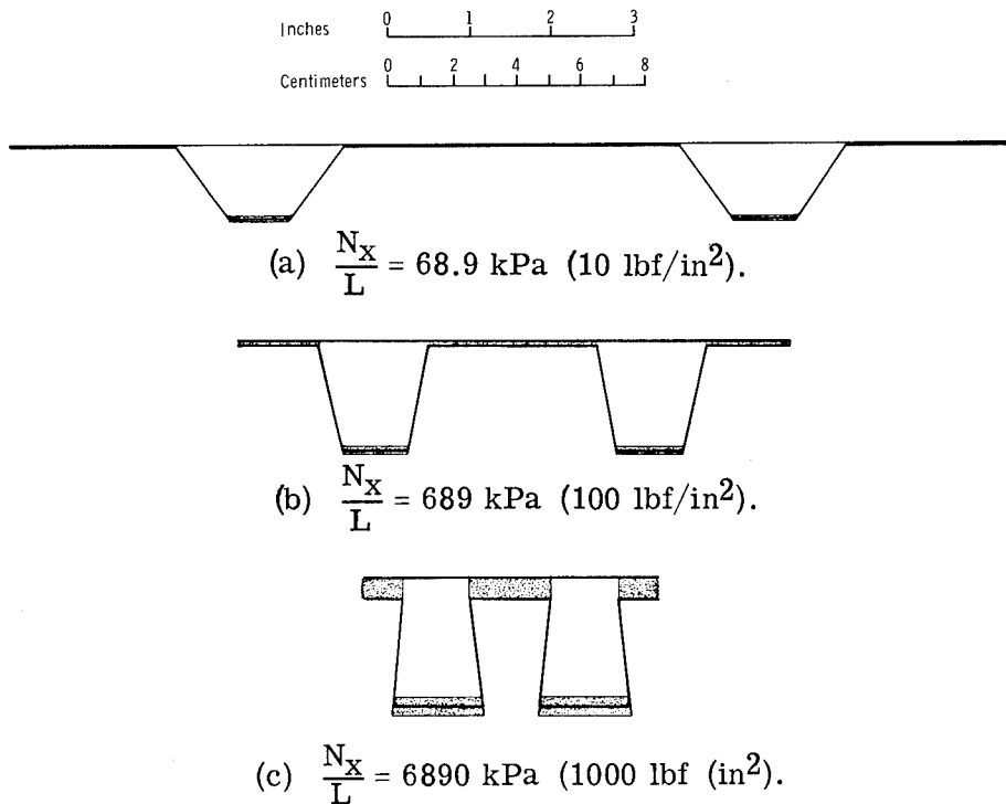
Figure 10.- Cross-sectional shapes of hat-stiffened, graphite-epoxy compression panels having t_2 = 0.56 mm (0.022 in.) and L = 0.76 m (30 in.) for three values of axial compressive load.
