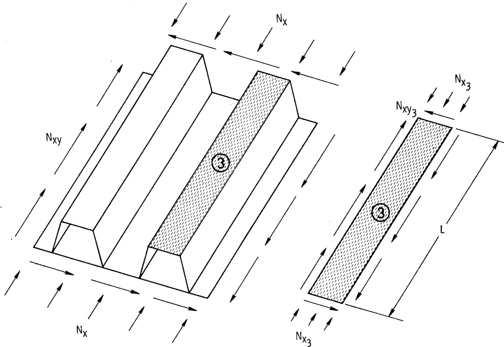
Figure 6.- Example of strip element used for local buckling.
