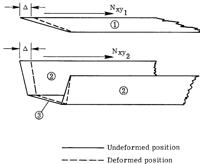
Figure 3.- Equating shear displacement of element 1 with sum of shear displacements of elements 2 and 3 to obtain internal shear-stress distribution.
