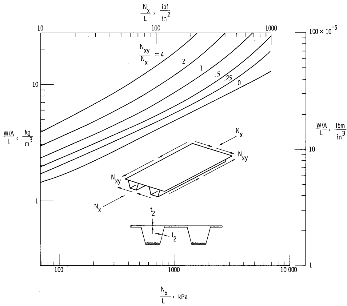
Figure 18.- Structural efficiency of graphite-epoxy, hat-stiffened panels subjected to combinations of longitudinal compression and shear loadings; L = 0.76 \text{ m (30 in.)} ; t_2 varies continuously.
