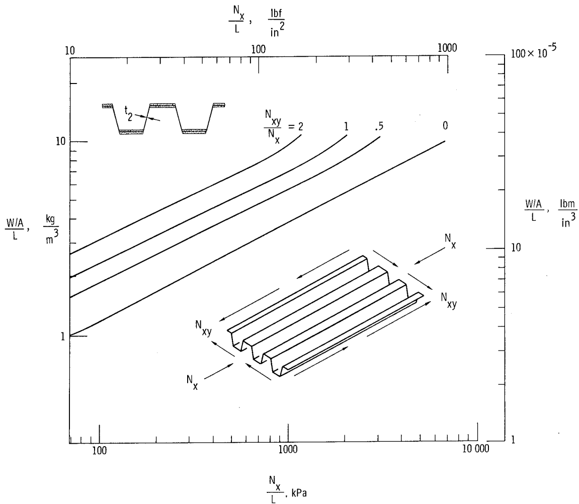
Figure 21.- Structural efficiency of graphite-epoxy corrugated panels subjected to combinations of longitudinal compression and shear loadings; L = 0.76 \text{ m} (30 in.); t_2 varies continuously.
