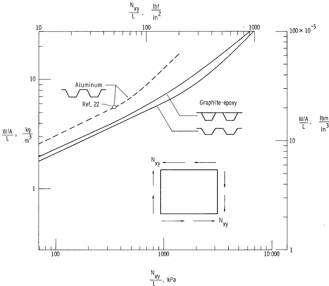
Figure 22. - Effect of shear loading on structural efficiency of graphite-epoxy and aluminum corrugated panels and graphite-epoxy hat-stiffened panels; L = 0.76 \text{ m} (30 in.); t_2 varies continuously.
