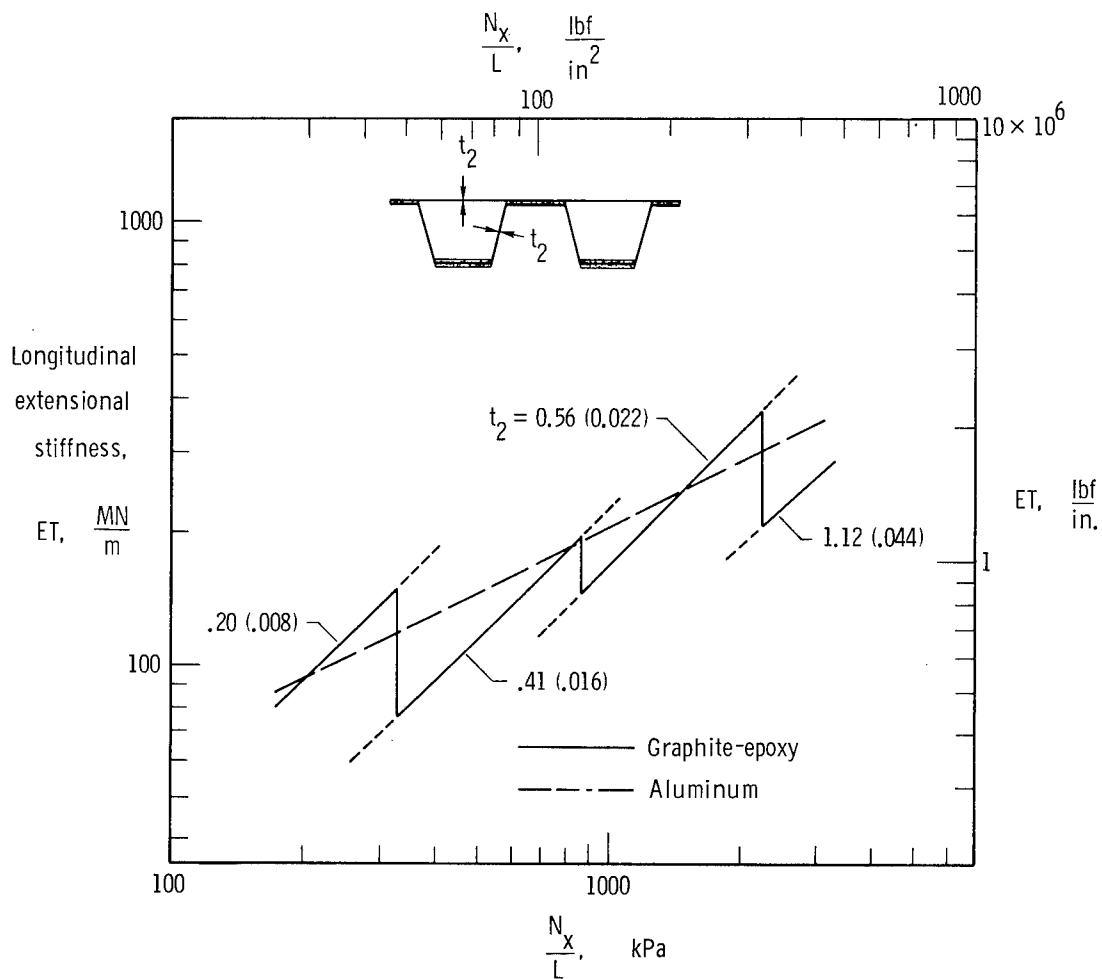
Figure 15.- Longitudinal extensional stiffness as function of loading for minimum-mass, graphite-epoxy and aluminum hat-stiffened compression panels; L = 0.76 \text{ m} (30 in.). Thicknesses are shown in mm (in.).
