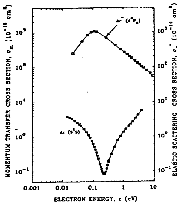
Fig. 3 Comparison of the momentum transfer cross section for scattering from the ground state argon atom \text{Ar}(3^1S) with the elastic electron scattering cross section from the excited argon atom \text{Ar}^*(4^3P_2) (see the text)
