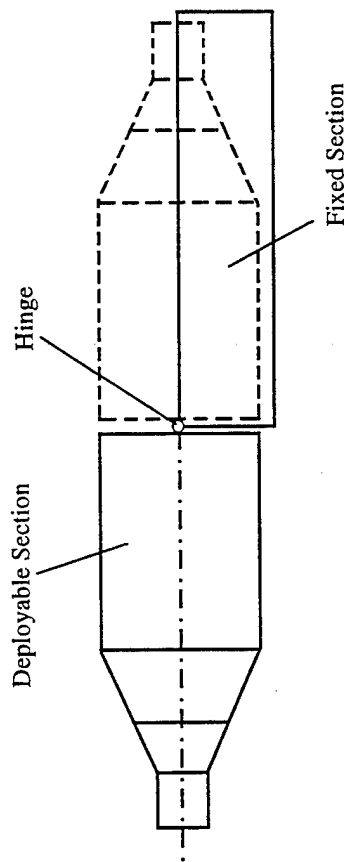
Fig. 4.13 Folding space radiator.
