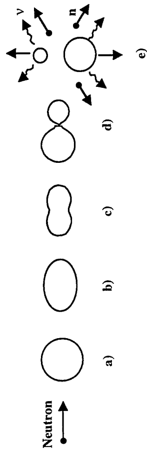
Fig. 2.8 Oscillating liquid droplet model of nuclear fission. a) spherical shape; b) ellipsoid; c) dumbbell; d) division; e) fission.
