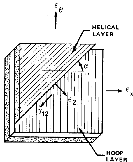
Figure 7. Laminate and lamina strains.
