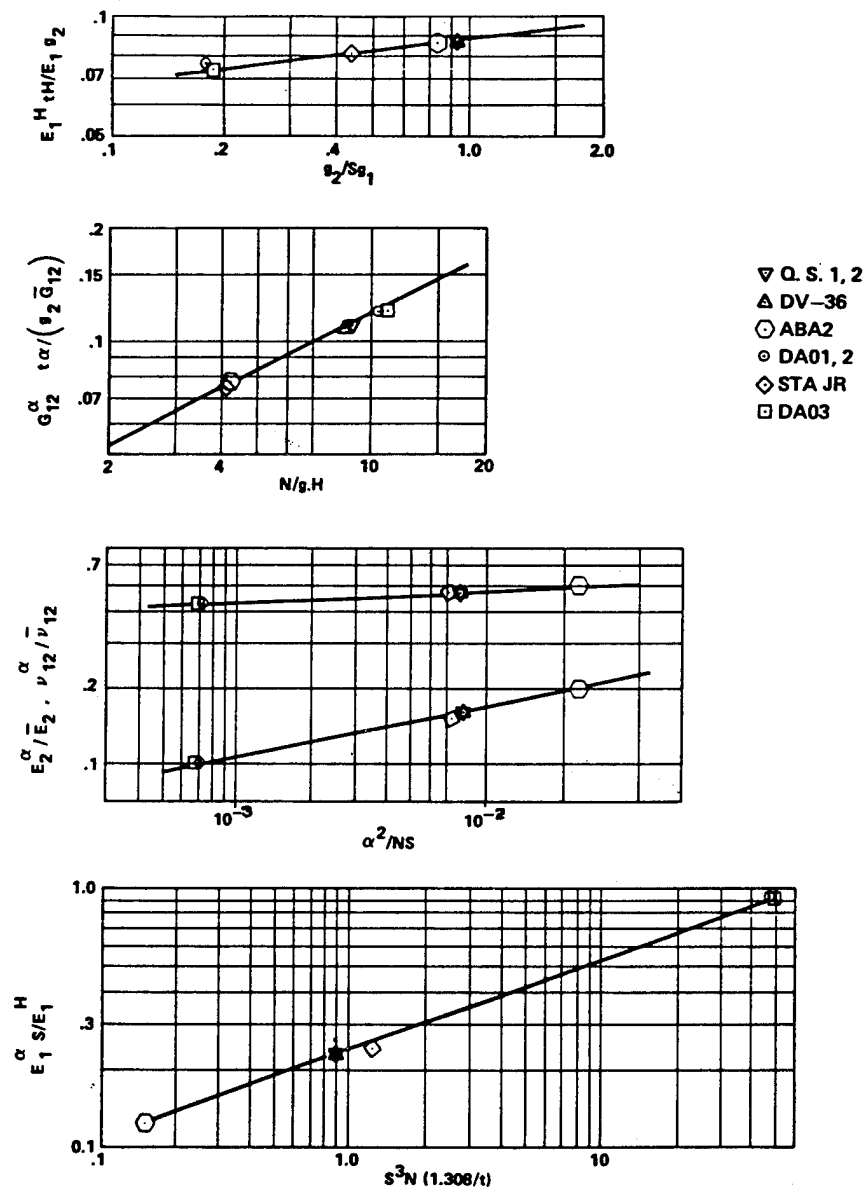
Figure 8. Scaling dependency of lamina elastic constants.
