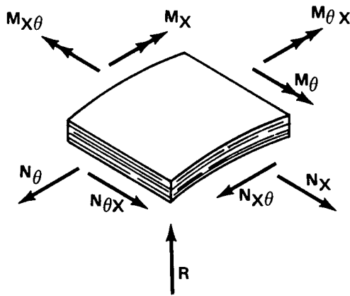
Figure 2. Membrane element.
