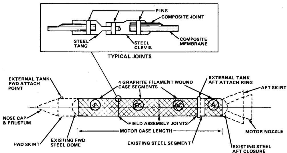
Figure 1. Solid rocket motor.
