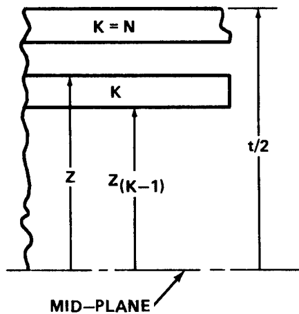
Figure 4. N-ply laminate about mid-plane.
