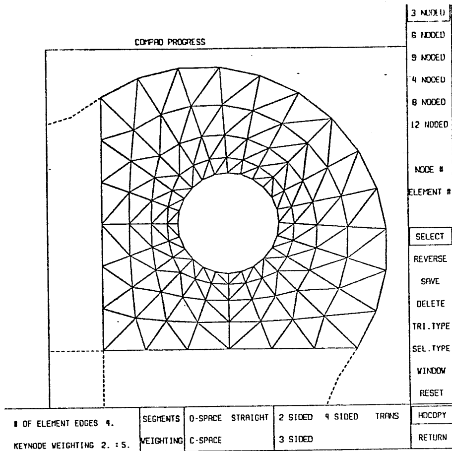
Figure 28 Two-Sided Mesh of Three-Noded Elements
