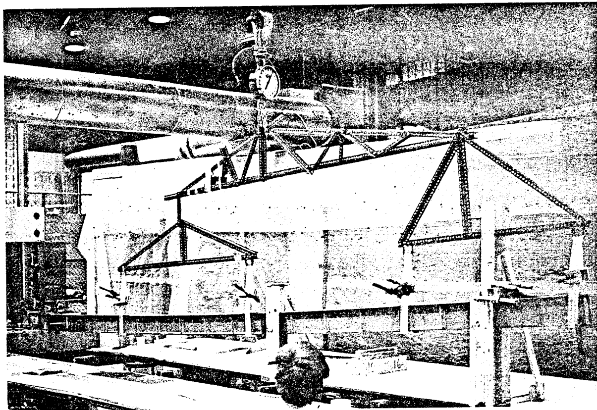
Figure 14 Spar Test
