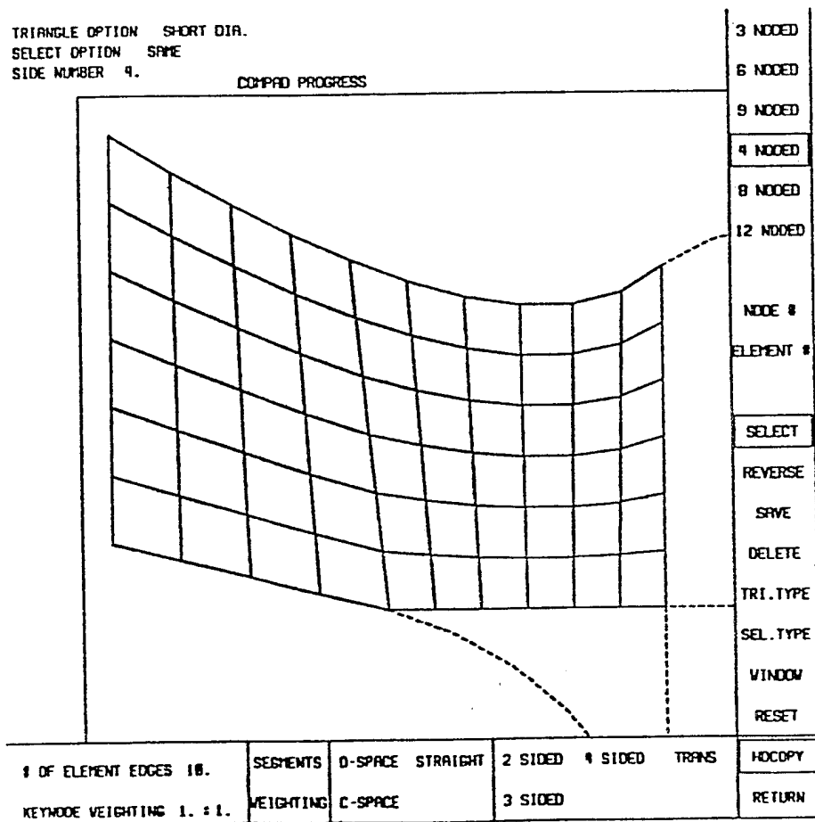
Figure 25 Four-Sided Mesh of Four-Noded Elements
