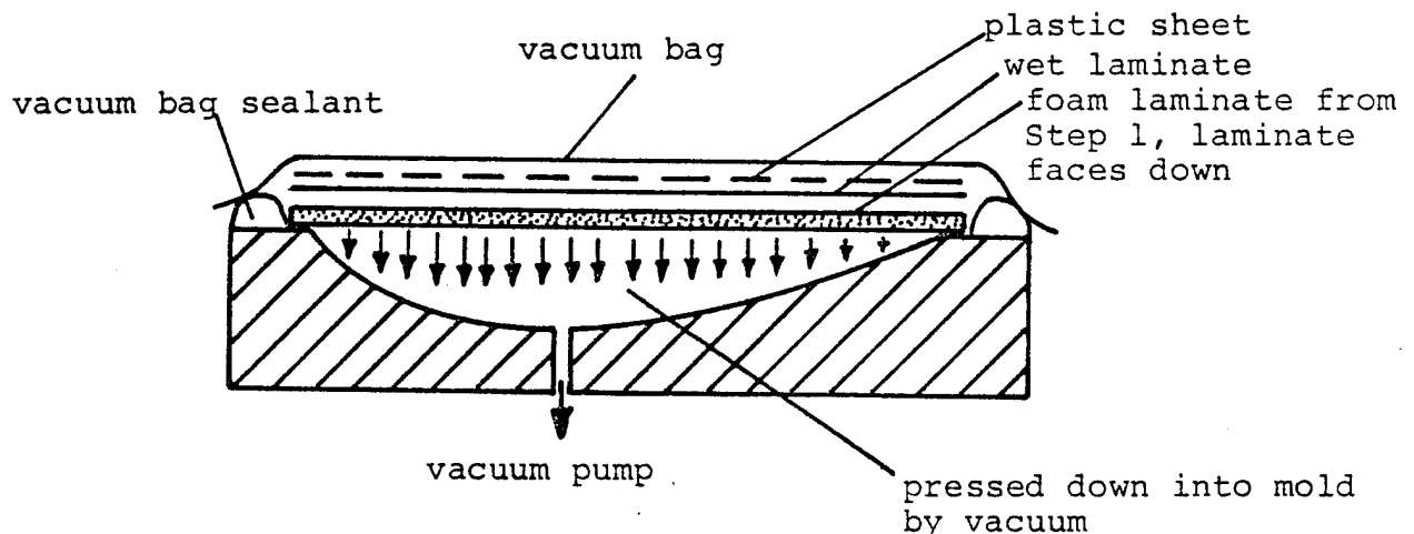
Wet-Lay-Up Mold Technique
