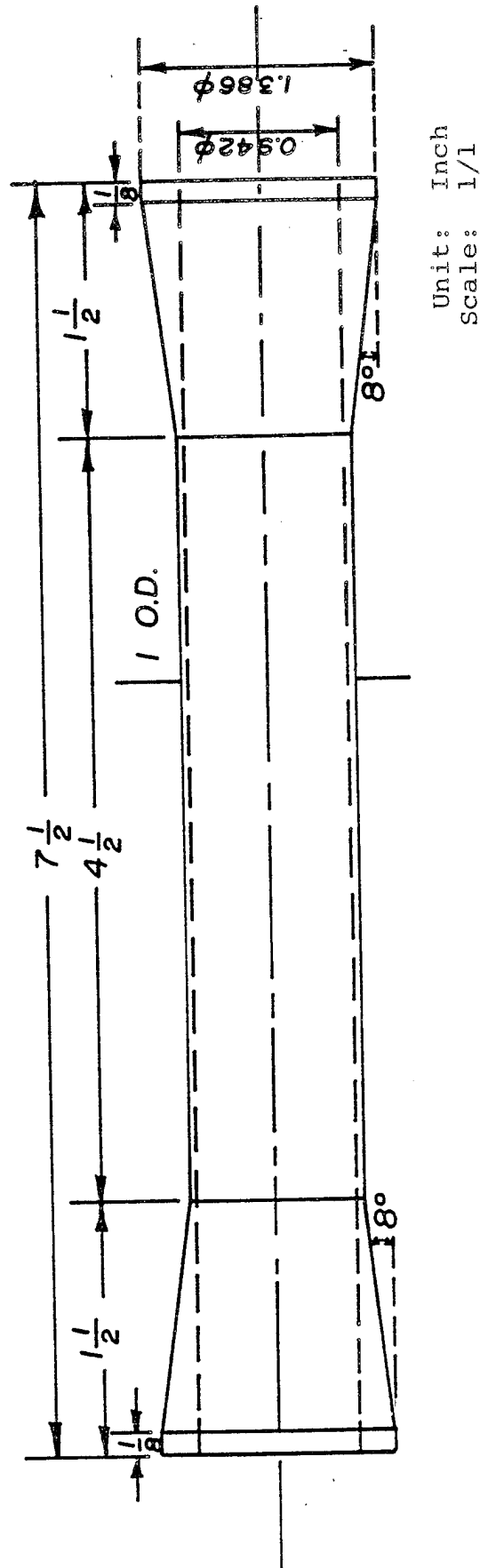
Graphite/Epoxy Thin-Walled Tube Specimen for Bi-Axial Fatigue Testing Wrap-Around Technique of 4 Layers \pm 45^\circ Graphite/Epoxy
