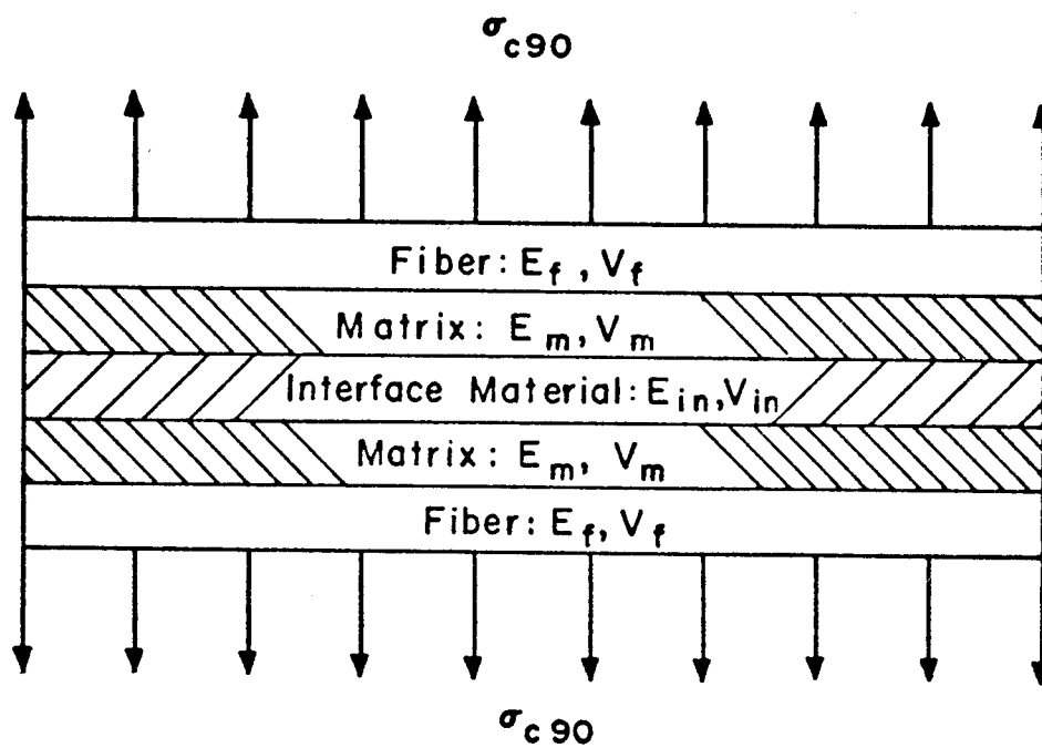
Fig. 5 Schematic of composite volume element containing fiber, matrix and interface material with loading perpendicular to fiber direction.
