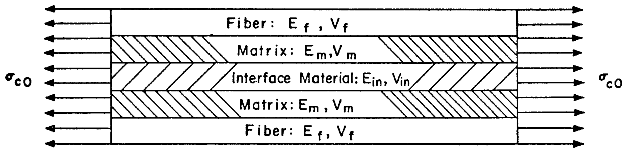
Fig. 4 Schematic of composite volume element containing fiber, matrix and interface material with loading in fiber direction.
