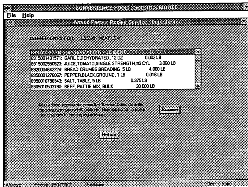
Figure 4 - Ingredients Screen
