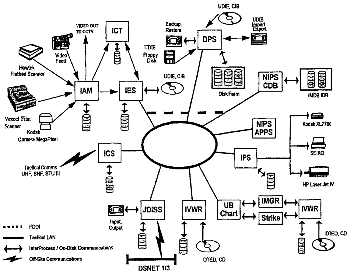
Figure 8.1: JMCIS Imagery Architecture [Ref. 26]
