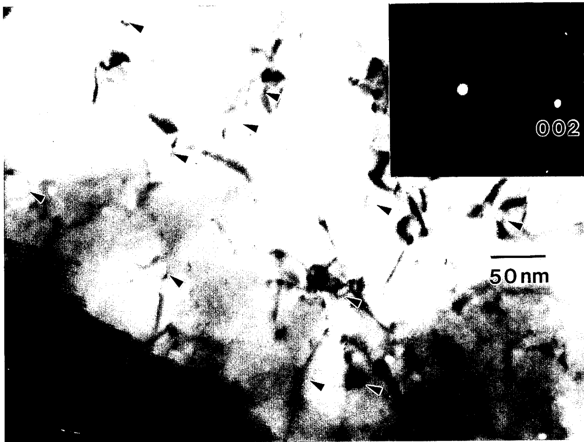
Figure 10c. TEM micrograph of Nb-1wt%Zr-0.1wt%C crept to 0.2 strain at 93 MPa and 1300 K showing detail of cell interior. Relatively few dislocations are present. Carbide particles shown at markers. Magnification 165 kX.
