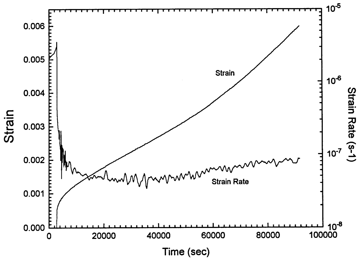
Figure 8. Example of monotonic creep test at 1400 K, 63 MPa illustrating increased strain rate due to particle growth.
