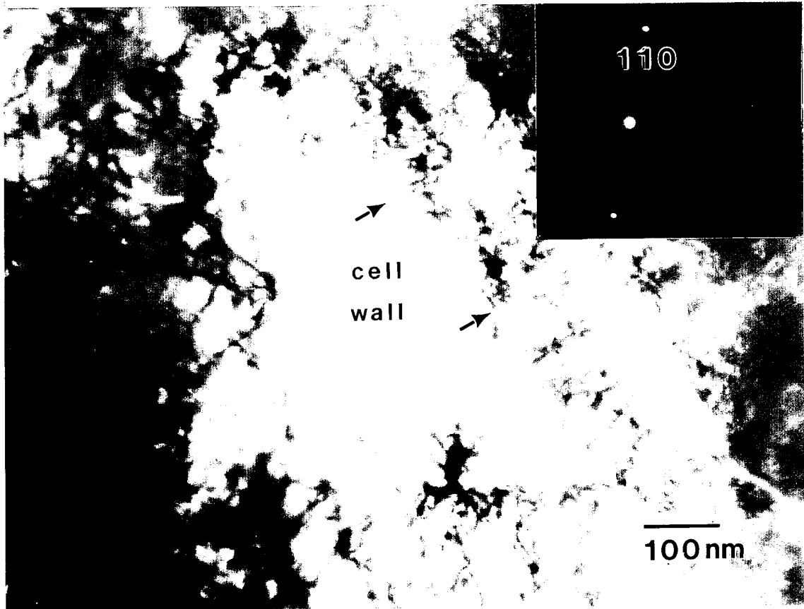
Figure 10b. TEM micrograph of Nb-1wt%Zr-0.1wt%C crept to 0.2 strain at 93 MPa and 1300 K showing detail of cell wall. Magnification 100 kX.
