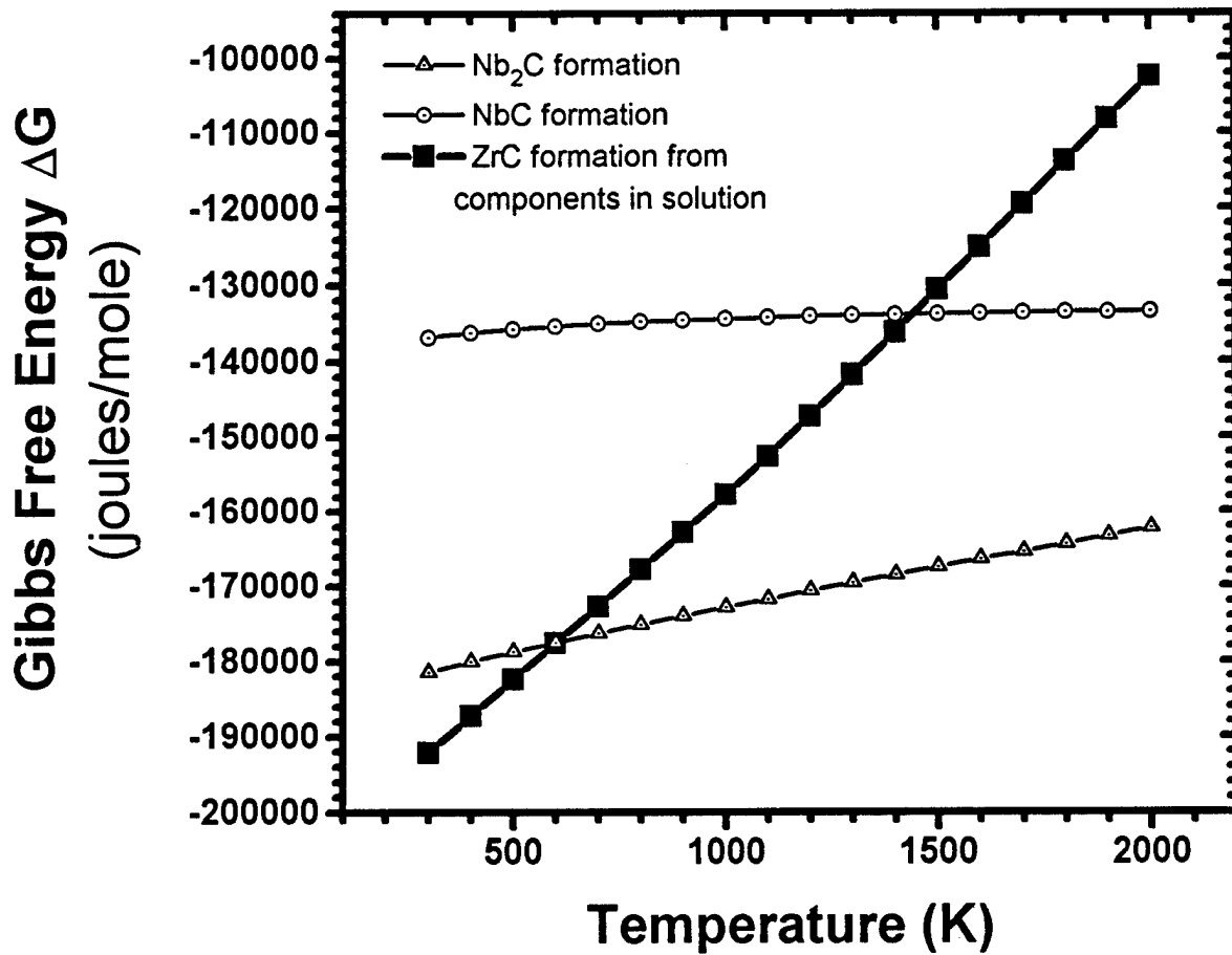
Figure 14. Free energy of formation for NbC, Nb 2 C and ZrC when activity of Zr is low as during initial solution treatment.
