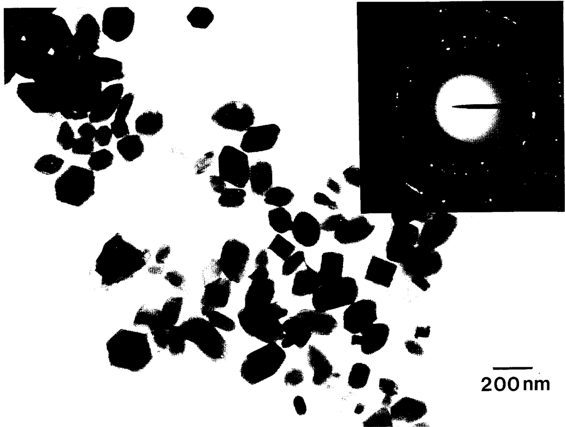
Figure 5. TEM micrograph of extracted (Nb,Zr)C carbide particles from as-received alloy. Magnification of negative 27.5 kX. Size marker shown.
