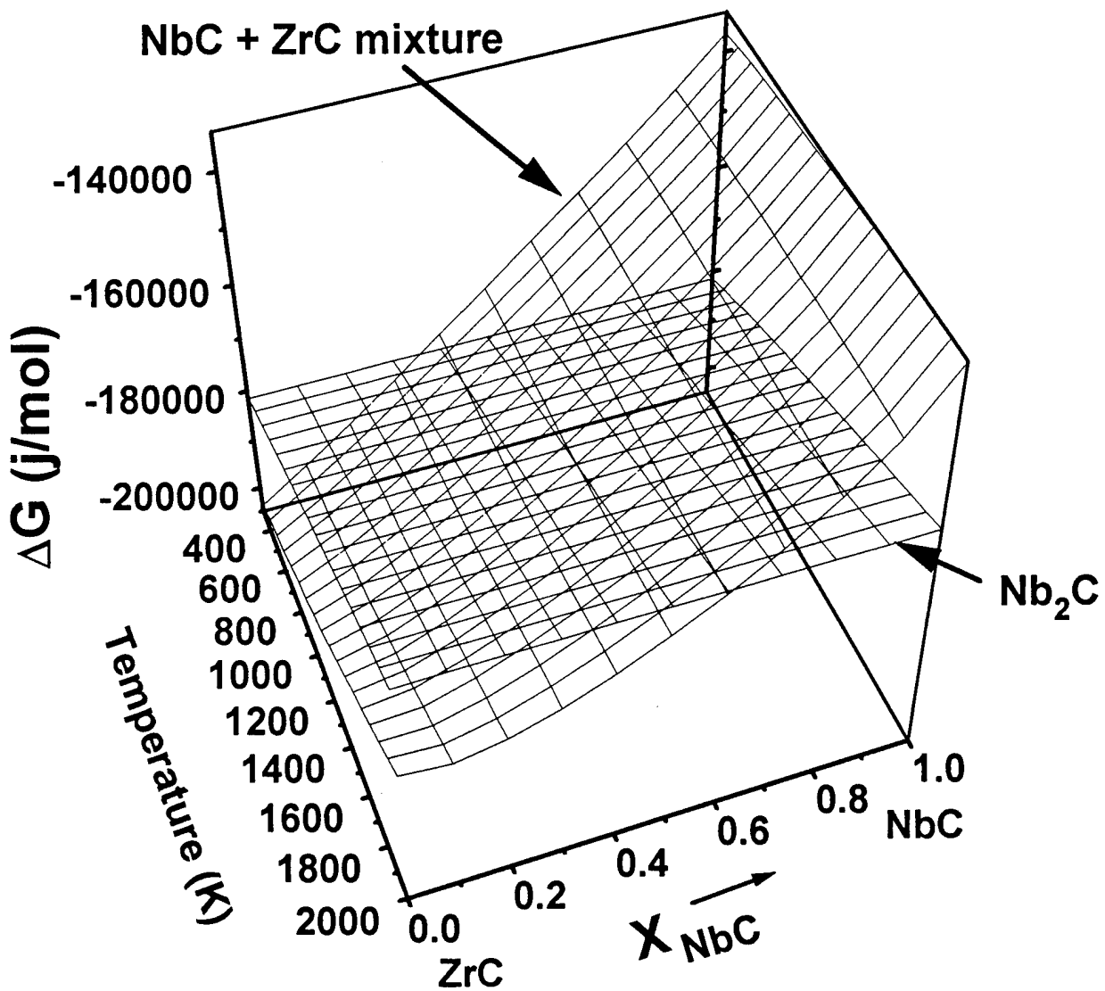
Figure 16. Free energy surfaces of Nb 2 C and (NbC + ZrC) mixture when Zr activity = 1. Intersection of two surfaces specifies equilibrium ZrC (and NbC) concentration of mixture.
