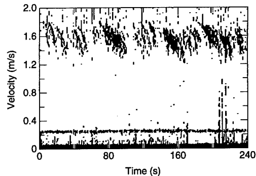
Figure 13. The part of the radar velocity record for breakup with dispersed ice floes in the river. Note the movement in time of strong returns from higher to lower velocity, corresponding to the movement of floes through the antenna footprint.
