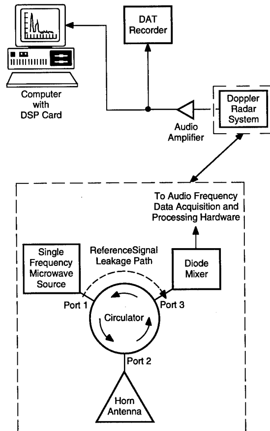
Figure 3. Fundamental components of the Doppler radar system with an expanded view of the front-end.
